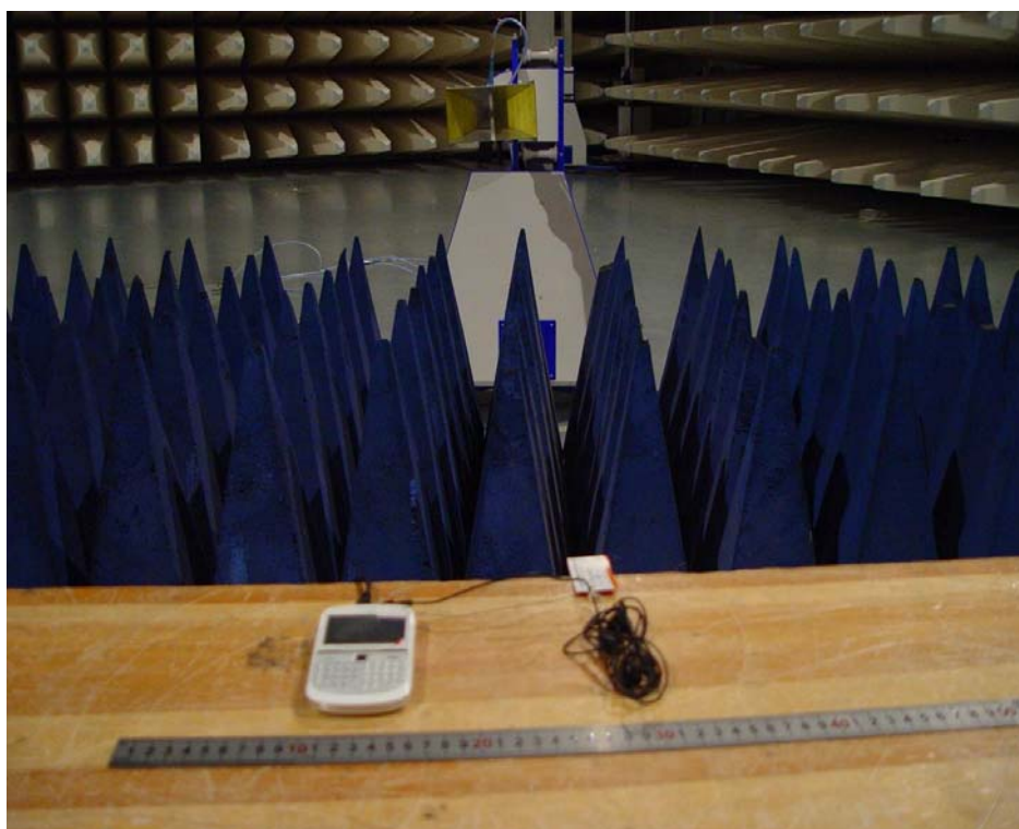
Spurious Radiated Emissions Test setup
