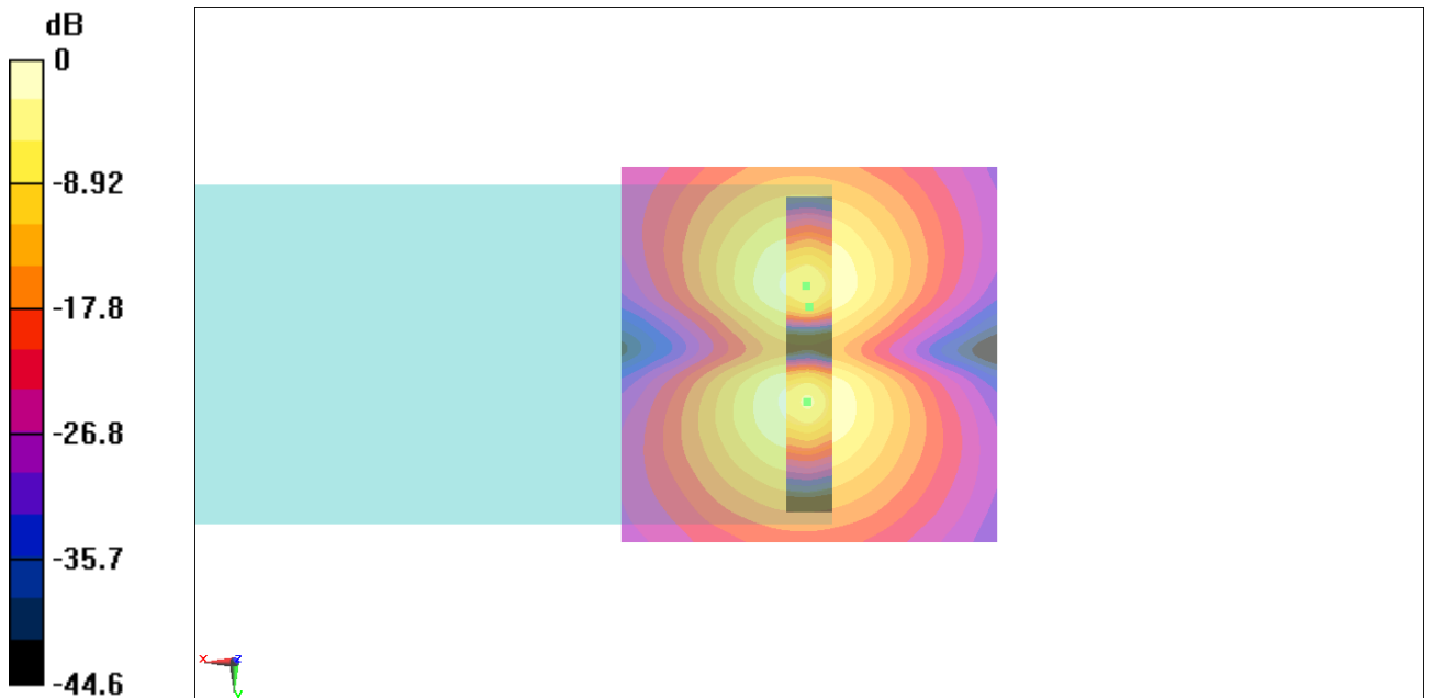
Fig B.5 T-Coil GSM 1900
