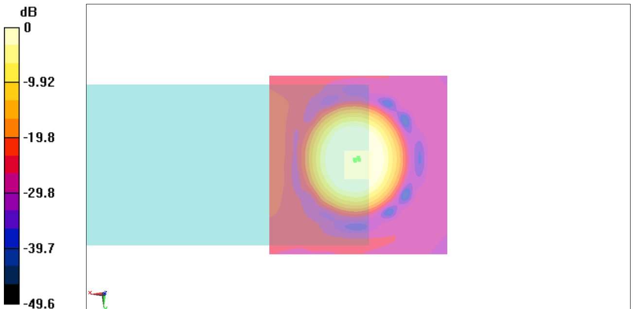
Fig B.6 T-Coil GSM 1900
