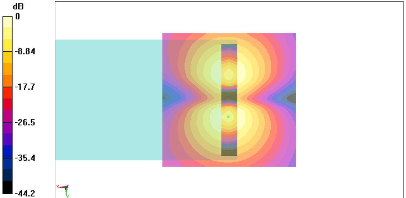
Fig B.2 T-Coil GSM 850
