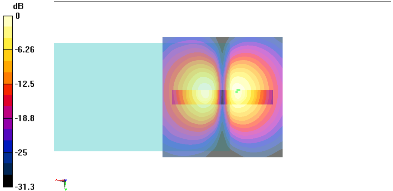
Fig B.1 T-Coil GSM 850
