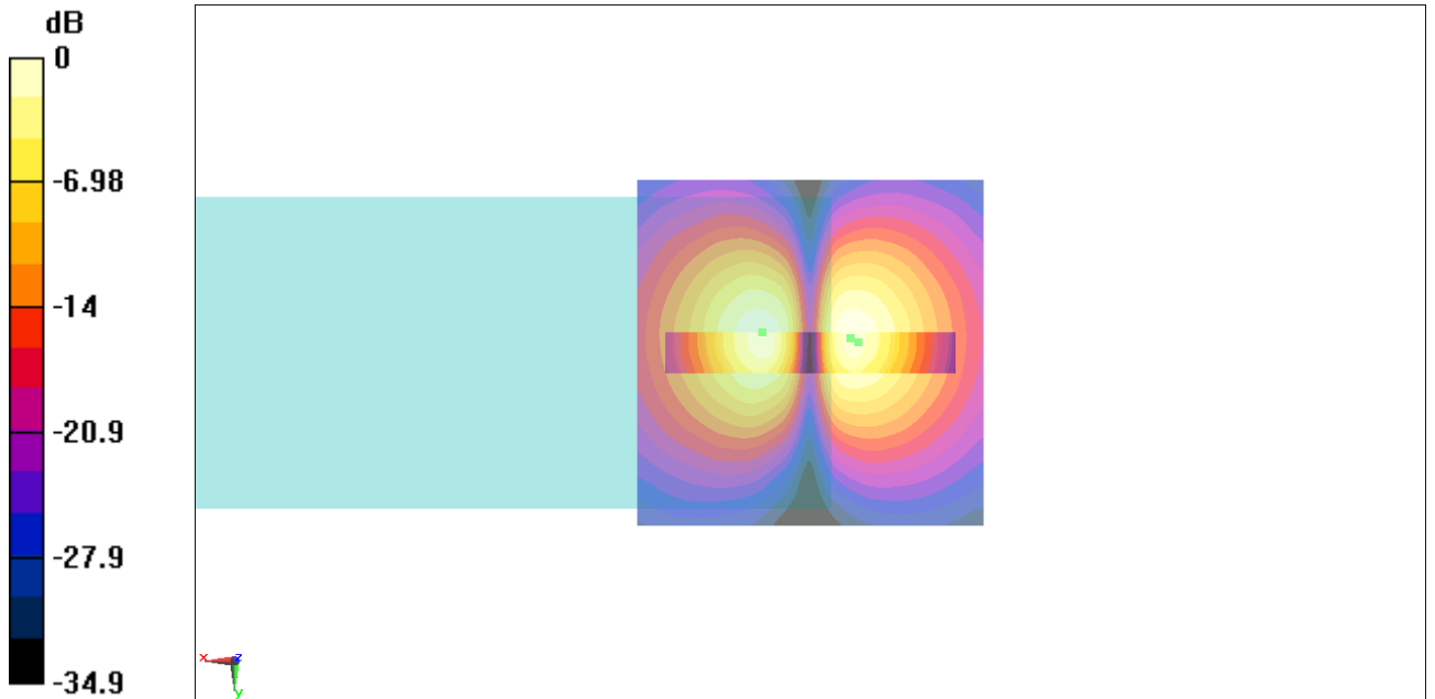
Fig B.4 T-Coil GSM 1900
