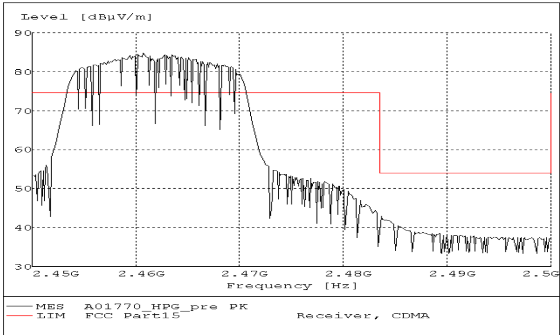
Fig. 115 Radiated Spurious Emission (Power): 802.11g, ch11, 2.45 GHz - 2.50GHz
