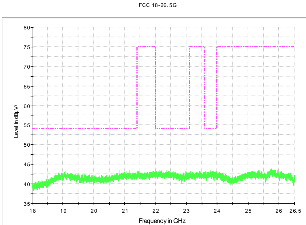
Fig. 130 Radiated emission: 18 GHz - 26.5 GHz
