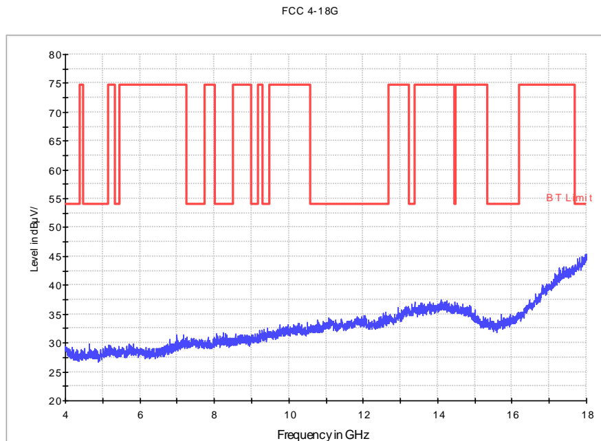
Fig. 122 Radiated Spurious Emission (802.11n-20MHz, Ch1, 4 GHz-18 GHz)
