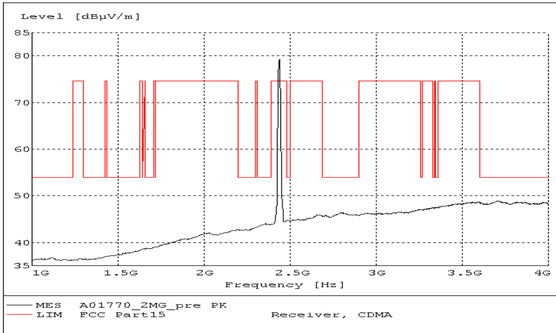
Fig. 113 Radiated Spurious Emission (802.11g, Ch6, 1 GHz-4 GHz)
