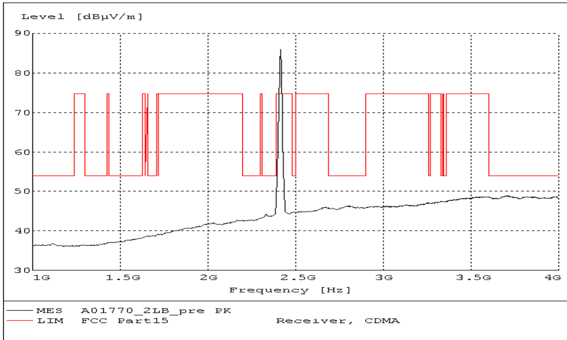
Fig. 121 Radiated Spurious Emission (802.11n-20MHz, Ch1, 1 GHz-4 GHz)
