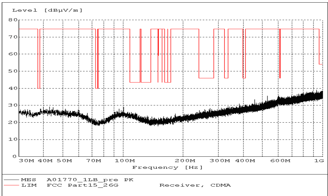
Fig. 120 Radiated Spurious Emission (802.11n-20MHz, Ch1, 30 MHz-1 GHz)
