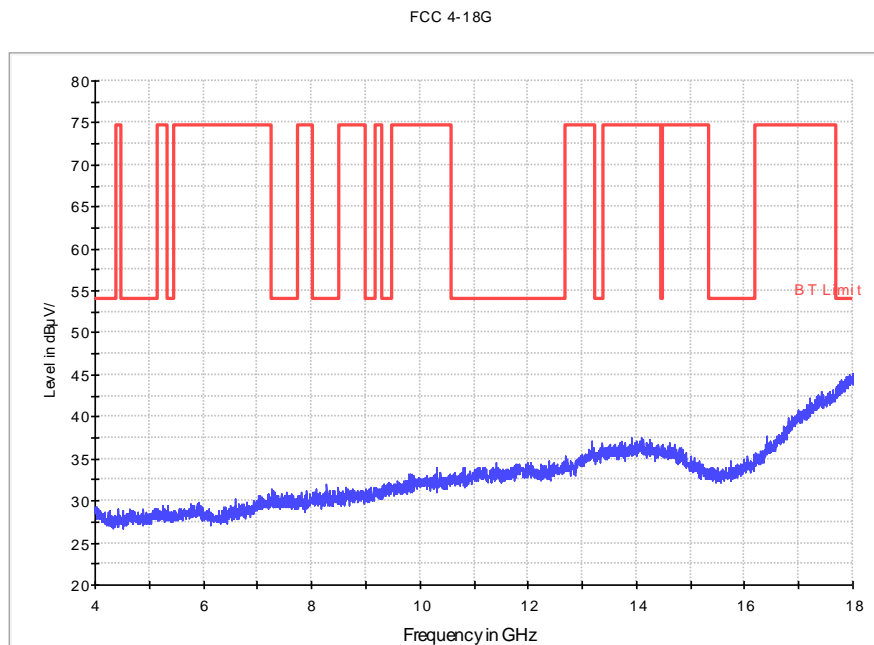
Fig. 114 Radiated Spurious Emission (802.11g, Ch6, 4 GHz-18 GHz)
