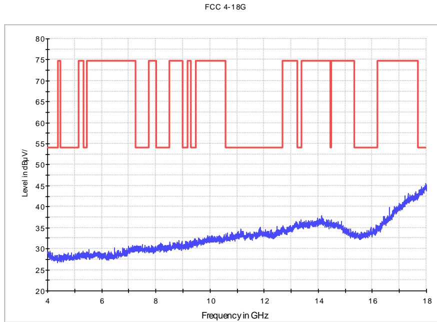
Fig. 129 Radiated Spurious Emission (802.11n-20MHz, Ch11, 4 GHz-18 GHz)
