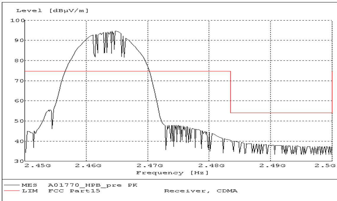
Fig. 104 Radiated Spurious Emission (Power): 802.11b, ch11, 2.45 GHz - 2.50GHz
