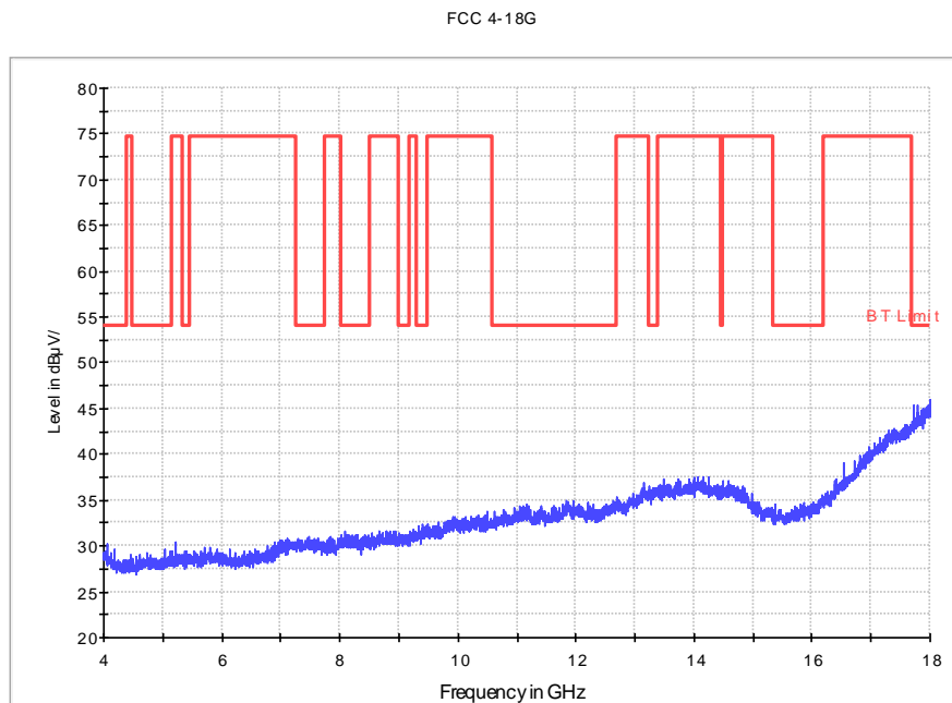
Fig. 118 Radiated Spurious Emission (802.11g, Ch11, 4 GHz-18 GHz)
