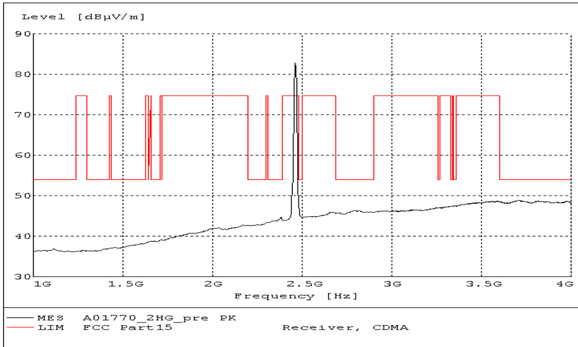
Fig. 117 Radiated Spurious Emission (802.11g, Ch11, 1 GHz-4 GHz)
