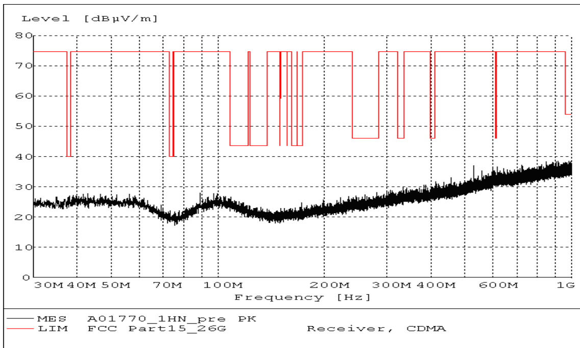
Fig. 127 Radiated Spurious Emission (802.11n-20MHz, Ch11, 30 MHz-1 GHz)
