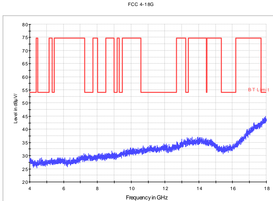
Fig. 125 Radiated Spurious Emission (802.11n-20MHz, Ch6, 4 GHz-18 GHz)
