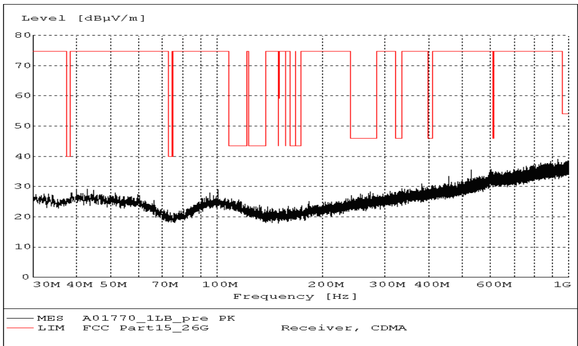
Fig. 98 Radiated Spurious Emission (802.11b, Ch1, 30 MHz-1 GHz)
