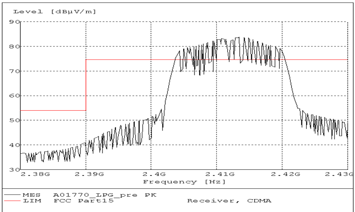
Fig. 108 Radiated Spurious Emission (Power): 802.11g, ch1, 2.38 GHz - 2.43GHz
