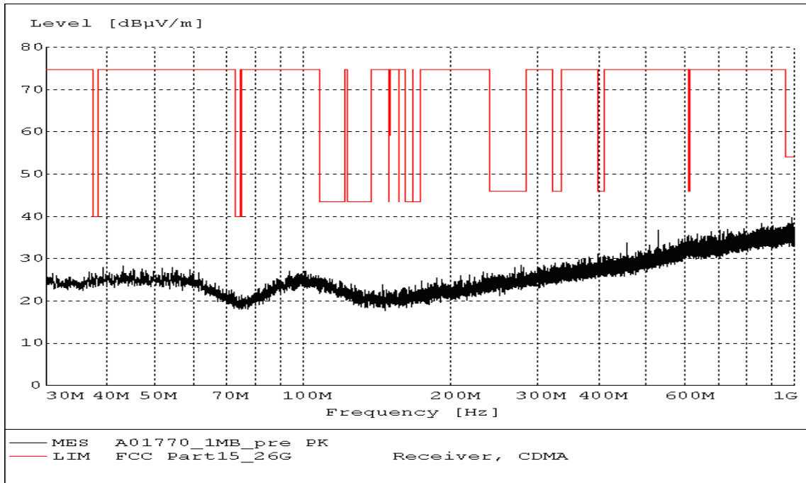
Fig. 101 Radiated Spurious Emission (802.11b, Ch6, 30 MHz-1 GHz)
