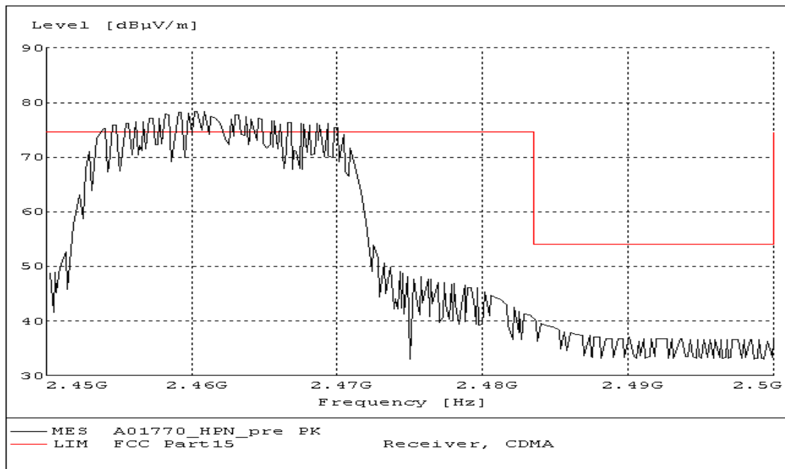
Fig. 126 Radiated Spurious Emission (Power): 802.11n-20MHz, ch11, 2.45 GHz - 2.50GHz
