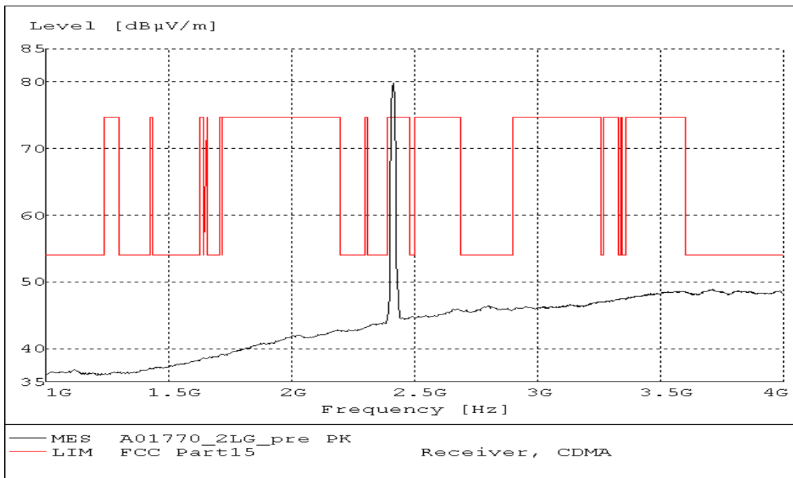
Fig. 110 Radiated Spurious Emission (802.11g, Ch1, 1 GHz-4 GHz)
