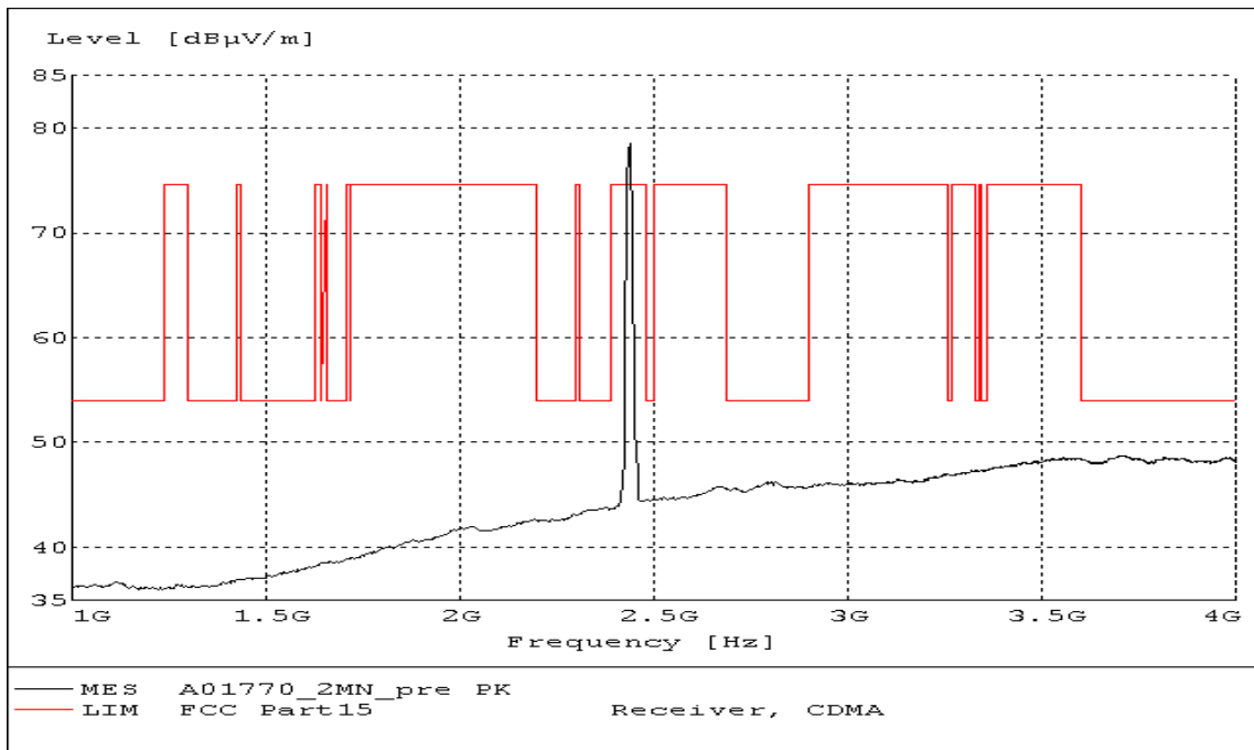
Fig. 124 Radiated Spurious Emission (802.11n-20MHz, Ch6, 1 GHz-4 GHz)
