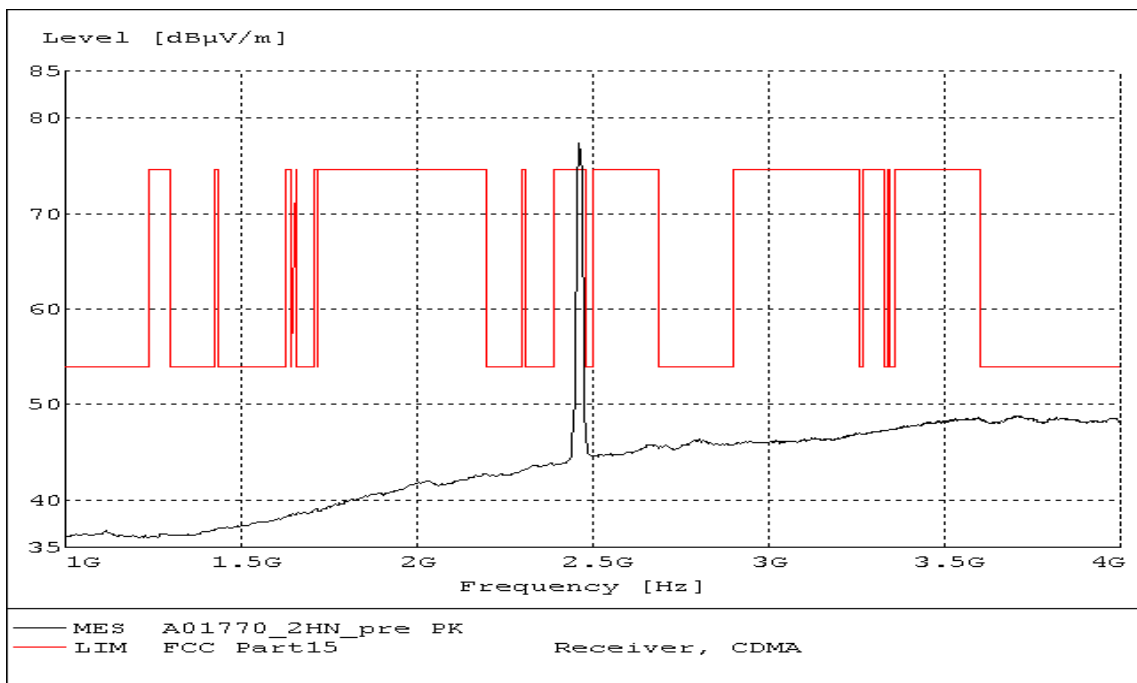
Fig. 128 Radiated Spurious Emission (802.11n-20MHz, Ch11, 1 GHz-4 GHz)
