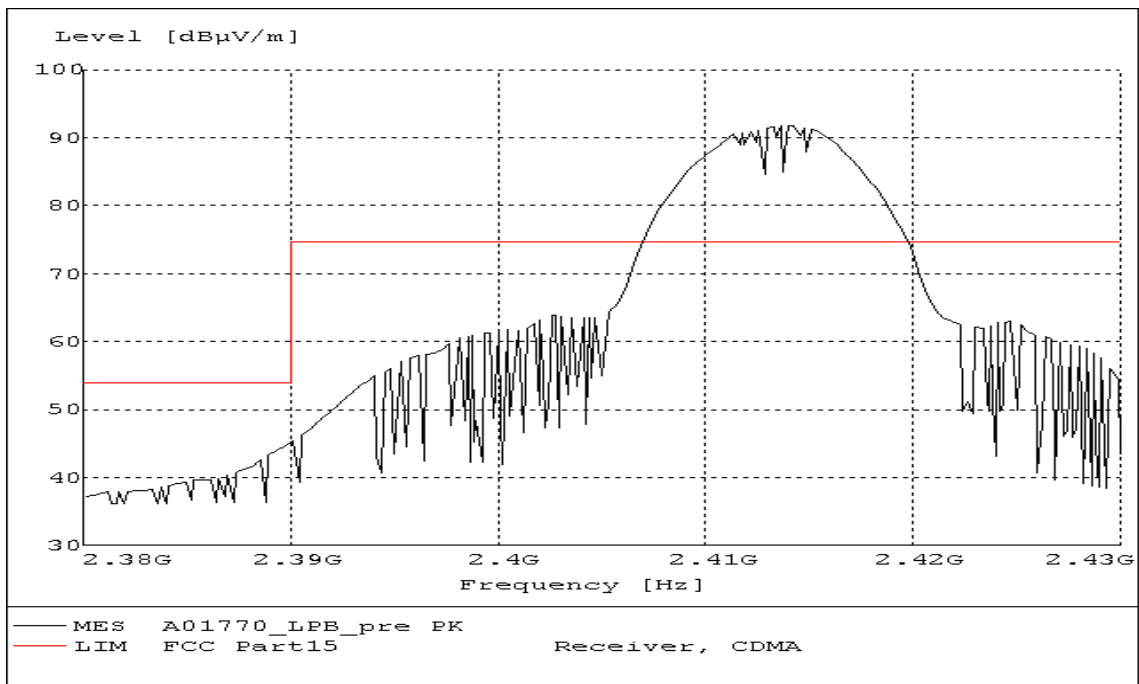
Fig. 97 Radiated Spurious Emission (Power): 802.11b, ch1, 2.38 GHz - 2.43GHz
