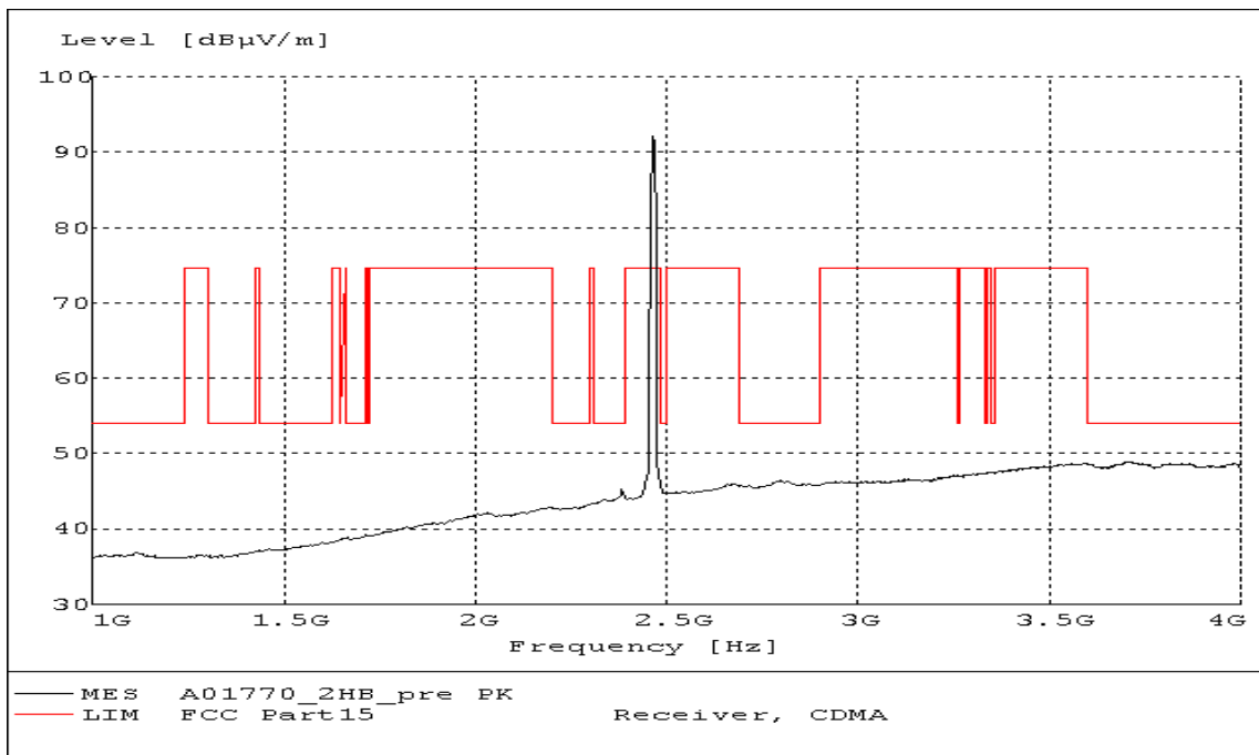
Fig. 106 Radiated Spurious Emission (802.11b, Ch11, 1 GHz-4 GHz)
