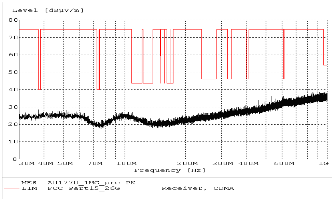
Fig. 112 Radiated Spurious Emission (802.11g, Ch6, 30 MHz-1 GHz)
