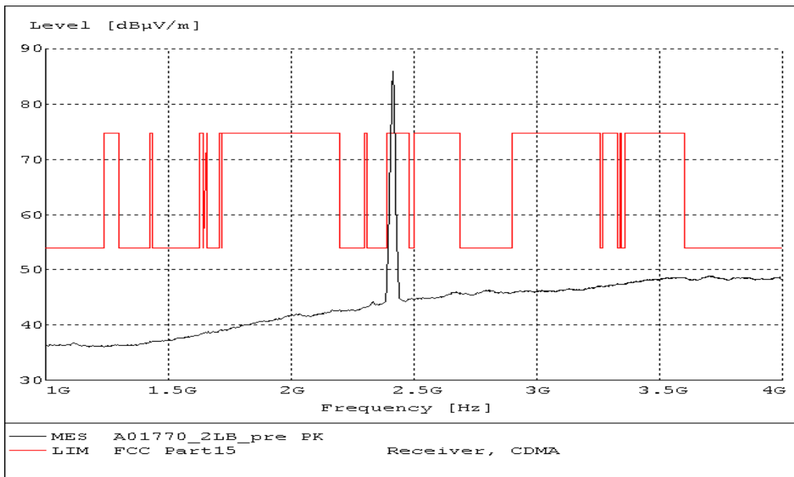
Fig. 99 Radiated Spurious Emission (802.11b, Ch1, 1 GHz-4 GHz)
