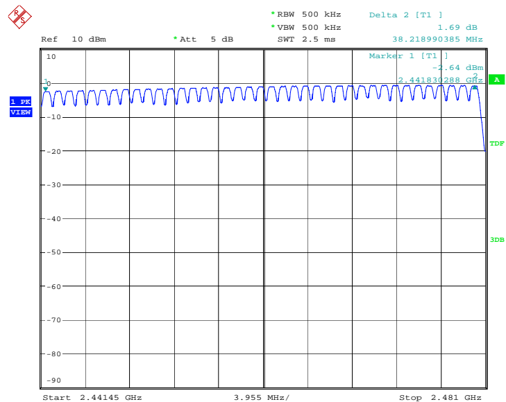
Fig.42. Number of hopping frequencies: GFSK, Channel 0 - 39
