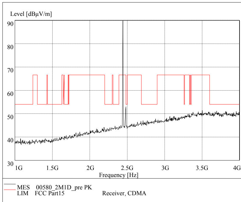
Fig.24. Radiated emission: GFSK, Channel 39, 1 GHz - 4 GHz
