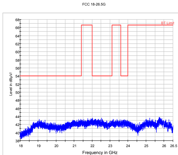
Fig.31. Radiated emission: GFSK, 18 GHz - 26 GHz
