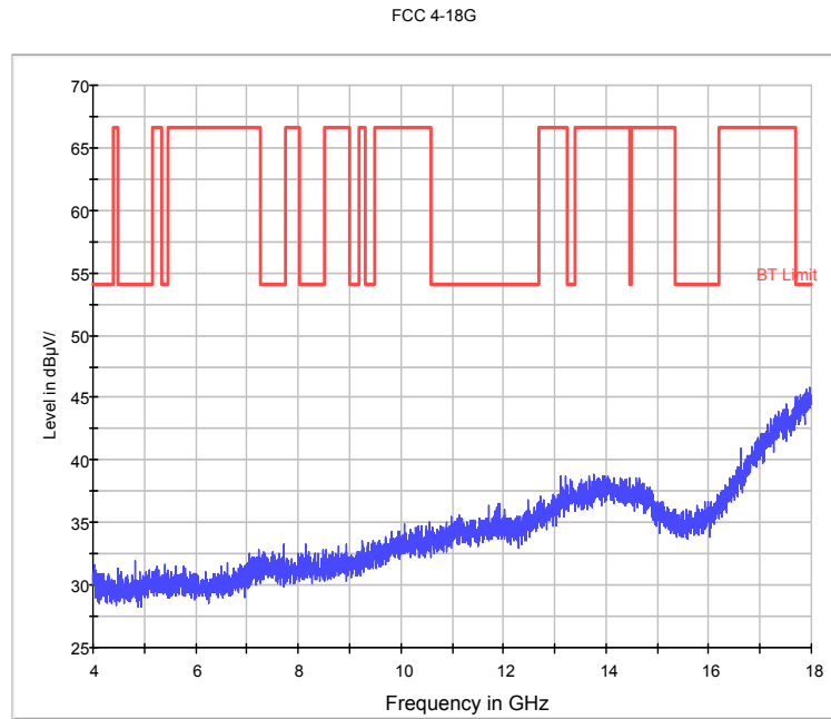
Fig.28. Radiated emission: GFSK, Channel 78, 4 GHz - 18 GHz
