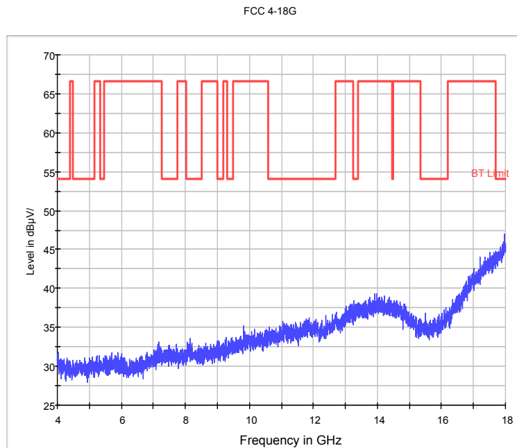
Fig.25. Radiated emission: GFSK, Channel 39, 4 GHz - 18 GHz
