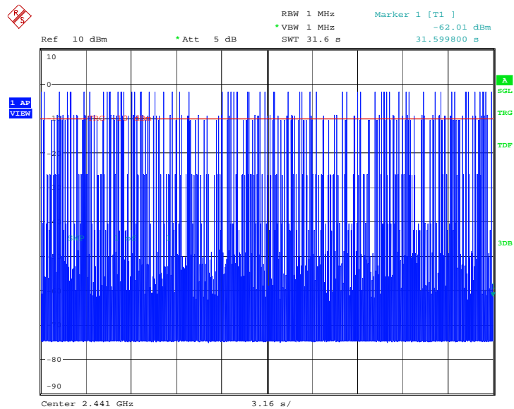
Fig.36. Time of occupancy (Dwell Time): Channel 39, Packet DH5
