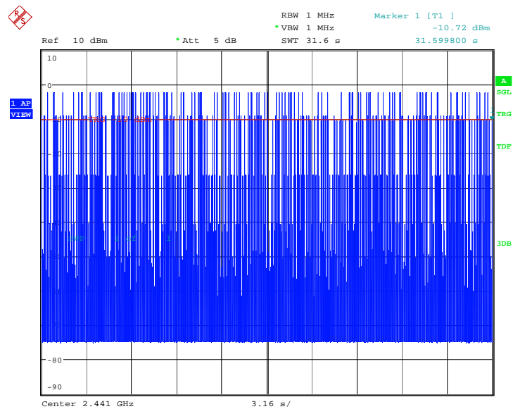
Fig.34. Time of occupancy (Dwell Time): Channel 39, Packet DH3
