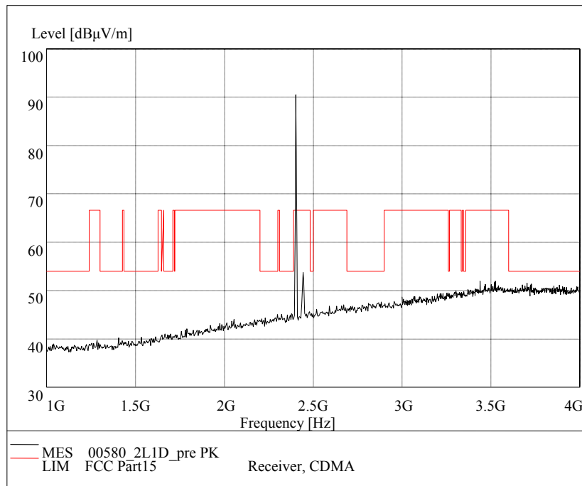
Fig.21. Radiated emission: GFSK, Channel 0, 1 GHz - 4 GHz
