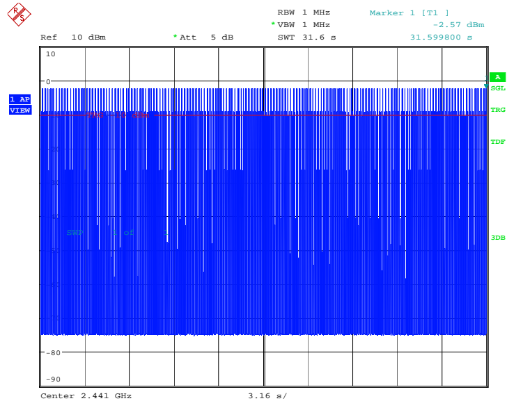
Fig.32. Time of occupancy (Dwell Time): Channel 39, Packet DH1
