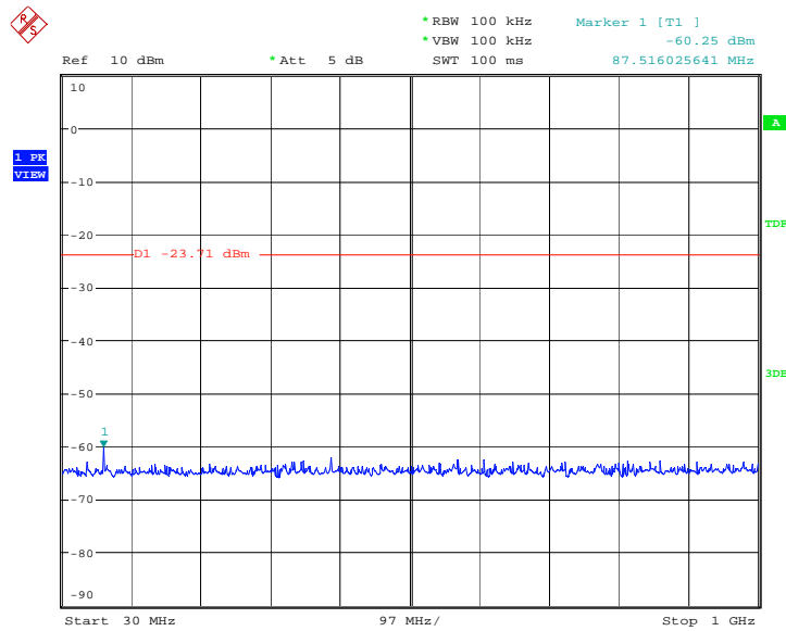
Fig.5. Conducted spurious emission: GFSK, Channel 0,2402MHz
