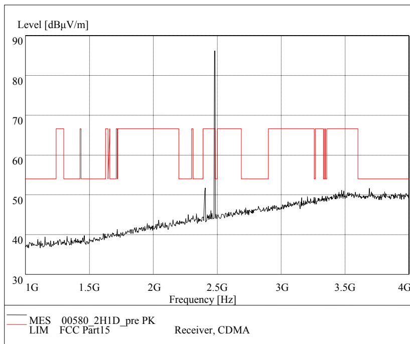
Fig.27. Radiated emission: GFSK, Channel 78, 1 GHz - 4 GHz
