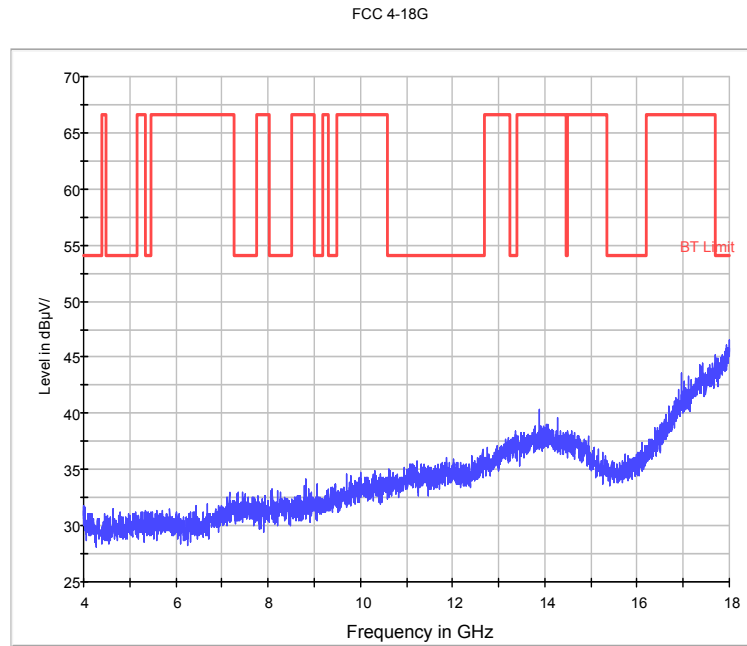
Fig.22. Radiated emission: GFSK, Channel 0, 4 GHz - 18 GHz
