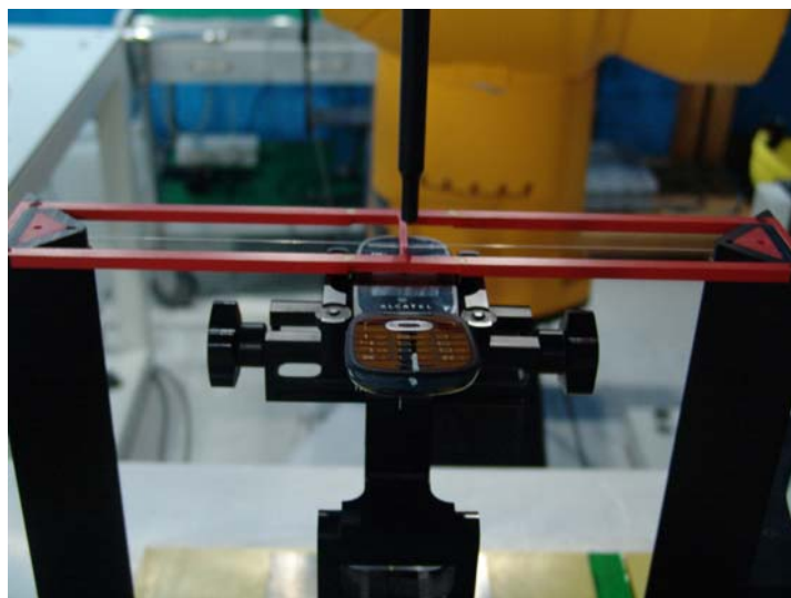
Picture 2: EUT Positioning for RF
