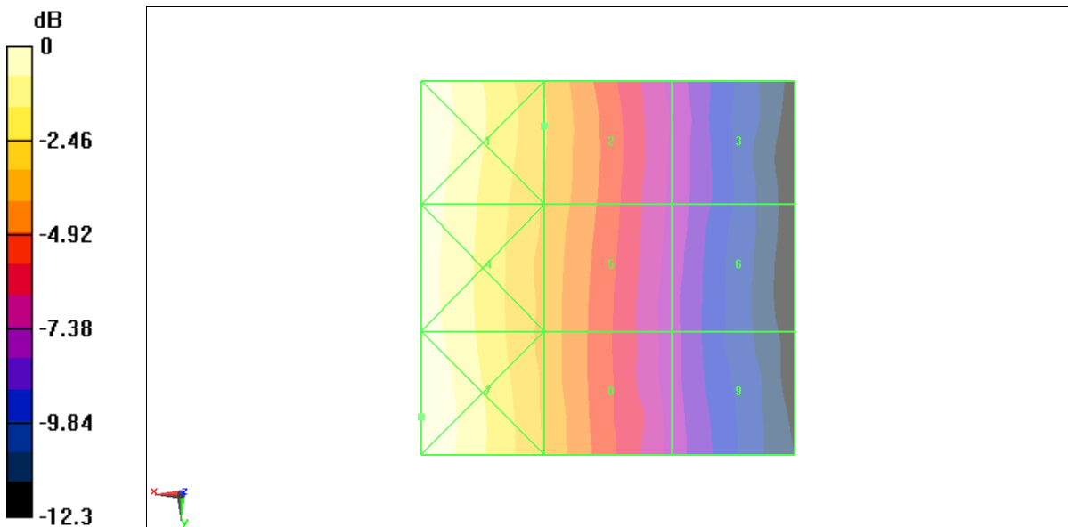
Fig B.14 HAC RF H-Field GSM 850 Middle
