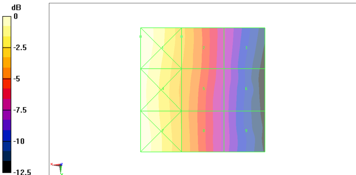
Fig B.19 HAC RF H-Field WCDMA 850 High
