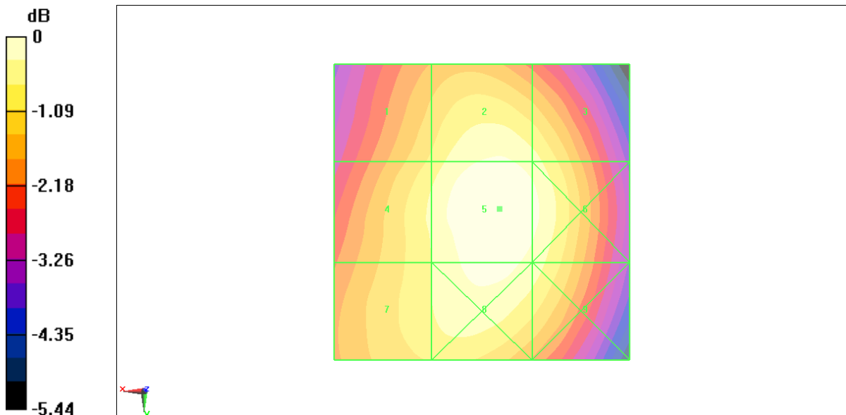
Fig B.8 HAC RF E-Field WCDMA 850 Middle
