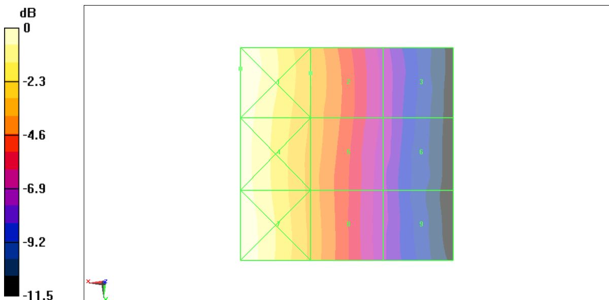
Fig B.15 HAC RF H-Field GSM 850 Low
