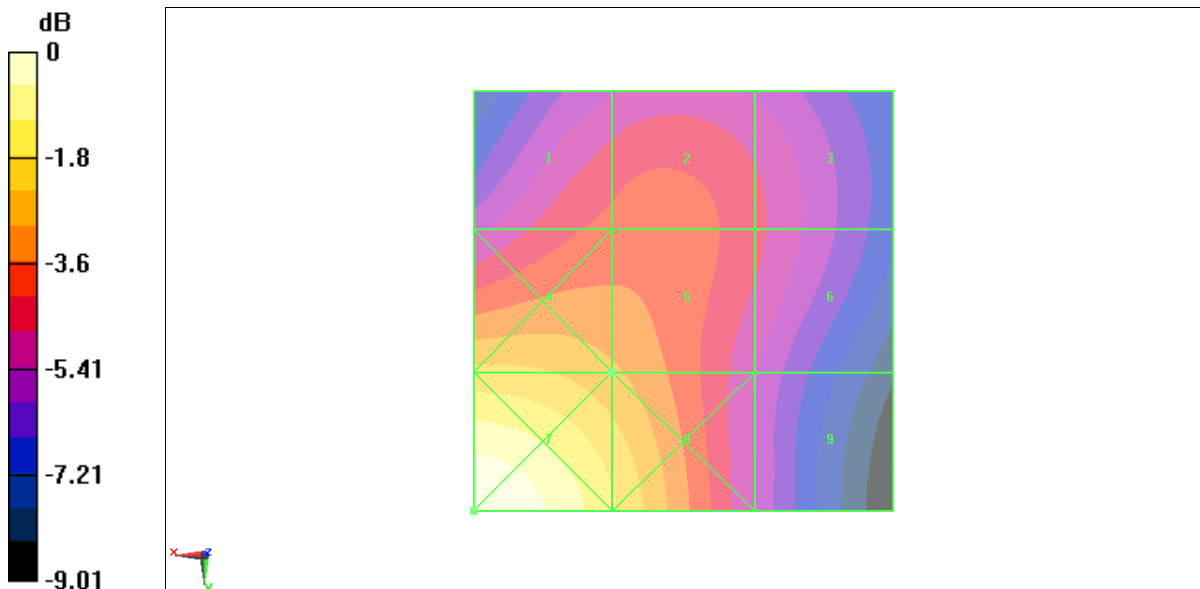
Fig B.22 HAC RF H-Field WCDMA 1900 High
