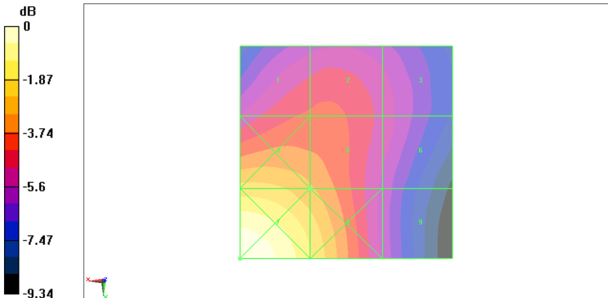
Fig B.17 HAC RF H-Field GSM 1900 Middle
