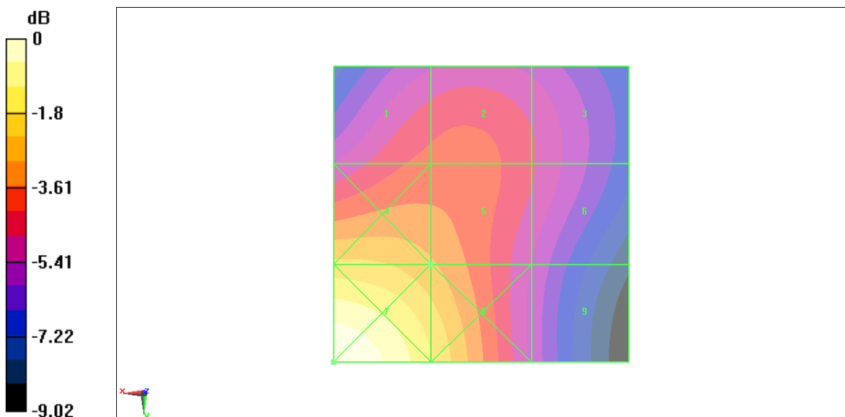
Fig B.23 HAC RF H-Field WCDMA 1900 Middle
