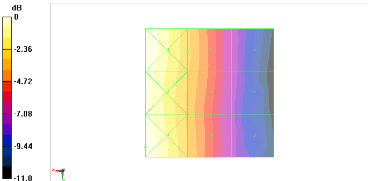
Fig B.21 HAC RF H-Field WCDMA 850 Low
