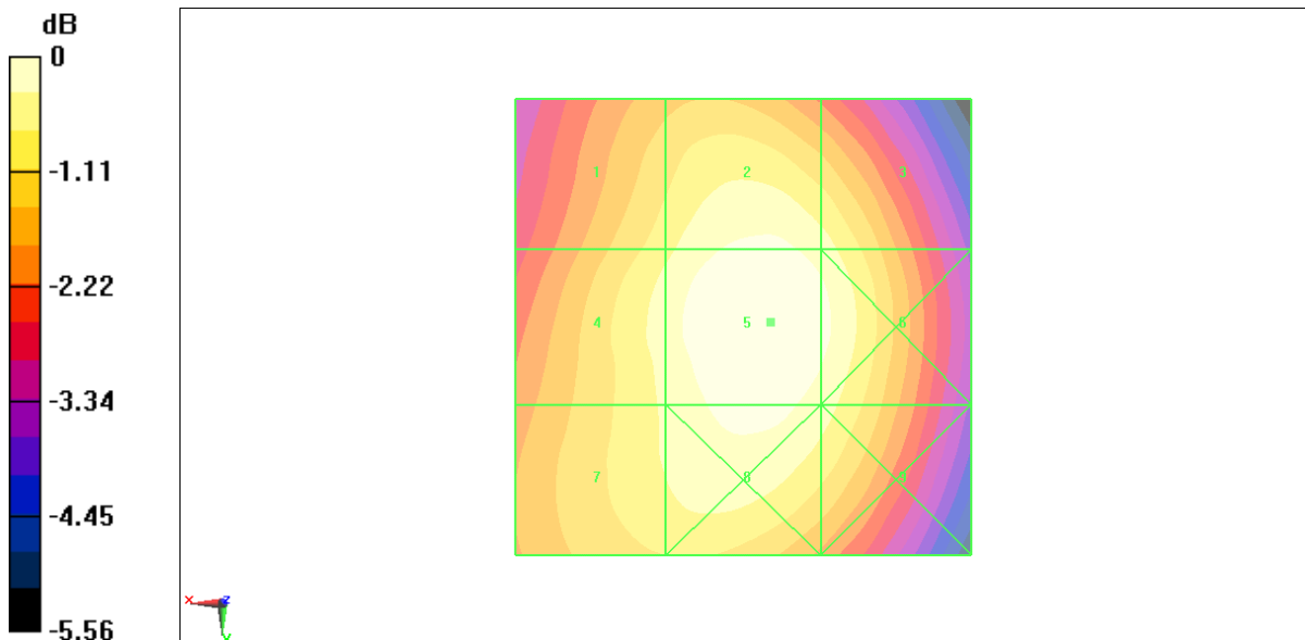
Fig B.9 HAC RF E-Field WCDMA 850 Low
