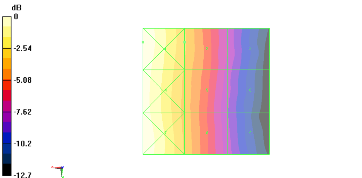
Fig B.13 HAC RF H-Field GSM 850 High
