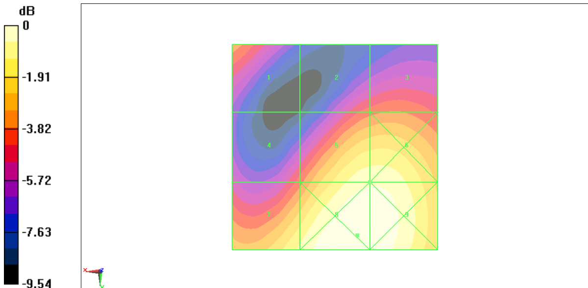
Fig B.10 HAC RF E-Field WCDMA 1900 High
