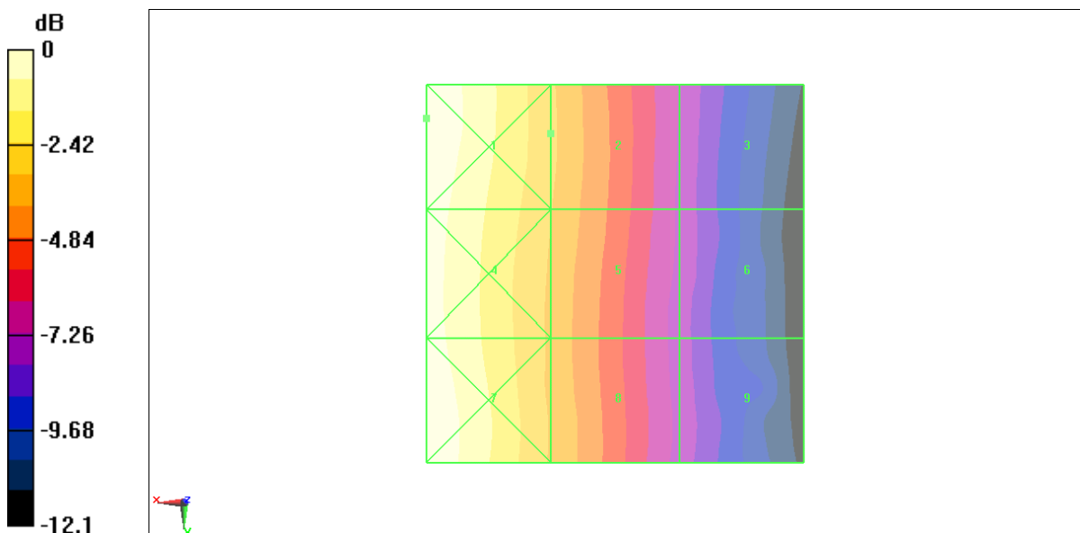
Fig B.20 HAC RF H-Field WCDMA 850 Middle
