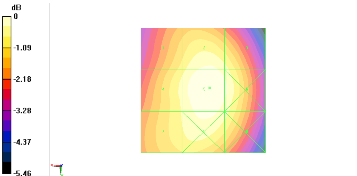
Fig B.7 HAC RF E-Field WCDMA 850 High
