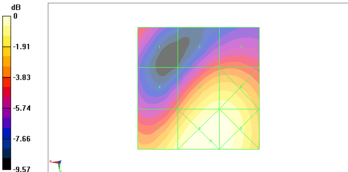
Fig B.12 HAC RF E-Field WCDMA 1900 Low
