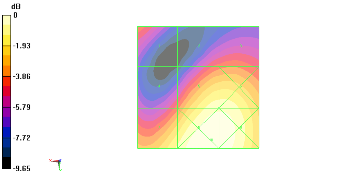
Fig B.11 HAC RF E-Field WCDMA 1900 Middle
