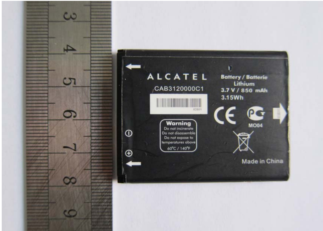
Battery CAB3120000C1
