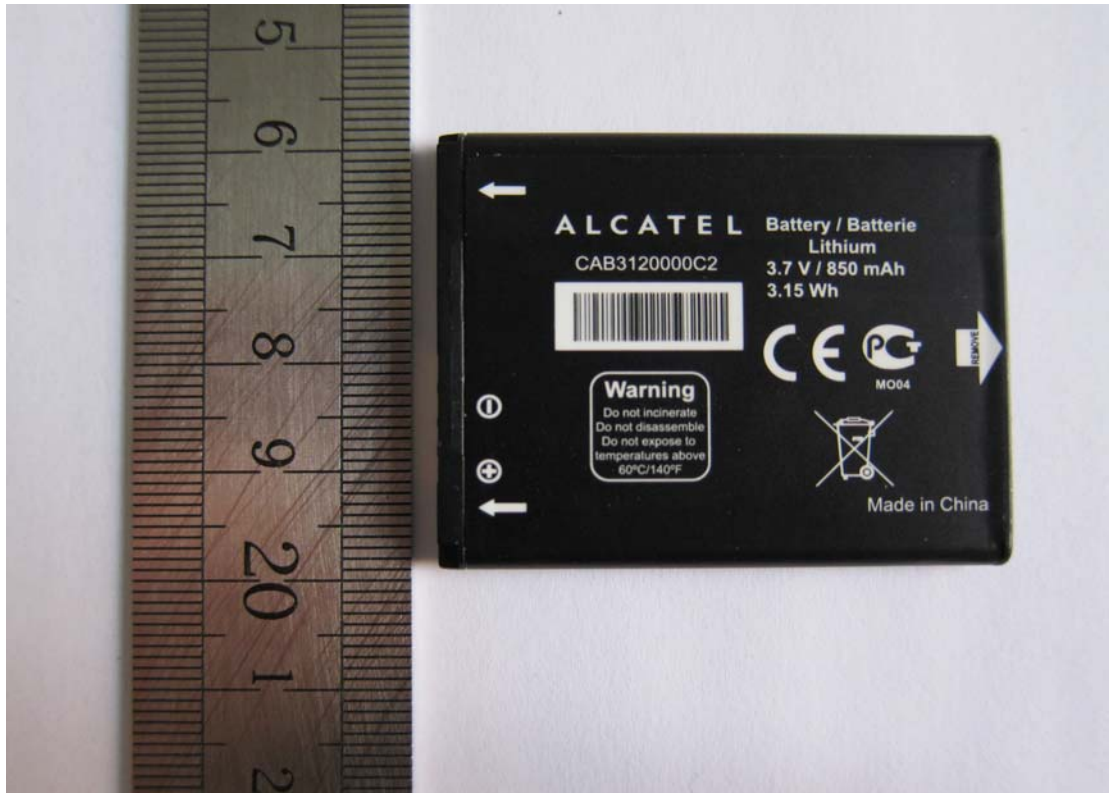
Battery CAB3120000C2
