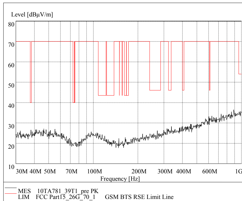
Fig.17 Radiated emission: GFSK, Channel 39, 30 MHz - 1 GHz
