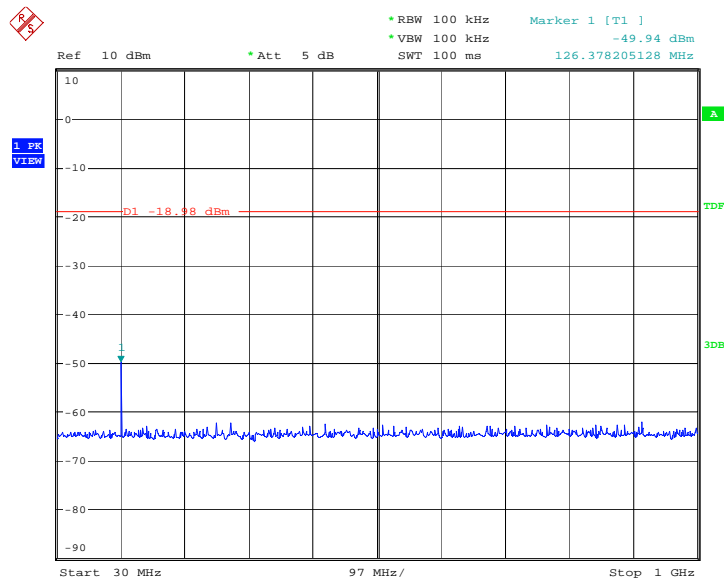
Fig.8 Conducted spurious emission: GFSK, Channel 39, 2441MHz
