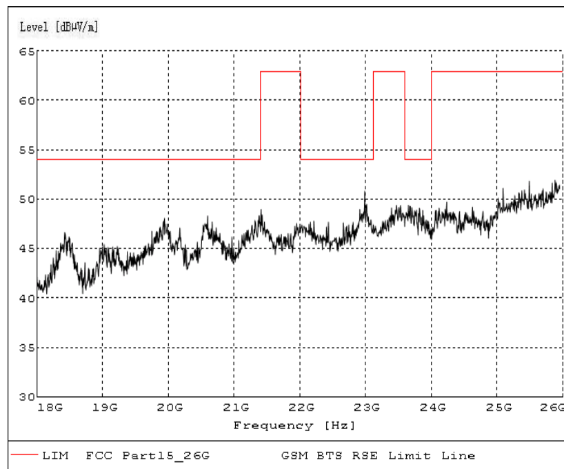
Fig.24 Radiated emission: GFSK, 18 GHz - 26 GHz
