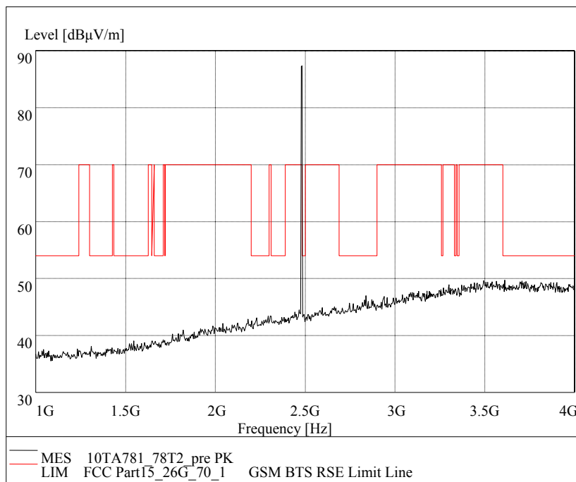
Fig.21 Radiated emission: GFSK, Channel 78, 1 GHz - 4 GHz
