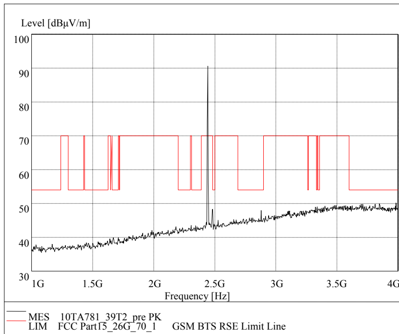
Fig.18 Radiated emission: GFSK, Channel 39, 1 GHz - 4 GHz
