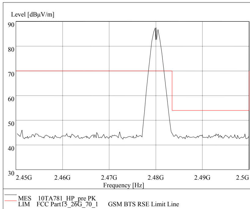
Fig.23 Radiated emission (Power): GFSK,
