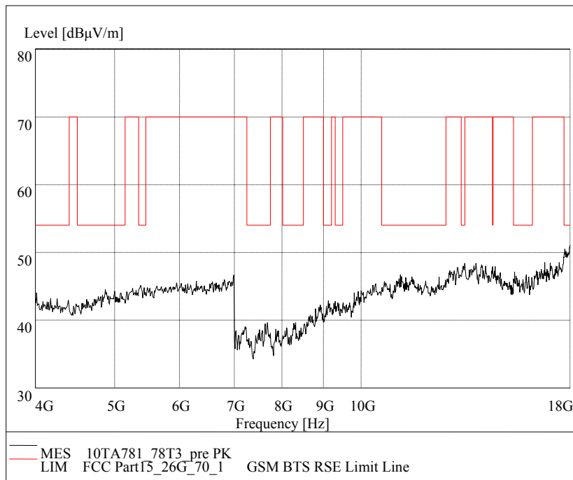
Fig.22 Radiated emission: GFSK, Channel 78, 4 GHz - 18 GHz
