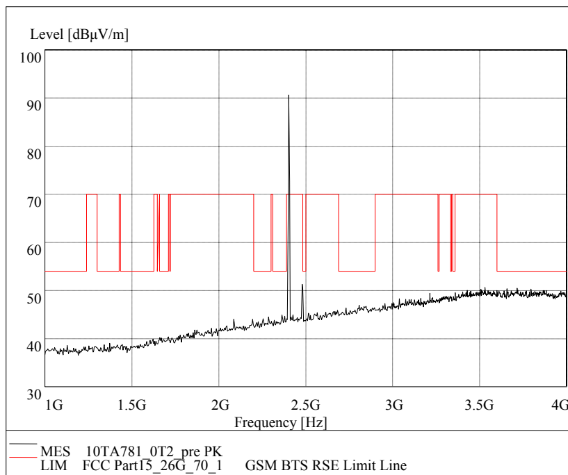
Fig.15 Radiated emission: GFSK, Channel 0, 1 GHz - 4 GHz
