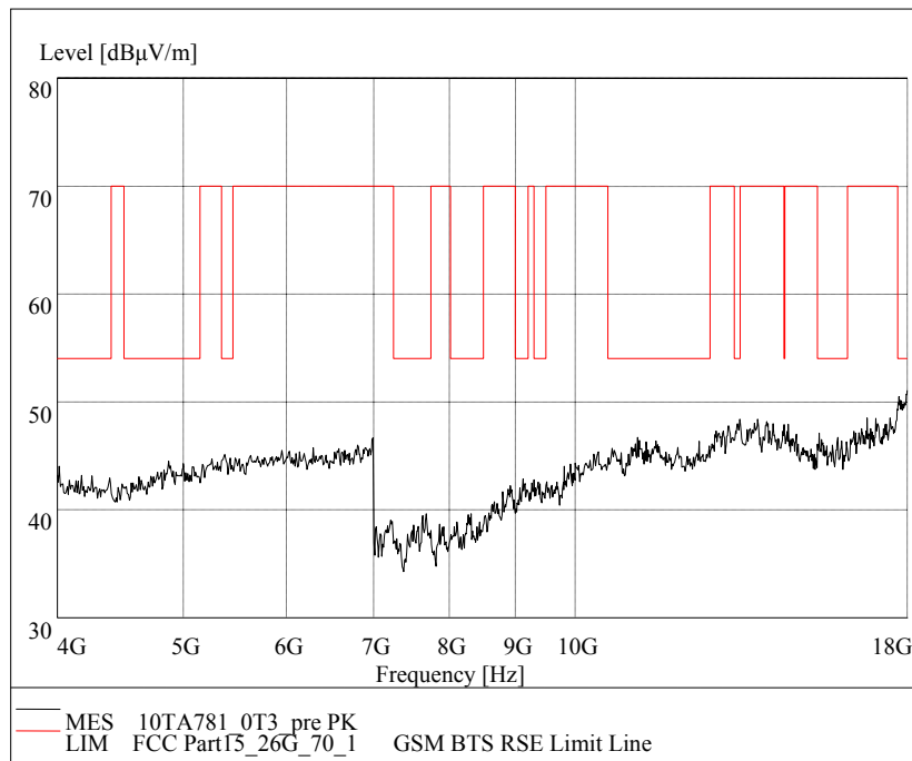
Fig.16 Radiated emission: GFSK, Channel 0, 4 GHz - 18 GHz
