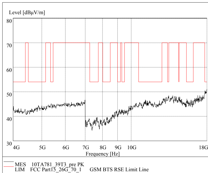
Fig.19 Radiated emission: GFSK, Channel 39, 4 GHz - 18 GHz
