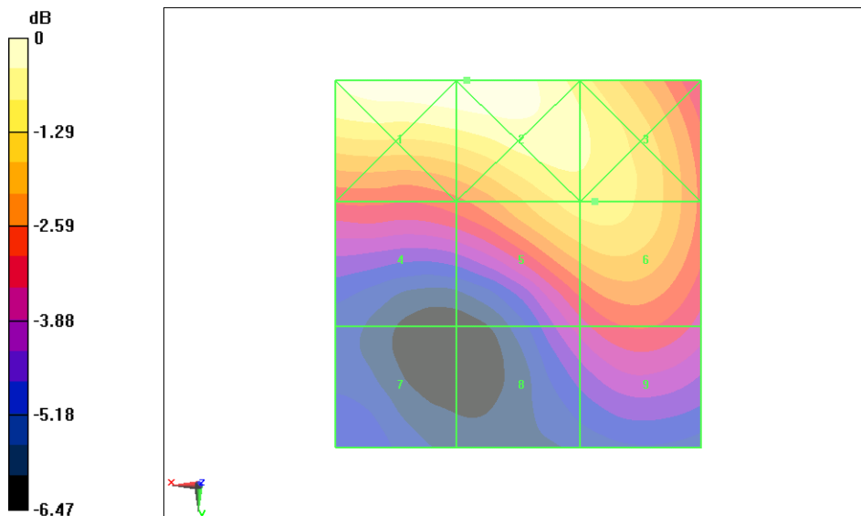
Fig B.6 HAC RF E-Field GSM 1900 Low
