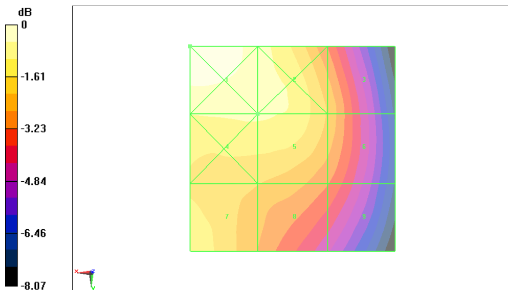
Fig B.7 HAC RF H-Field GSM 850 High
