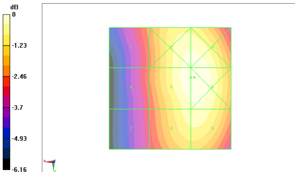
Fig B.3 HAC RF E-Field GSM 850 Low
