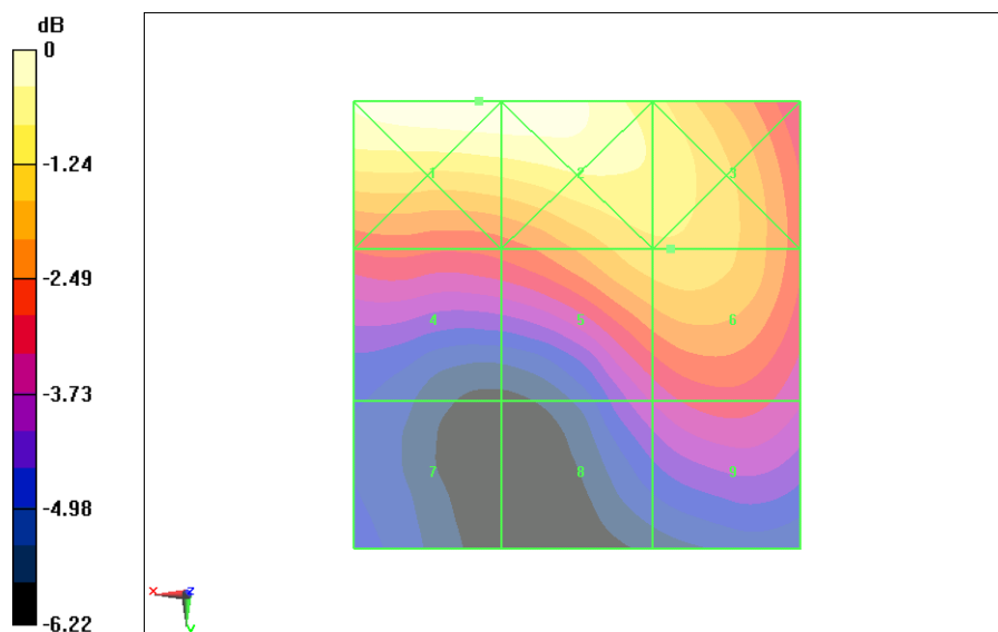
Fig B.5 HAC RF E-Field GSM 1900 Middle
