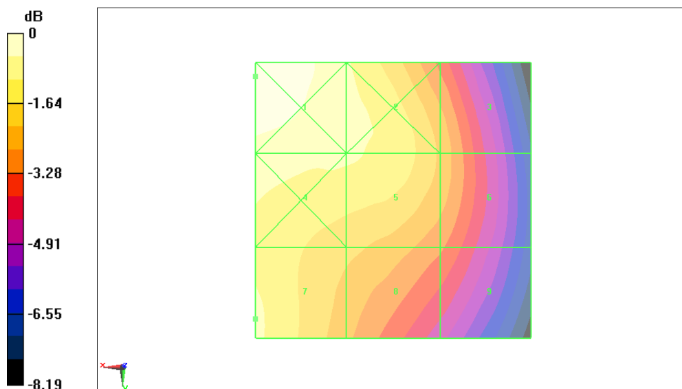
Fig B.9 HAC RF H-Field GSM 850 Low
