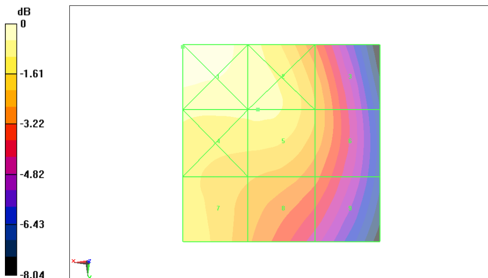
Fig B.8 HAC RF H-Field GSM 850 Middle
