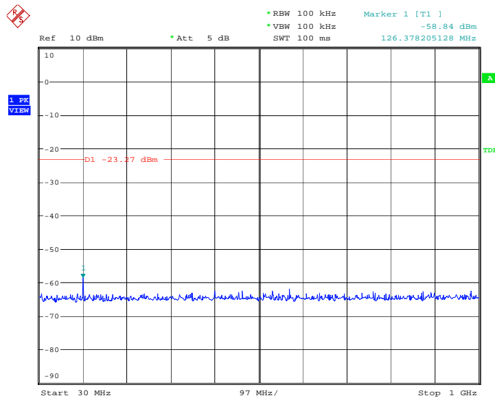
Fig.8 Conducted spurious emission: GFSK, Channel 39, 2441MHz
