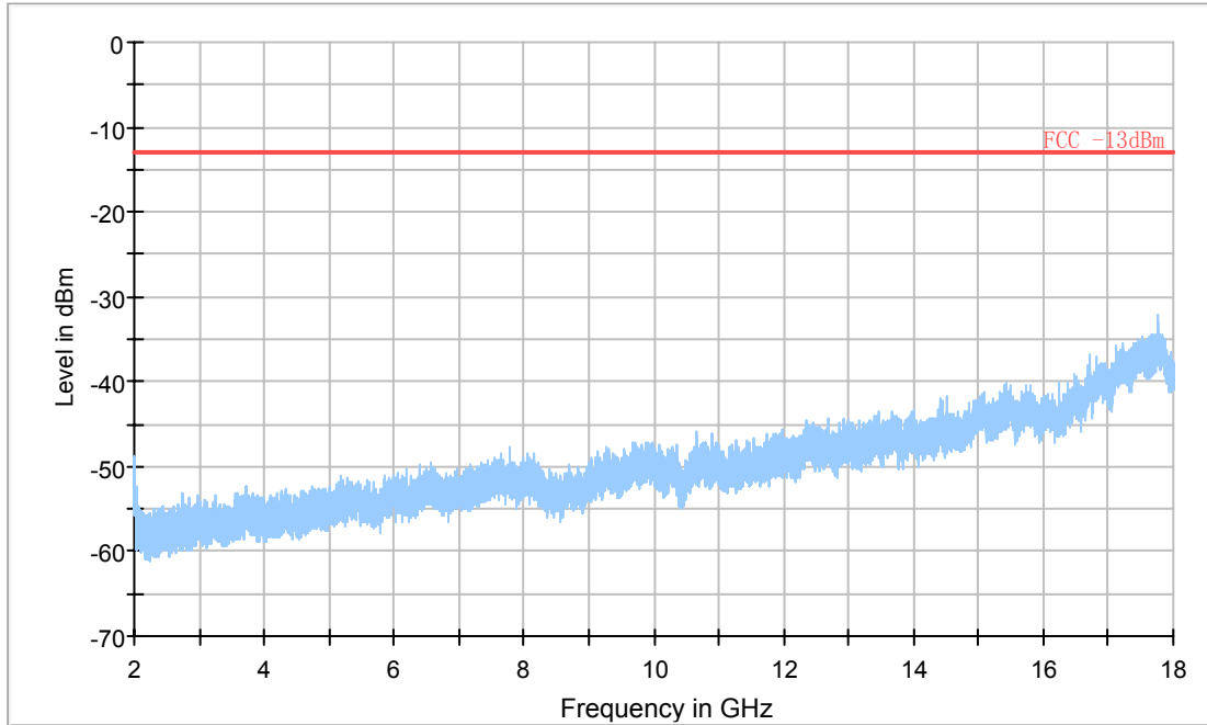
FCC24 2-18 GHz
