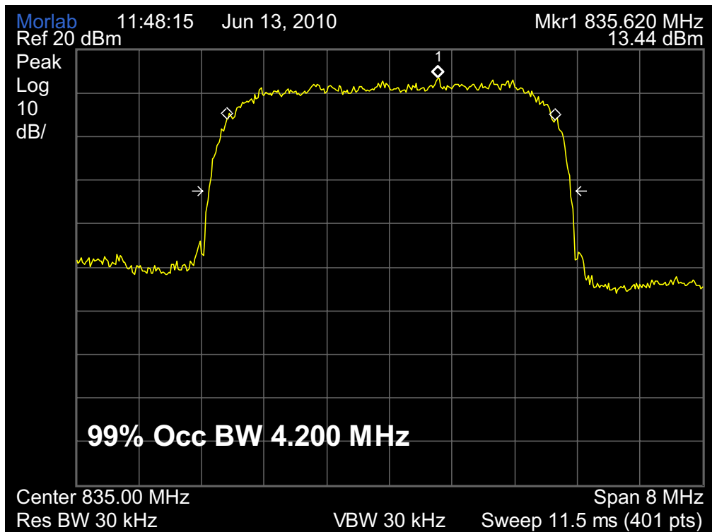
(Plot O: HSUPA 850MHz Channel = 4175)
