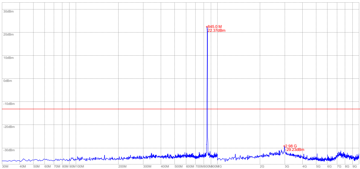
(Plot O: WCDMA 850MHz Channel = 4233, 30MHz to 10GHz)
