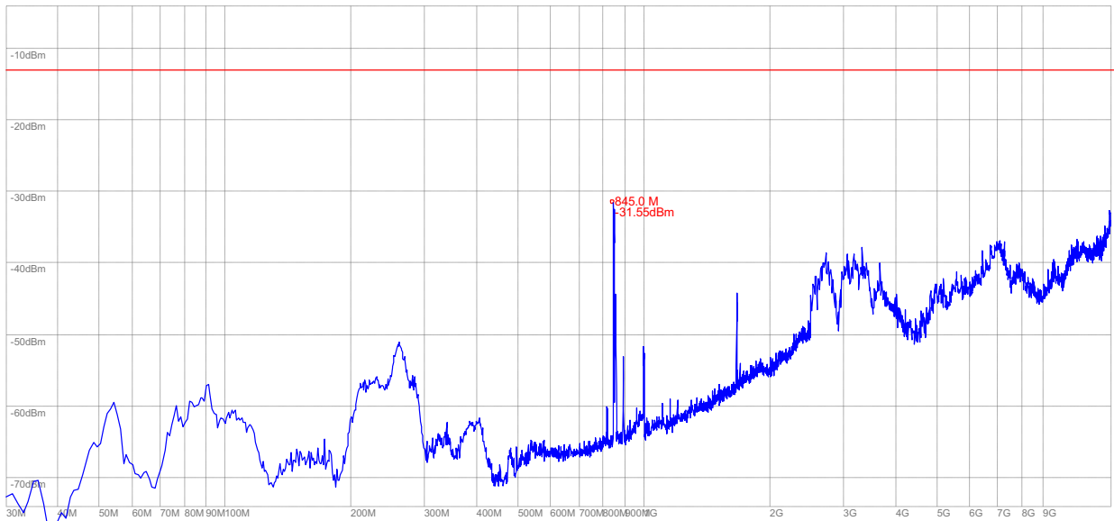
(Plot U.1: HSUPA 850MHz Channel = 4233, Test Antenna Horizontal)
