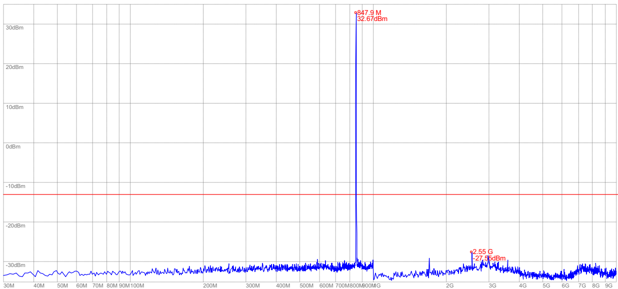
(Plot I: EDGE 850MHz Channel = 251, 30MHz to 10GHz)
