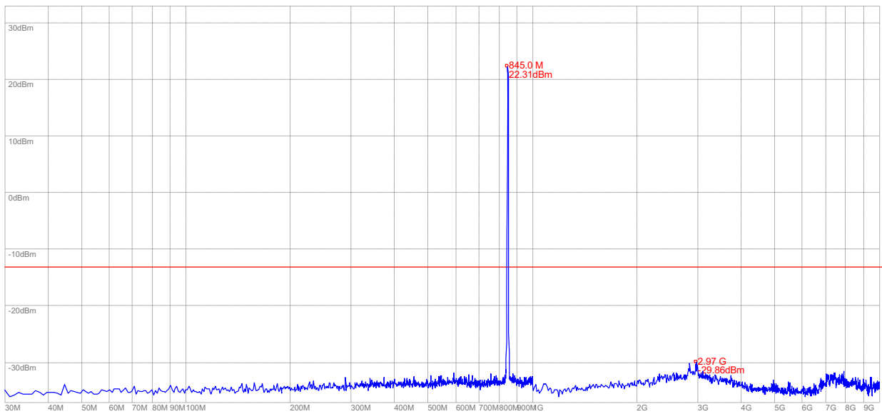
(Plot U: HSUPA 850MHz Channel = 4233, 30MHz to 10GHz)
