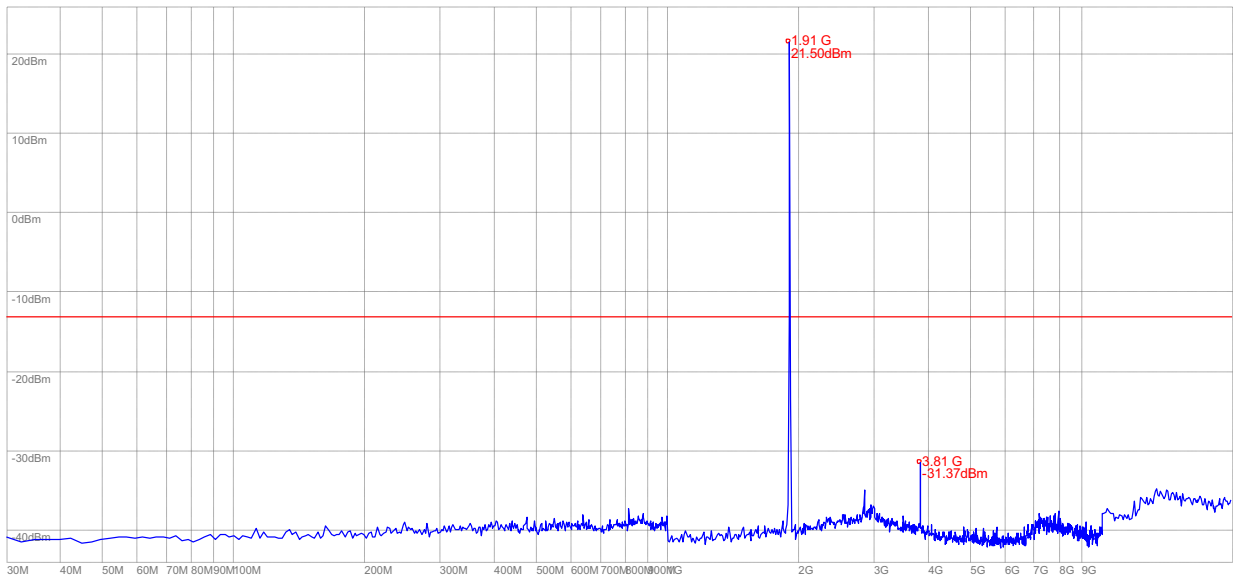
(Plot X: HSUPA 1900MHz Channel = 9538, 30MHz to 20GHz)
