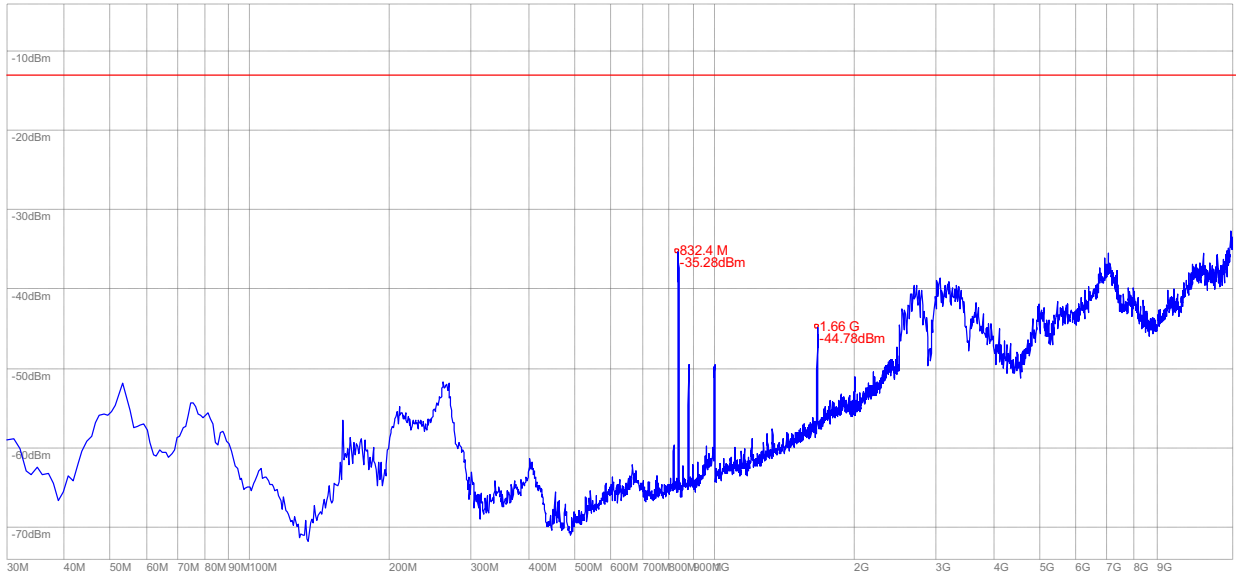
(Plot T.2: HSUPA 850MHz Channel = 4175, Test Antenna Vertical)
