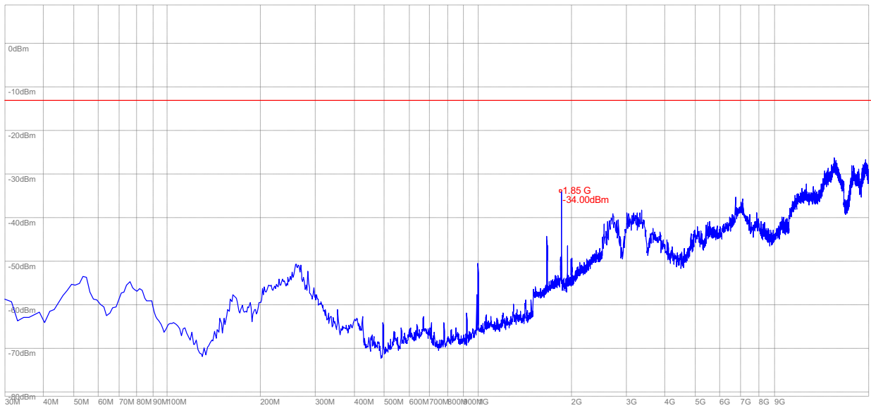
(Plot V.2: HSUPA 1900MHz Channel = 9262, Test Antenna Vertical)
