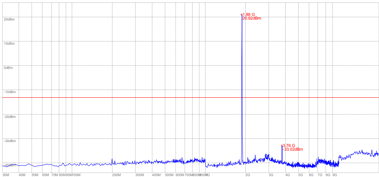
(Plot W: HSUPA 1900MHz Channel = 9400, 30MHz to 20GHz)
