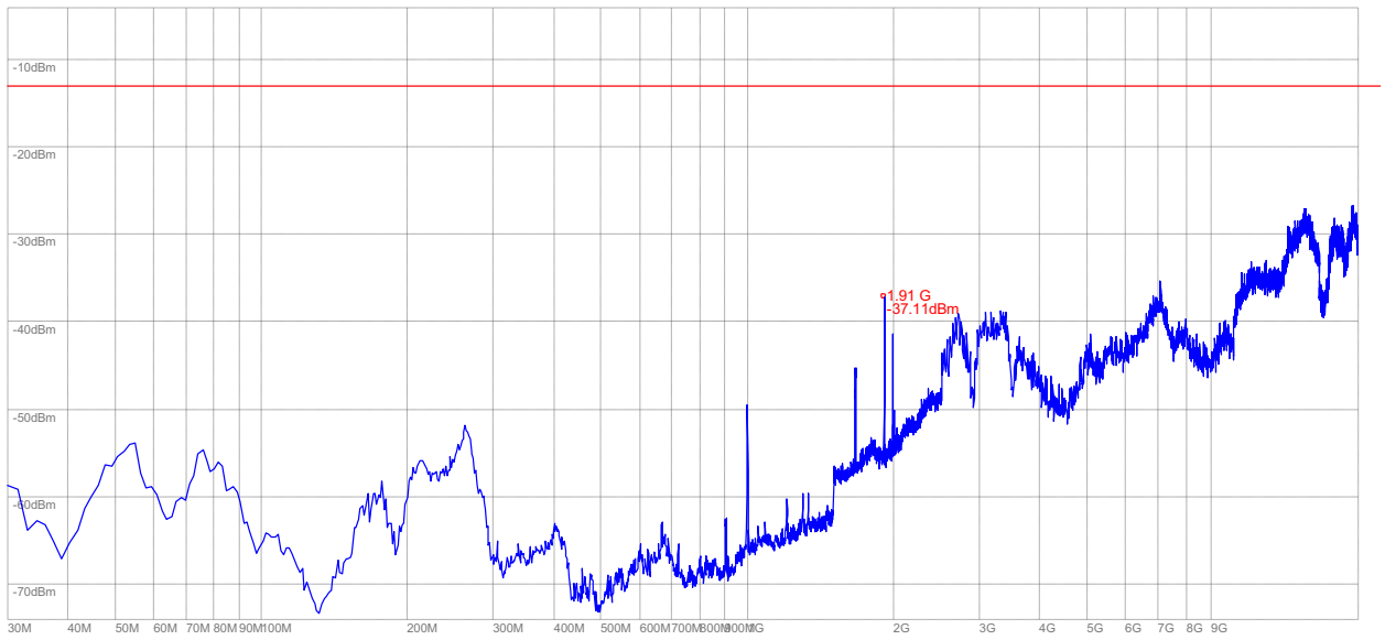
(Plot X.2: HSUPA 1900MHz Channel = 9538, Test Antenna Vertical)
