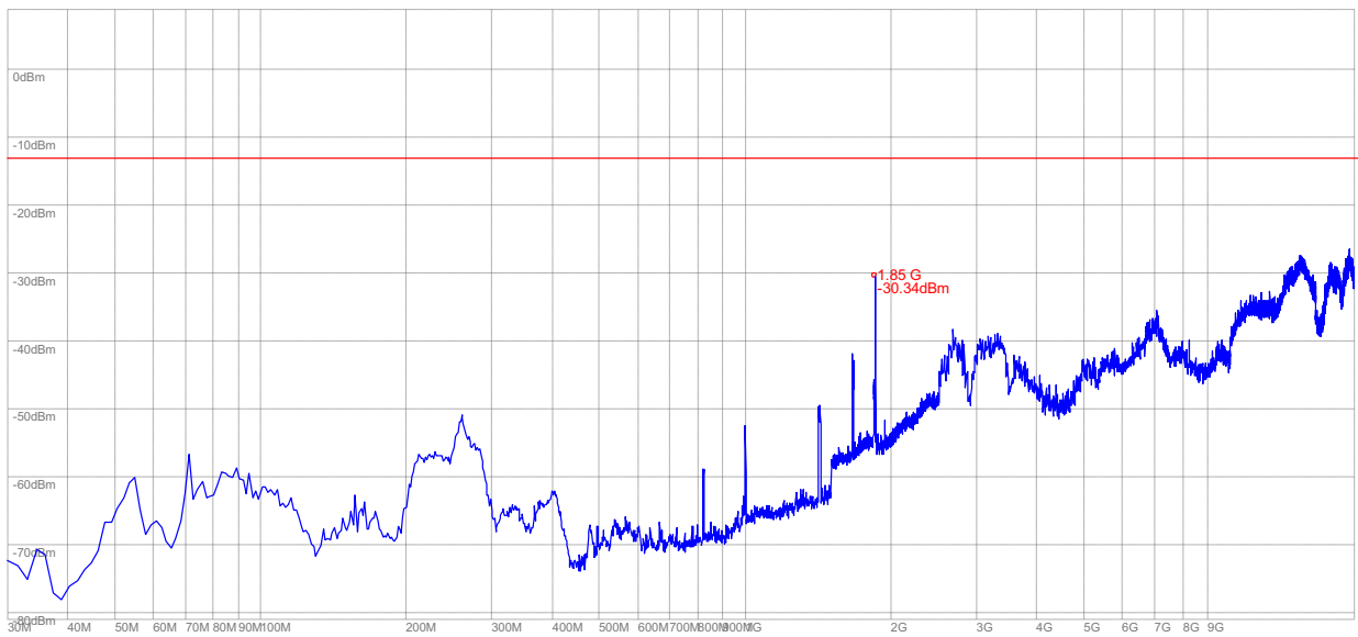
(Plot V.1: HSUPA 1900MHz Channel = 9262, Test Antenna Horizontal)
