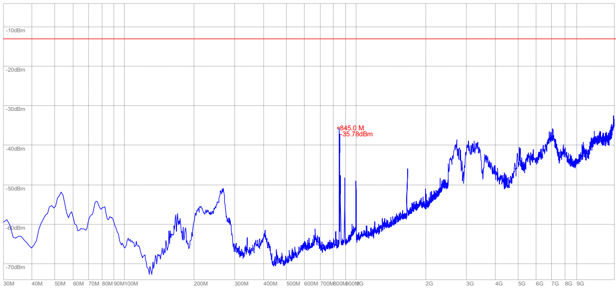
(Plot U.2: HSUPA 850MHz Channel = 4233, Test Antenna Vertical)
