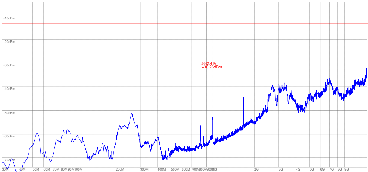
(Plot T.1: HSUPA 850MHz Channel = 4175, Test Antenna Horizontal)
