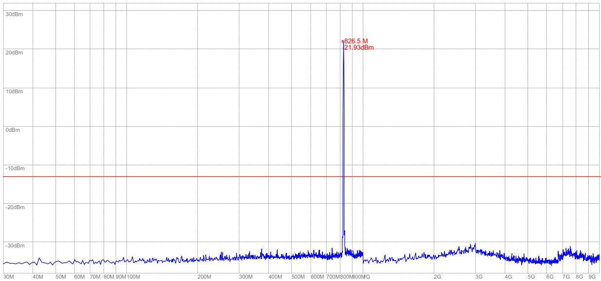
(Plot S: HSUPA 850MHz Channel = 4132, 30MHz to 10GHz)
