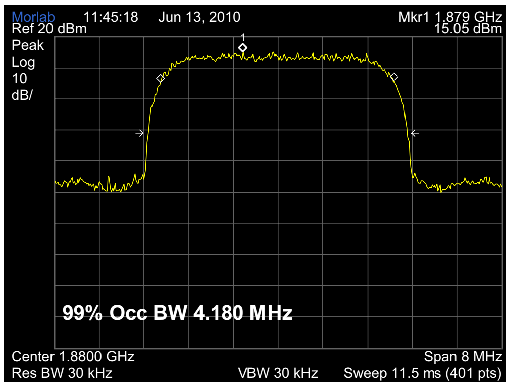
(Plot P: HSUPA 1900MHz Channel = 9400)
