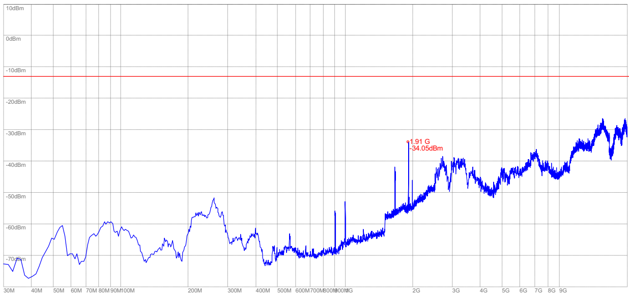
(Plot X.1: HSUPA 1900MHz Channel = 9538, Test Antenna Horizontal)
