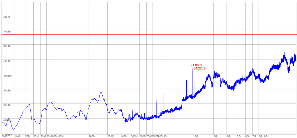
(Plot W.1: HSUPA 1900MHz Channel = 9400, Test Antenna Horizontal)
