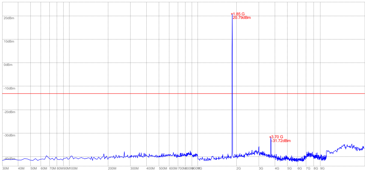
(Plot V: HSUPA 1900MHz Channel = 9262, 30MHz to 20GHz)
