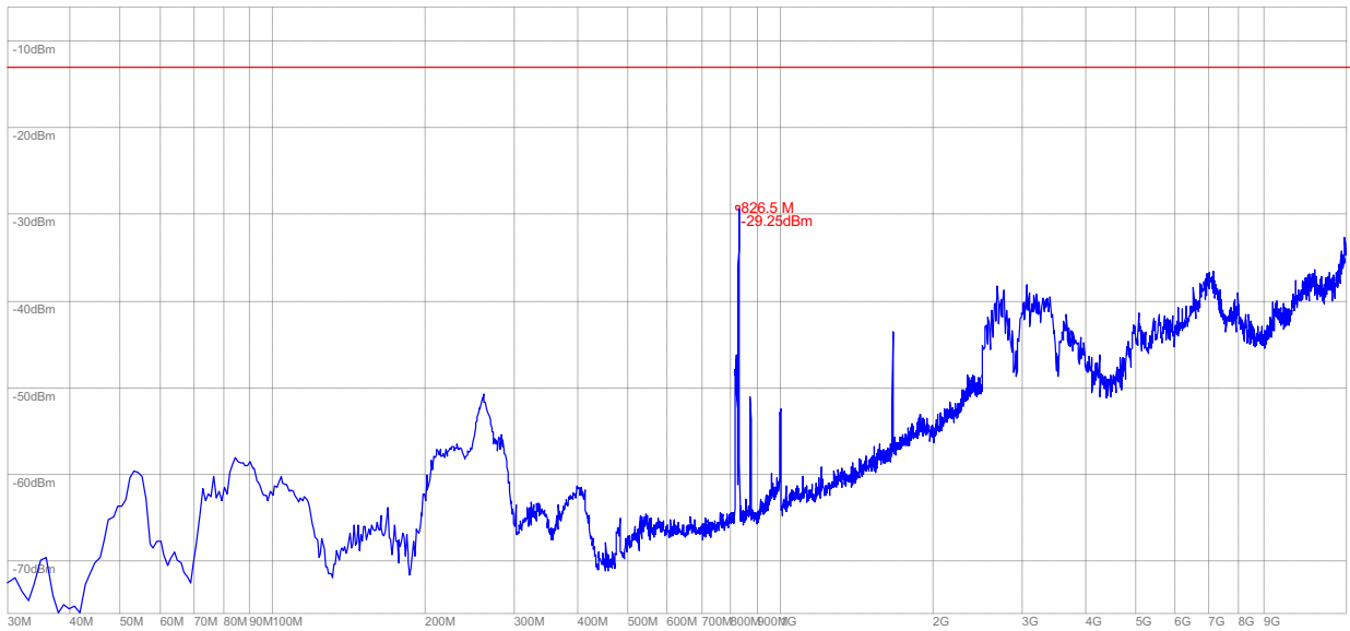
(Plot S.1: HSPA 850MHz Channel = 4132, Test Antenna Horizontal)
