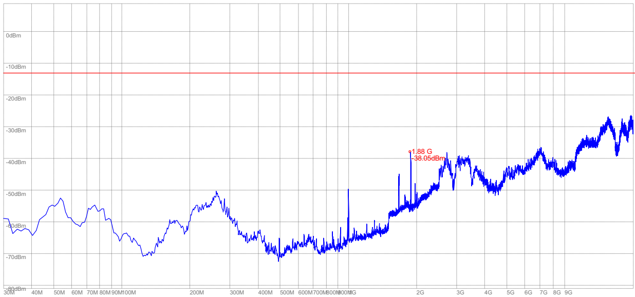
(Plot W.2: HSUPA 1900MHz Channel = 9400, Test Antenna Vertical)
