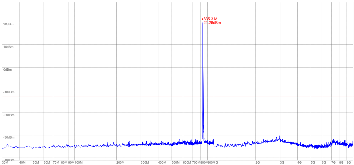
(Plot N: WCDMA 850MHz Channel = 4175, 30MHz to 10GHz)
