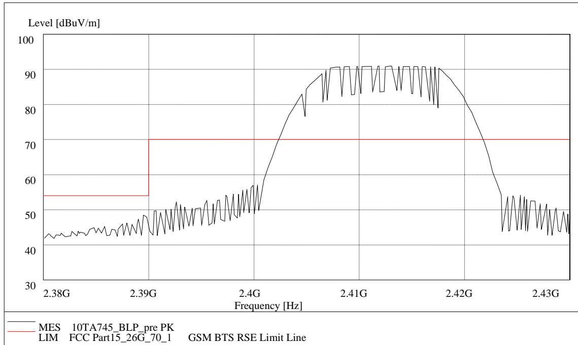
Fig. 35 Radiated Spurious Emission (Power): 802.11b, 2.38 GHz - 243GHz
