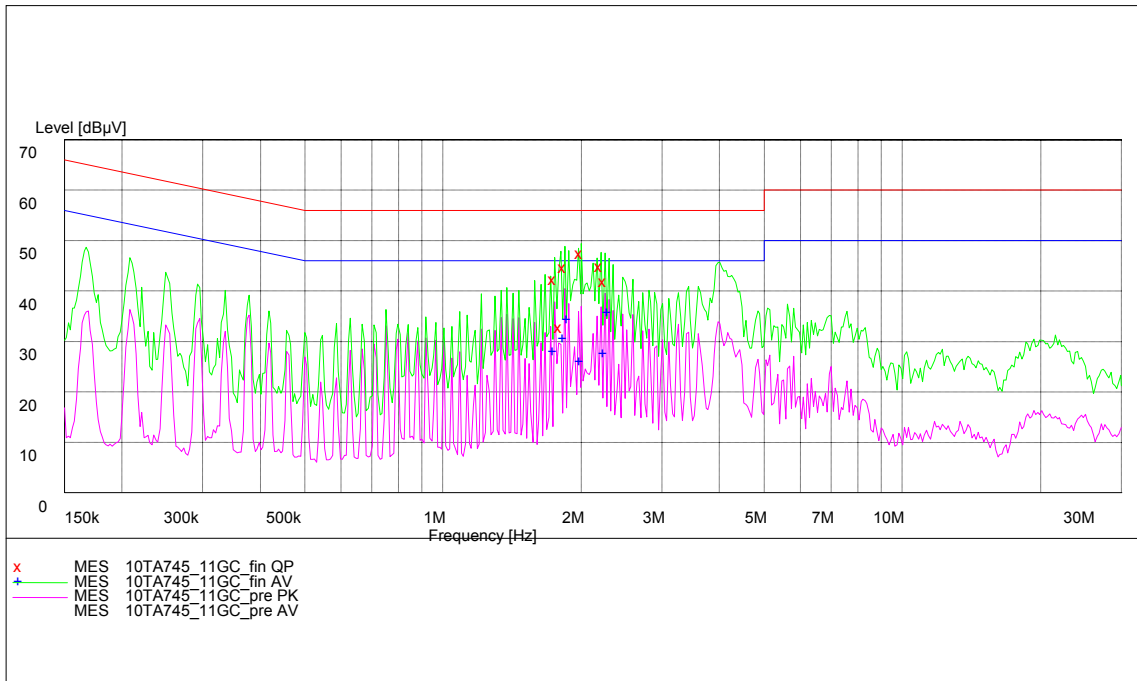
Fig. 57 AC Powerline Conducted Emission-802.11g
