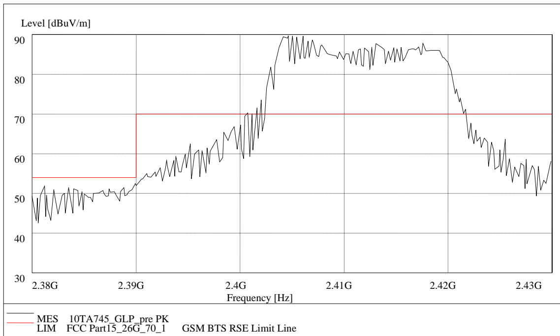
Fig. 45 Radiated Spurious Emission (Power): 802.11g, 2.38 GHz - 2.43GHz
