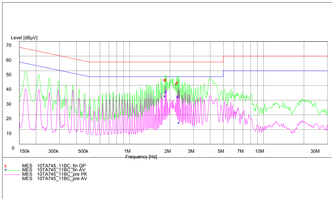
Fig. 56 AC Powerline Conducted Emission-802.11b
