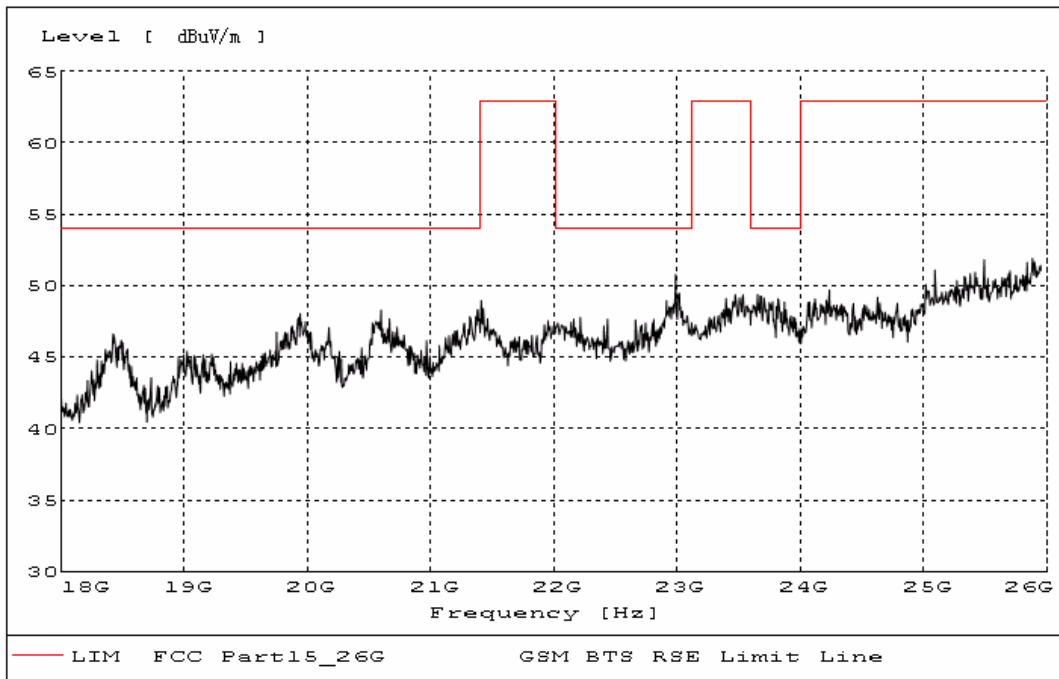
Fig. 55 Radiated emission: 18 GHz - 26 GHz
