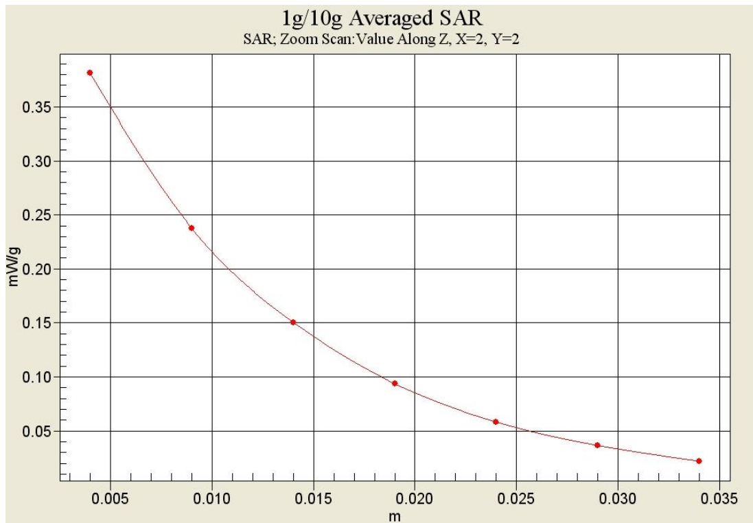
Fig. 35-1 Z-Scan at power reference point (1900 MHz CH512)
