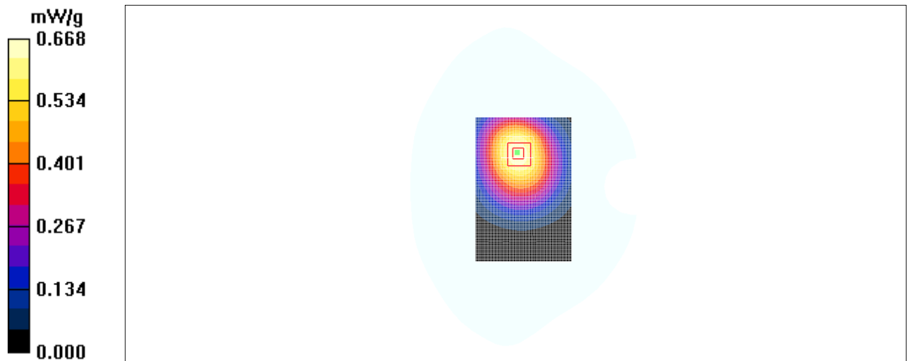
Fig. 30 850 MHz CH128
