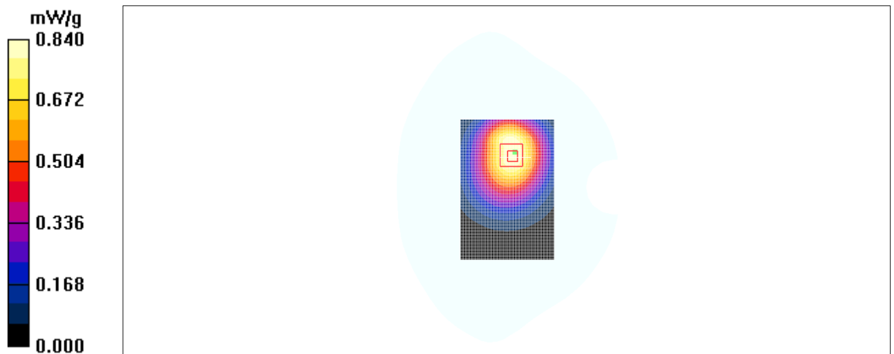
Fig. 27 850 MHz CH128
