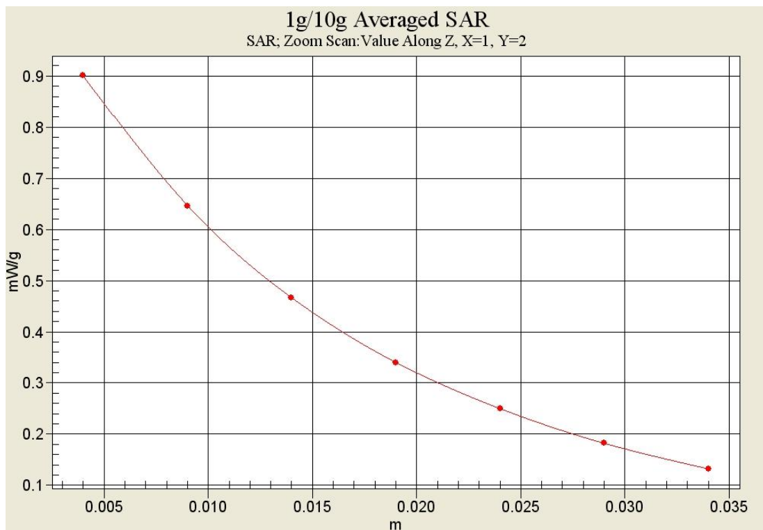
Fig. 25-1 Z-Scan at power reference point (850 MHz CH251)
