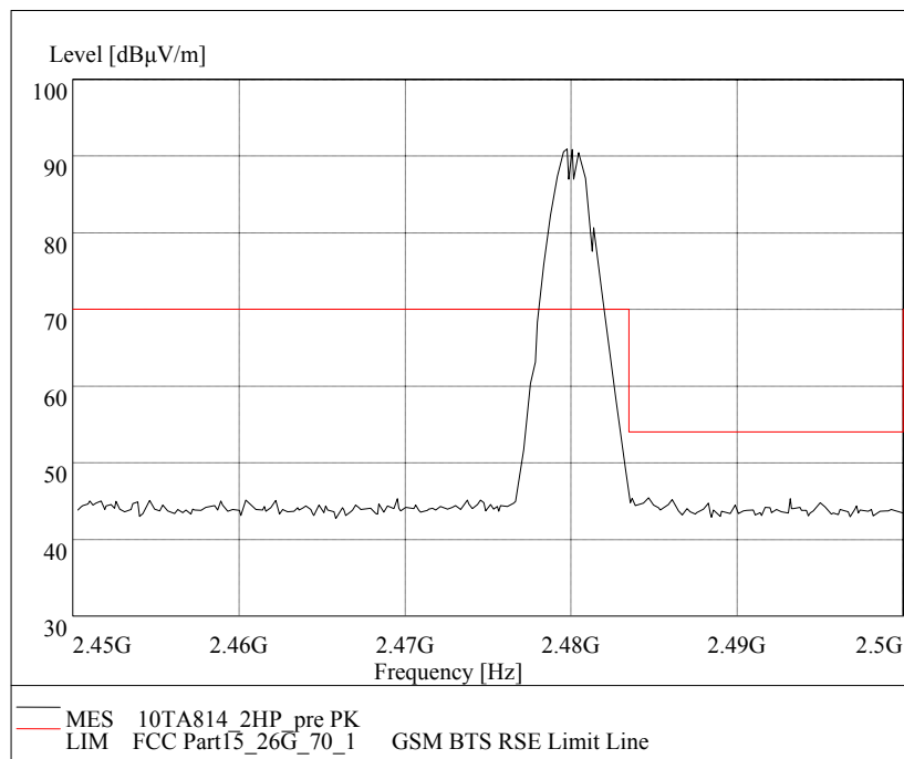
Fig.60 Radiated emission (Power): \pi/4 DQPSK
