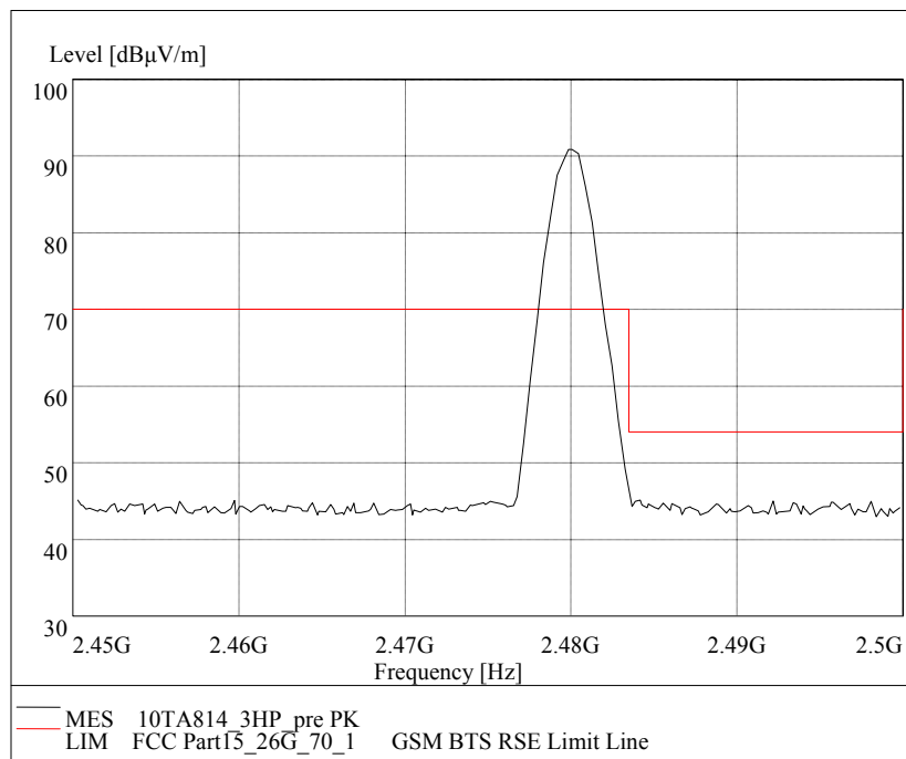
Fig.71 Radiated emission (Power): 8DPSK Level [dBµV/m]
