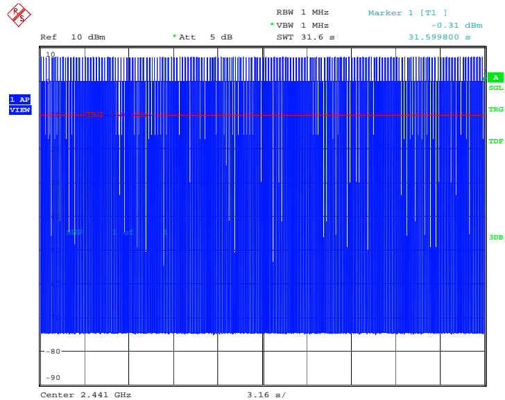
Fig.73 Time of occupancy (Dwell Time): Channel 39, Packet DH1
