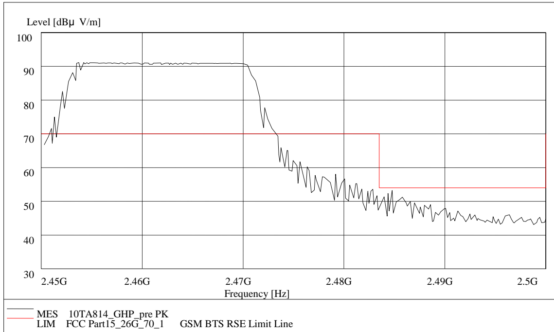
Fig. 53 Radiated Spurious Emission (Power): 802.11b, 2.45 GHz - 2.50GHz
