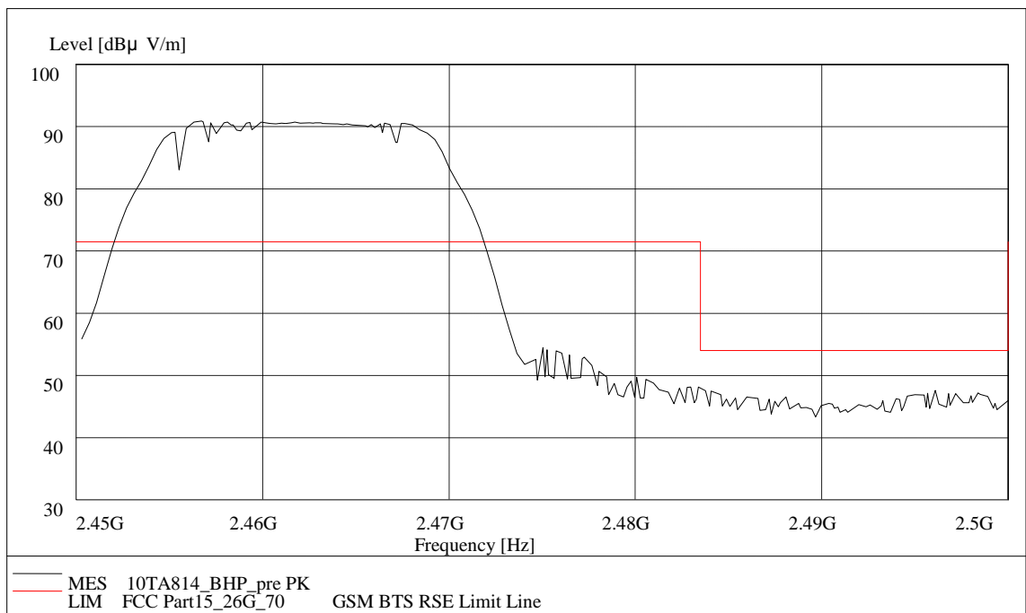
Fig. 42 Radiated Spurious Emission (Power): 802.11b, 2.45 GHz - 2.50GHz
