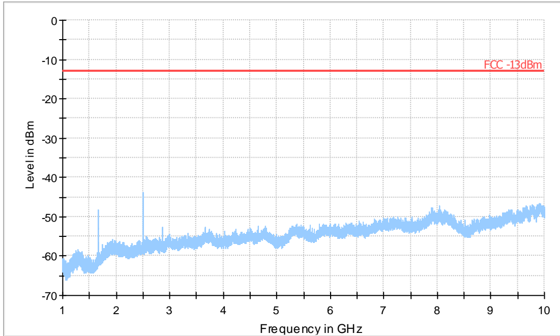
FCC22 1-10 GHz
