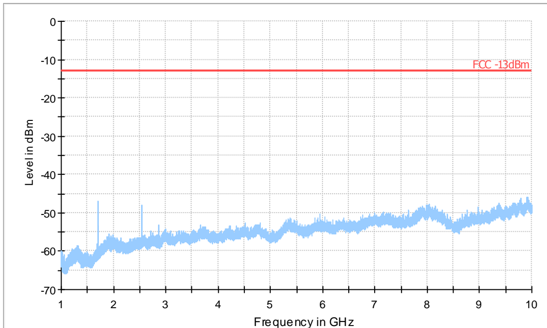
FCC22 1-10 GHz
