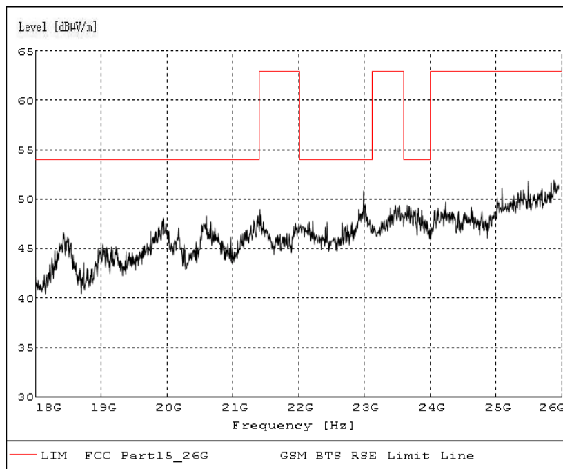
Fig.72 Radiated emission: 8DPSK, 18 GHz - 26 GHz
