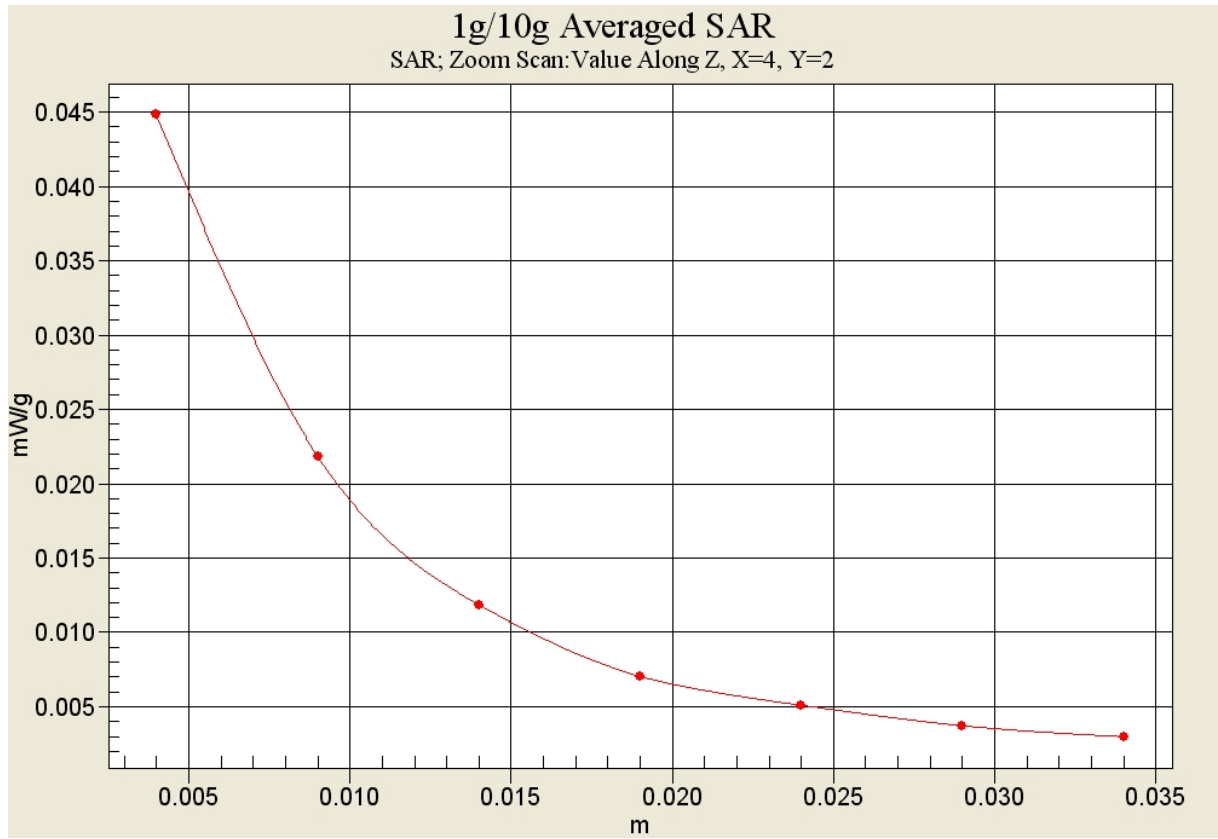
Fig. 186-1 Z-Scan at power reference point (802.11g 36Mbps CH11)
