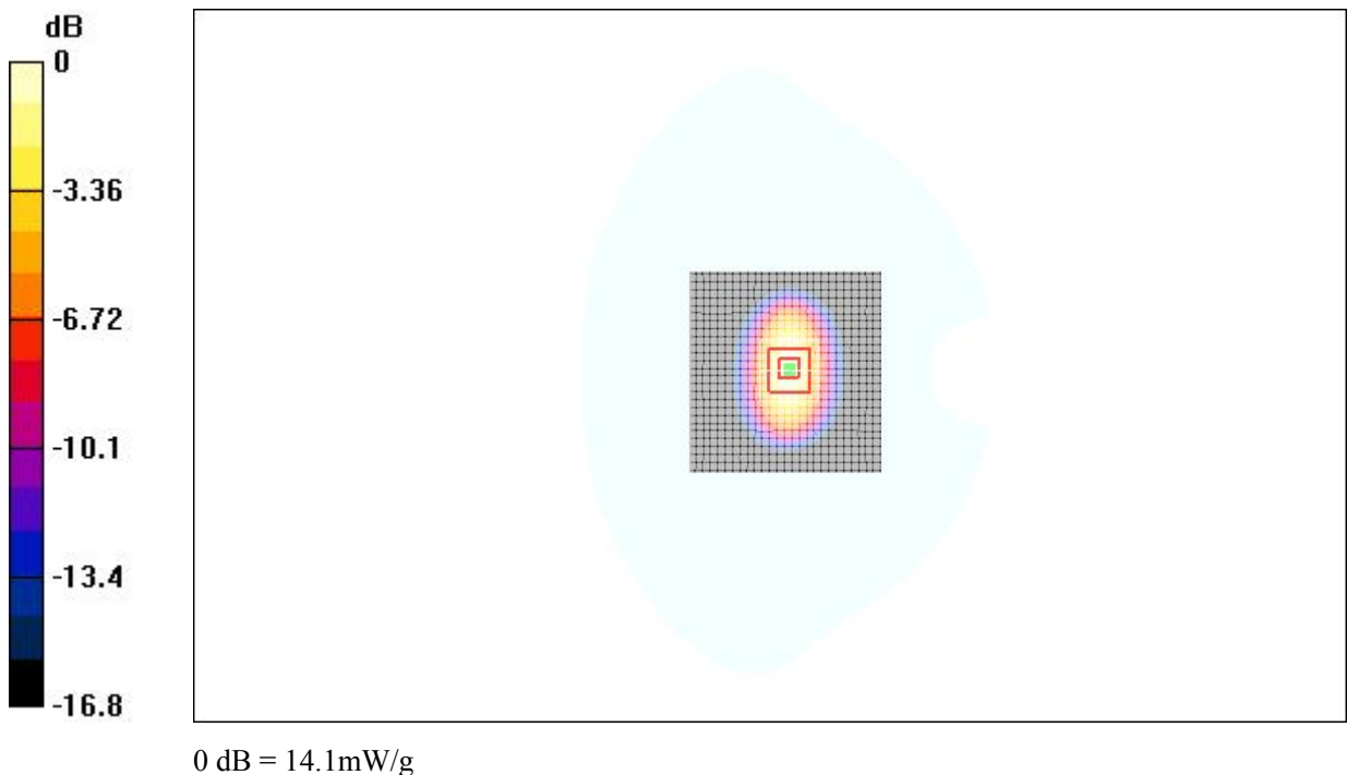
Fig.191 validation 2450MHz 250mW
