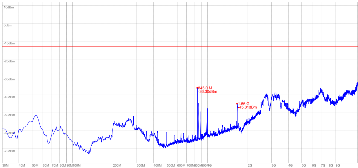
(Plot O.2: WCDMA 850MHz Channel = 4233, Test Antenna Vertical)
