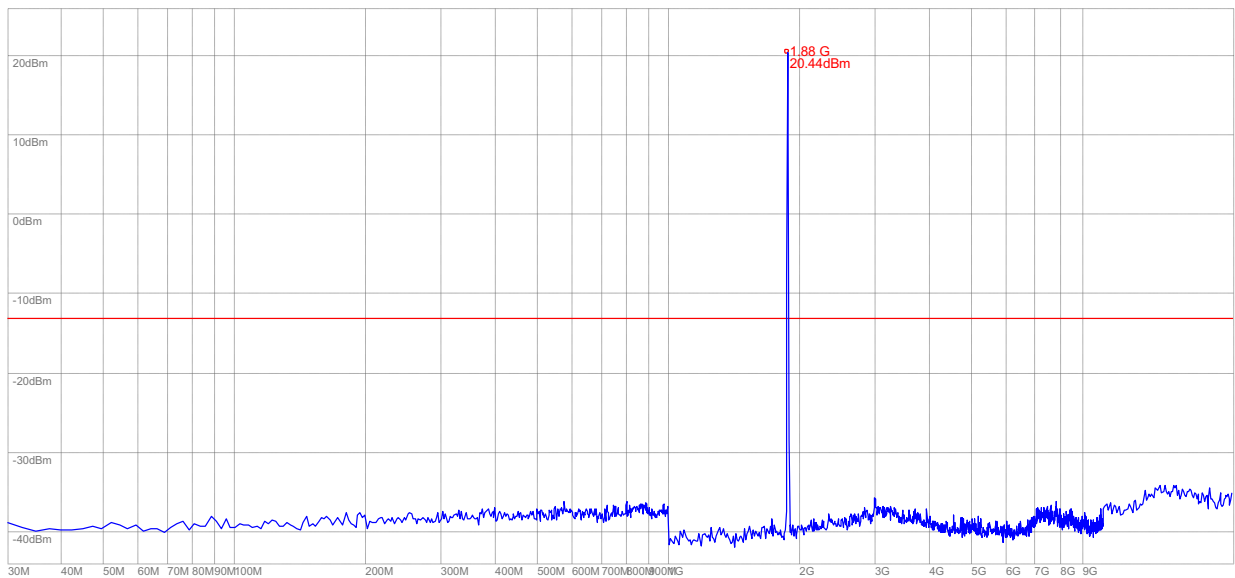
(Plot W: HSDPA 1900MHz Channel = 9400, 30MHz to 20GHz)
