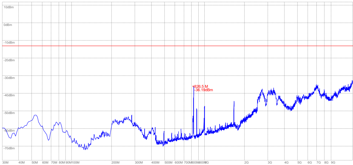
(Plot S.2: HSDPA 850MHz Channel = 4132, Test Antenna Vertical)
