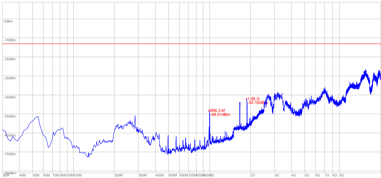
(Plot Q.2: WCDMA 1900MHz Channel = 9400, Test Antenna Vertical)
