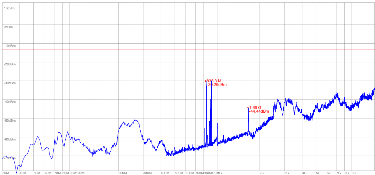
(Plot T.1: HSDPA 850MHz Channel = 4175, Test Antenna Horizontal)
