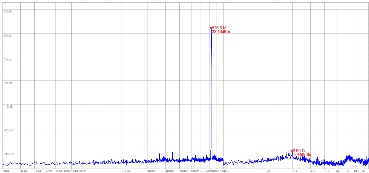
(Plot M: WCDMA 850MHz Channel = 4132, 30MHz to 10GHz)
