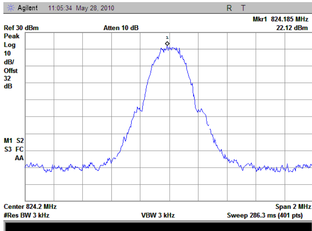
(Plot E: EDGE 850MHz Channel = 128)
