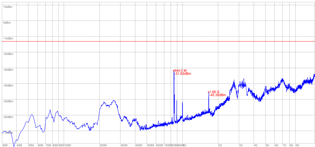
(Plot O.1: WCDMA 850MHz Channel = 4233, Test Antenna Horizontal)
