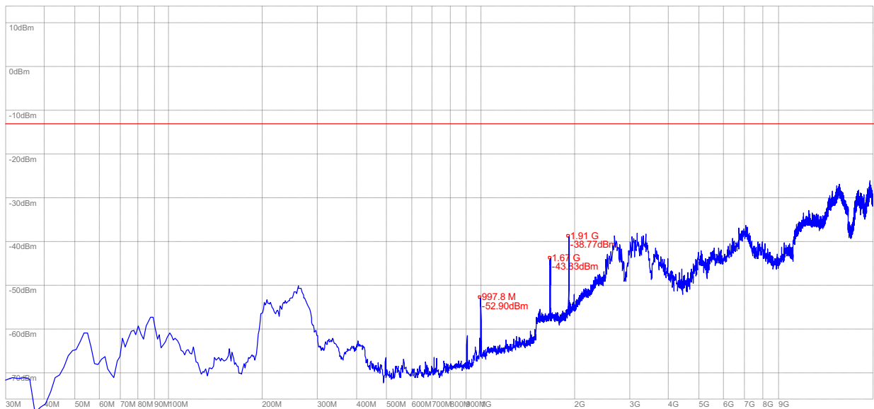
(Plot R.1: WCDMA 1900MHz Channel = 9538, Test Antenna Horizontal)
