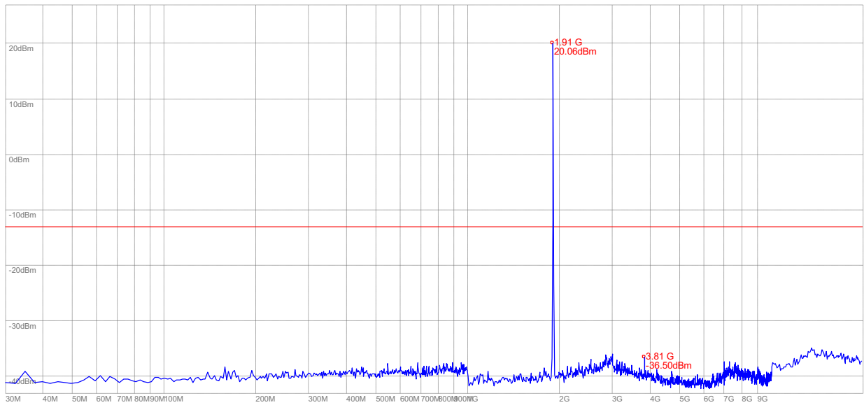
(Plot R: WCDMA 1900MHz Channel = 9538, 30MHz to 20GHz)
