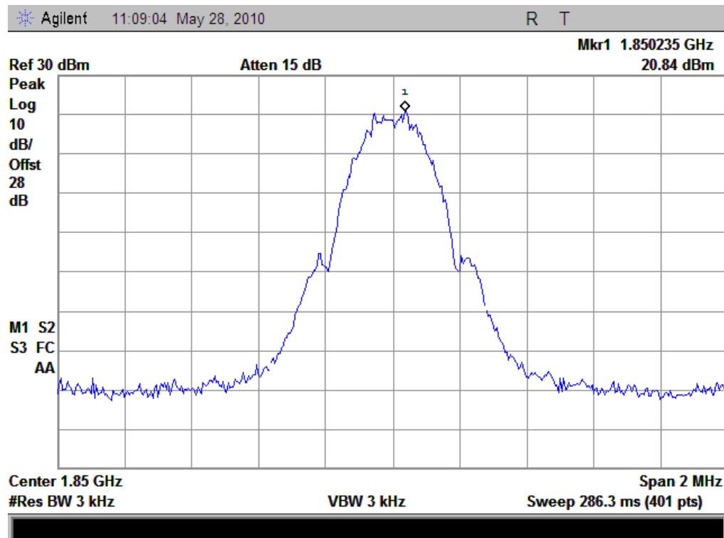
(Plot G: EDGE 1900MHz Channel = 512)
