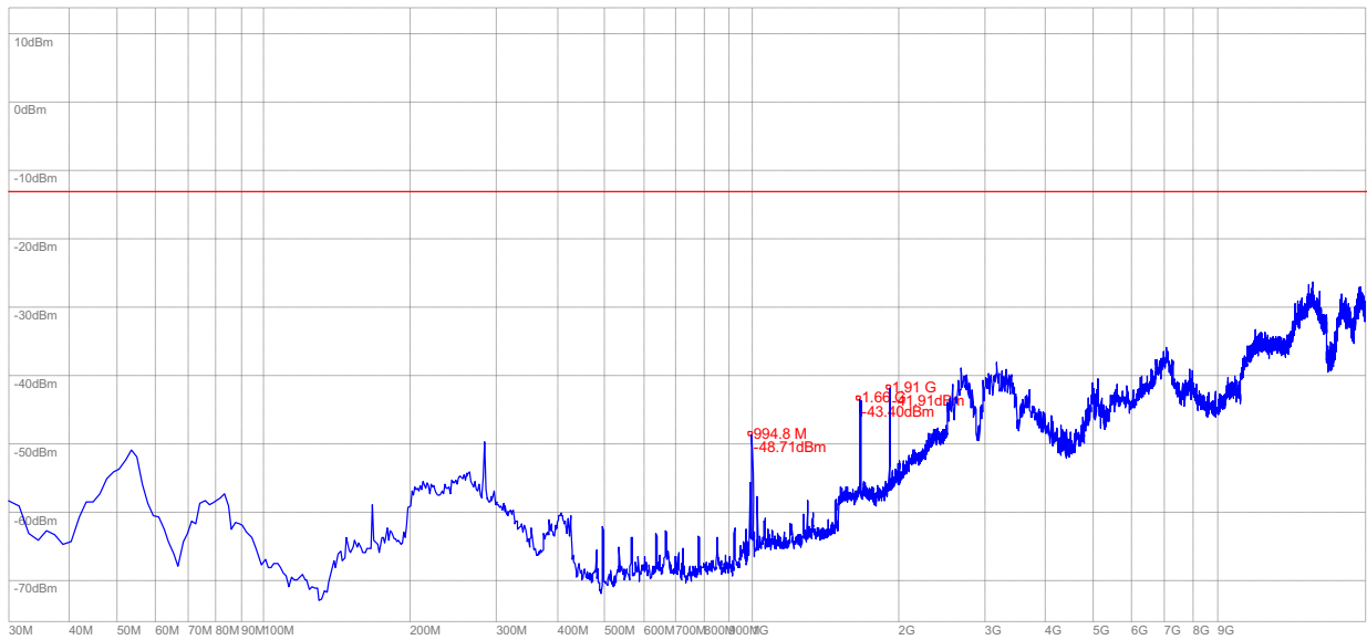
(Plot R.2: WCDMA 1900MHz Channel = 9538, Test Antenna Vertical)
