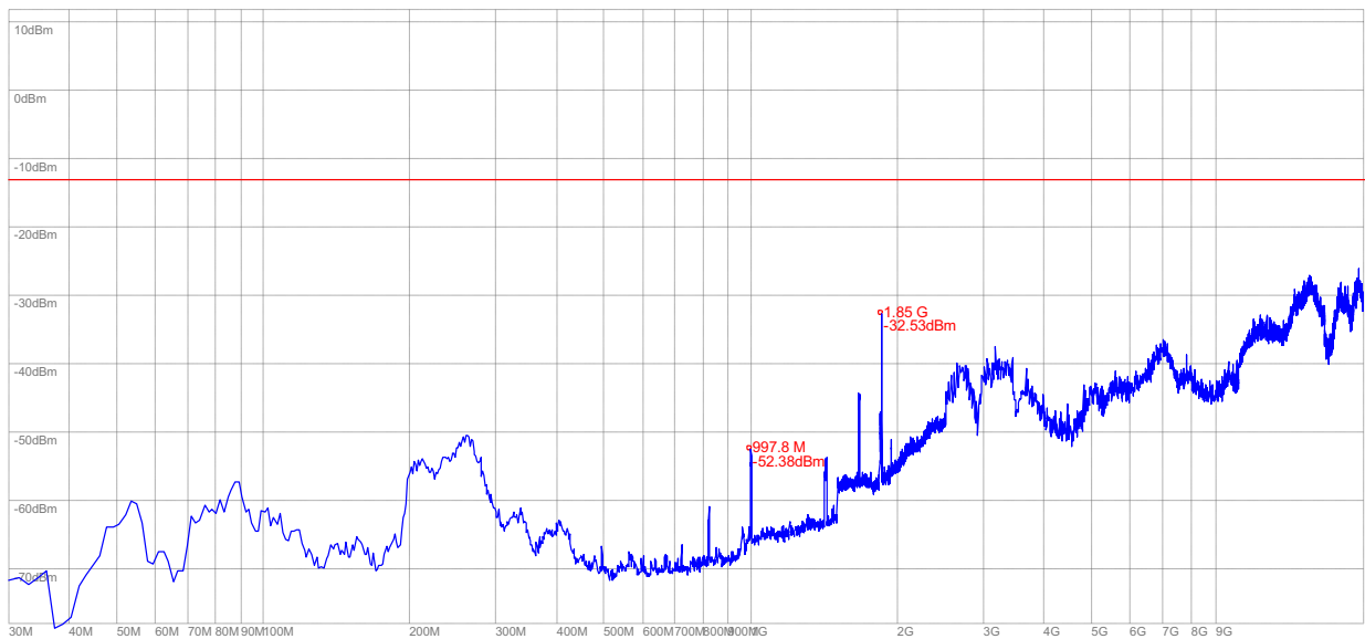
(Plot P.1: WCDMA 1900MHz Channel = 9262, Test Antenna Horizontal)
