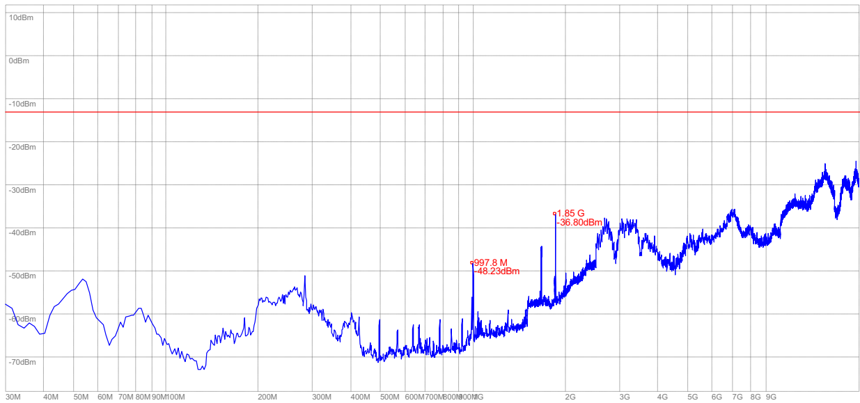
(Plot V.2: HSDPA 1900MHz Channel = 9262, Test Antenna Vertical)
