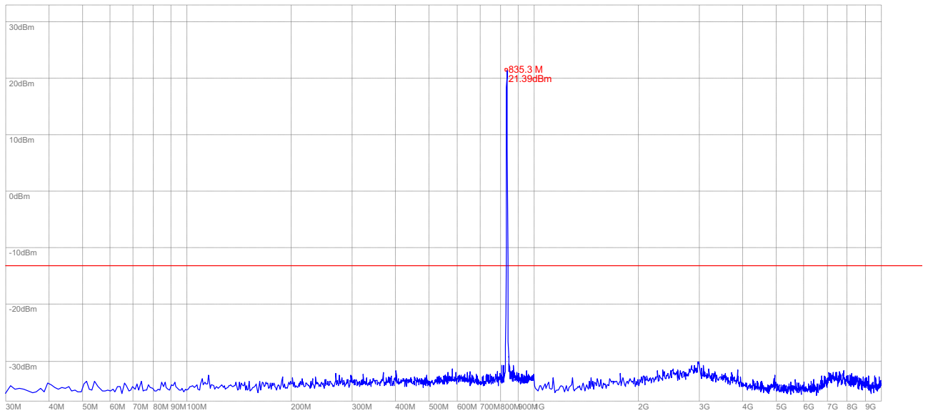
(Plot N: WCDMA 850MHz Channel = 4175, 30MHz to 10GHz)
