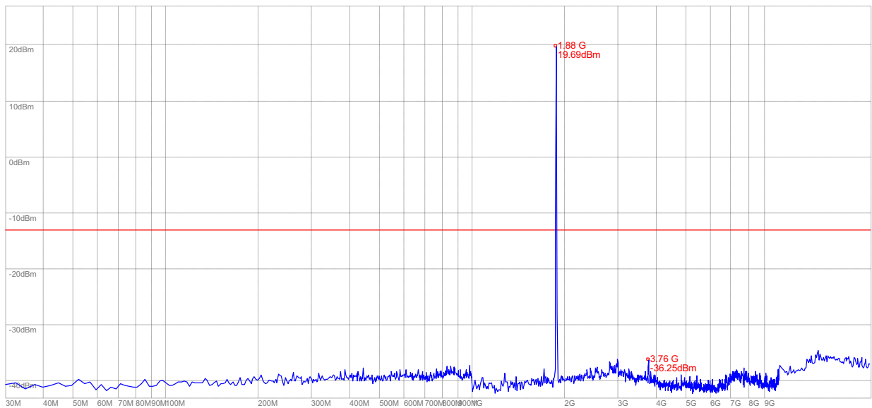
(Plot Q: WCDMA 1900MHz Channel = 9400, 30MHz to 20GHz)
