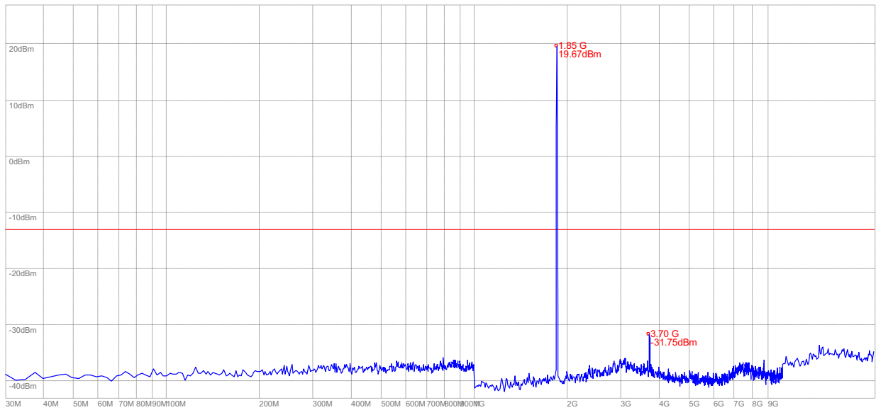
(Plot V: HSDPA 1900MHz Channel = 9262, 30MHz to 20GHz)
