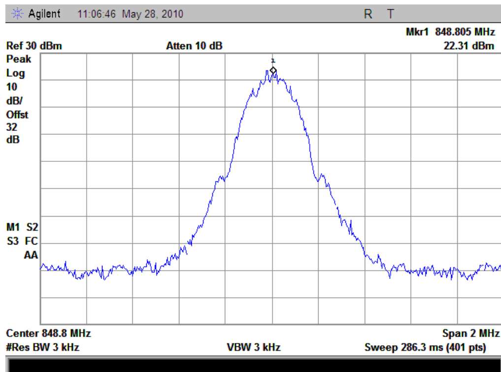
(Plot F: EDGE 850MHz Channel = 251)
