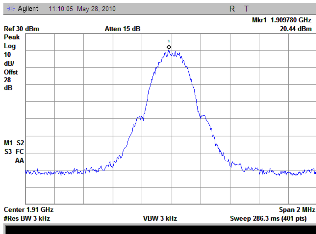
(Plot H: EDGE 1900MHz Channel = 810)
