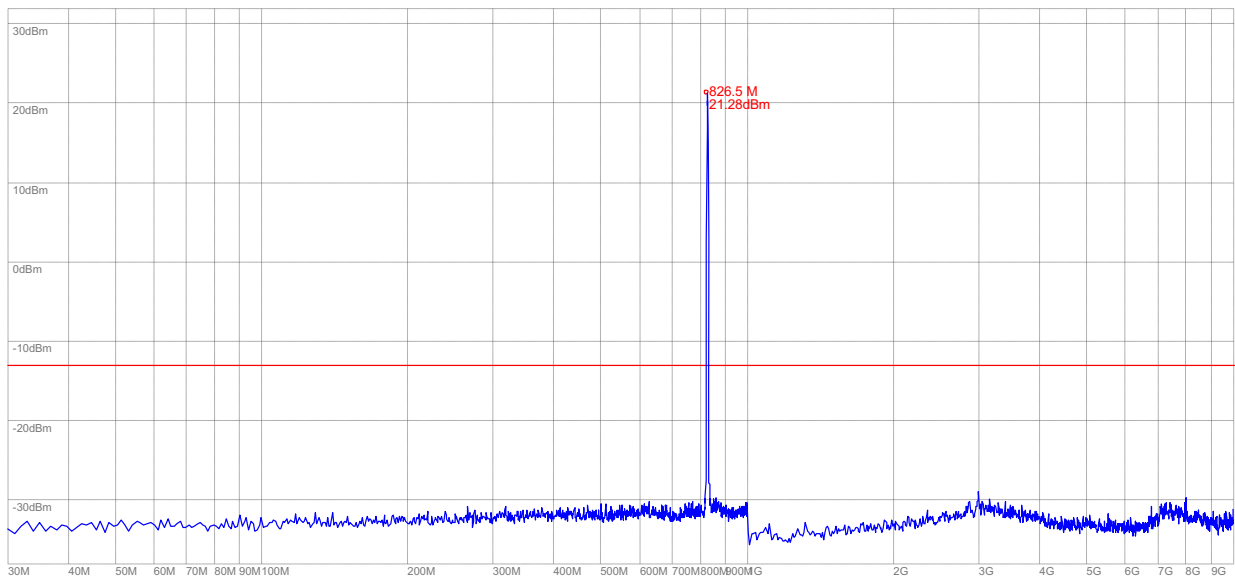
(Plot S: HSDPA 850MHz Channel = 4132, 30MHz to 10GHz)
