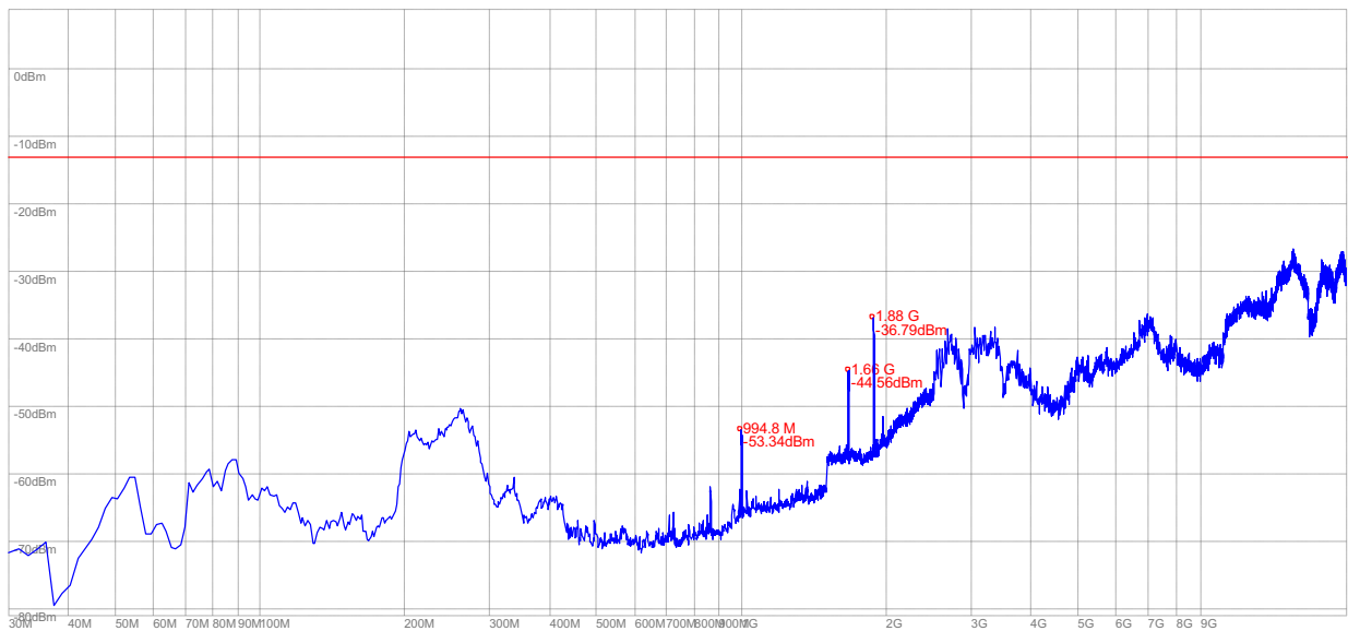
(Plot W.1: HSDPA 1900MHz Channel = 9400, Test Antenna Horizontal)
