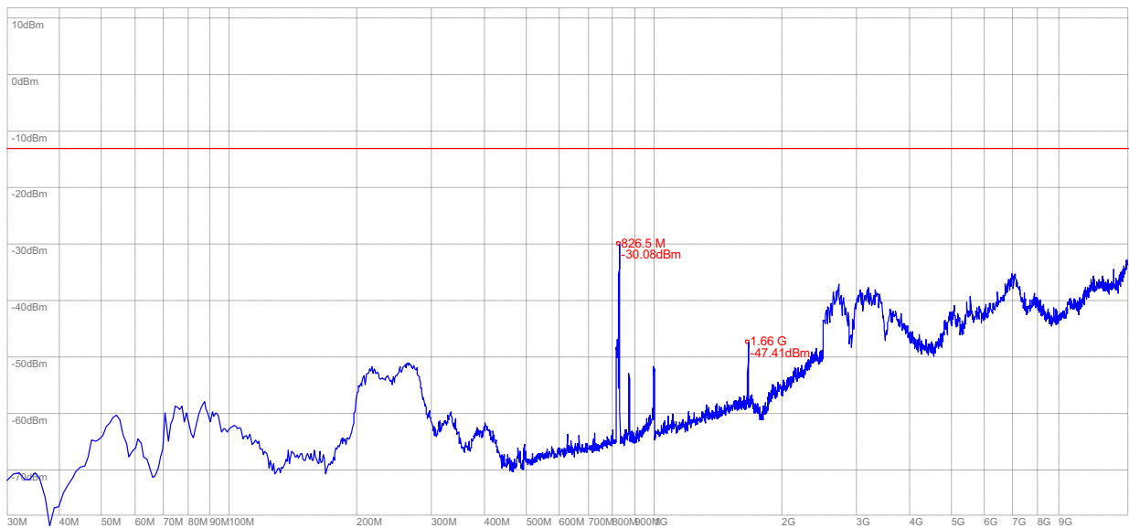
(Plot M.1: WCDMA 850MHz Channel = 4132, Test Antenna Horizontal)
