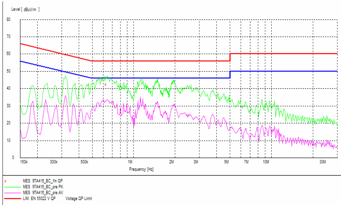
Fig. 34 AC Powerline Conducted Emission with charger
