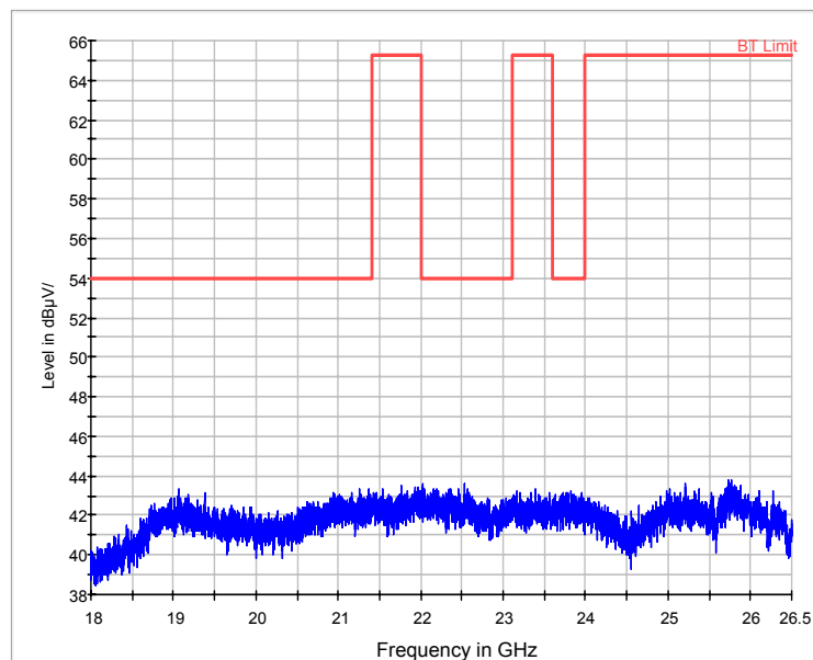
Fig.92. Radiated emission (Power): 8DPSK, high channel
