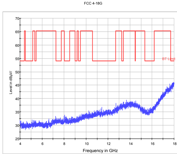
Fig.90. Radiated emission: 8DPSK, Channel 78, 4 GHz - 18 GHz
