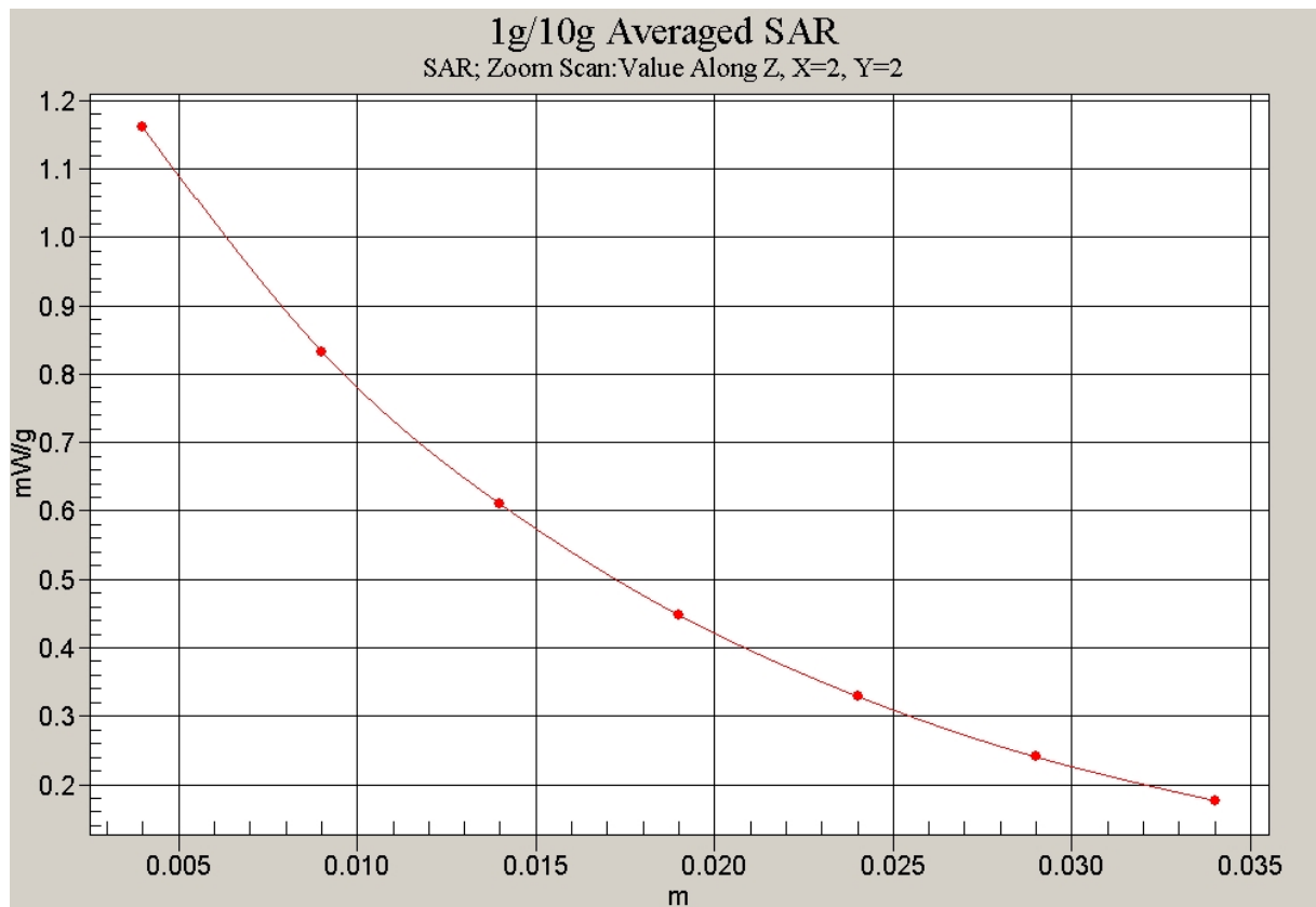
Fig. 13-2 Z-Scan at power reference point (850 MHz CH251)
