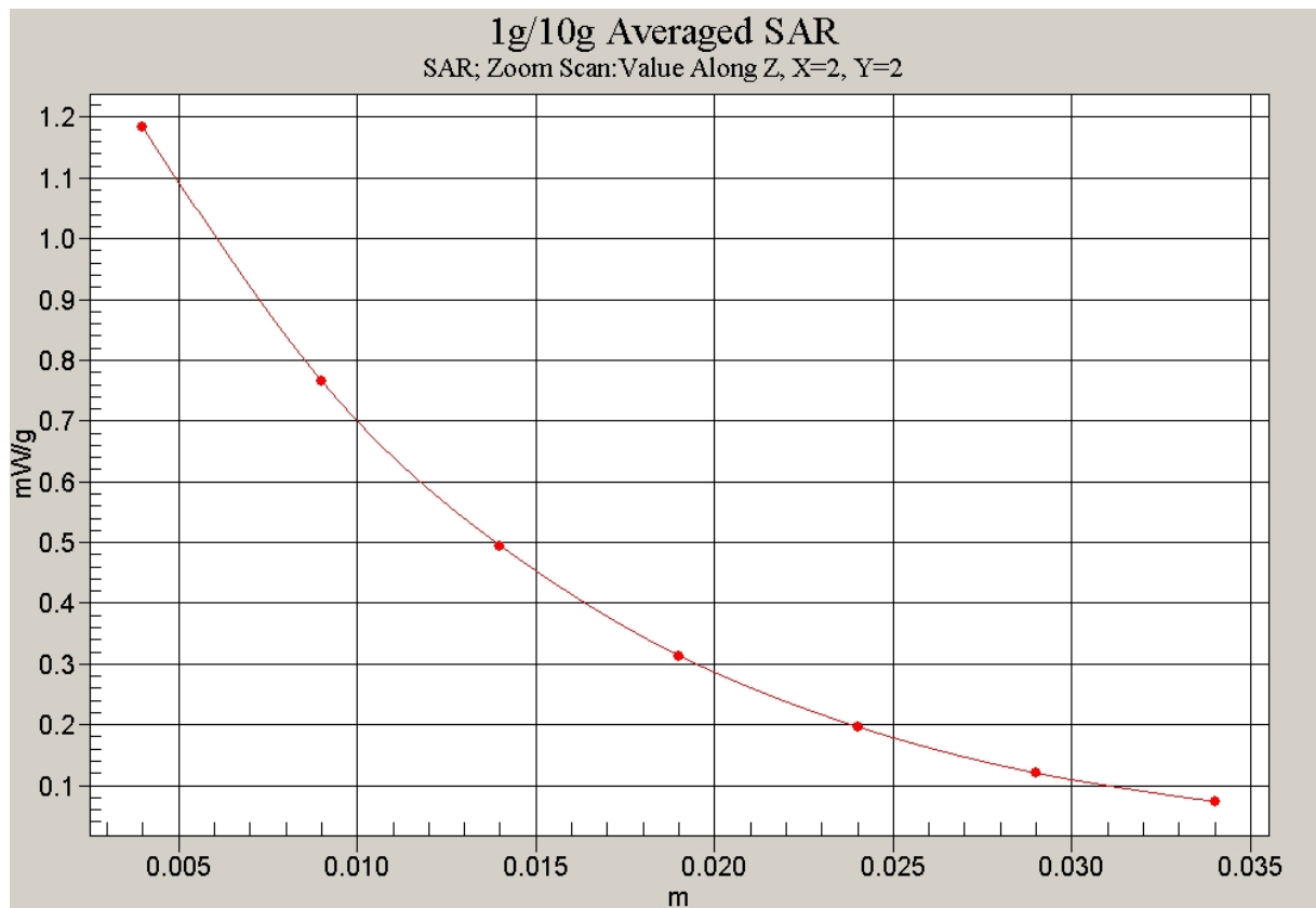
Fig. 18-2 Z-Scan at power reference point (1900 MHz CH661)
