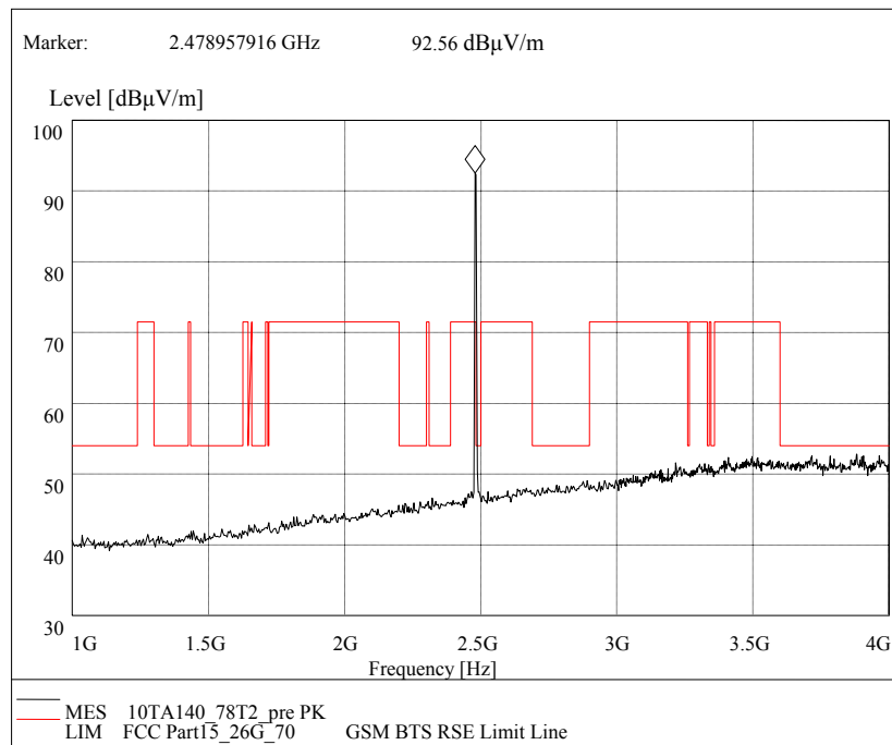
Fig. 21 Radiated emission: Channel 78, 1 GHz - 4 GHz
