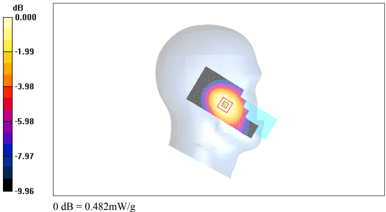
Fig.4 850 MHz CH251
