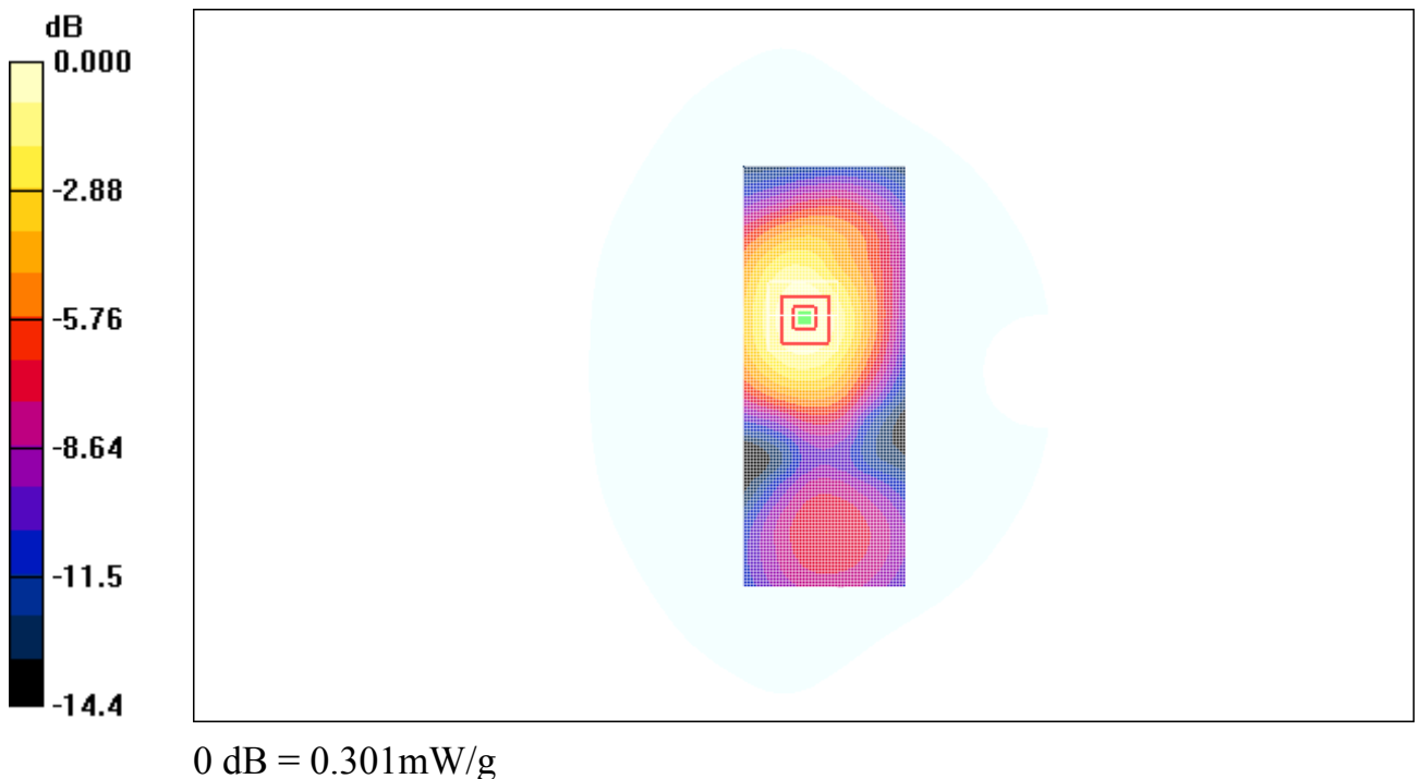
Fig. 31 1900 MHz CH512
