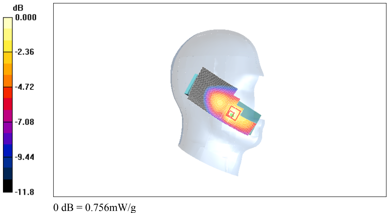
Fig. 3 850 MHz CH128
