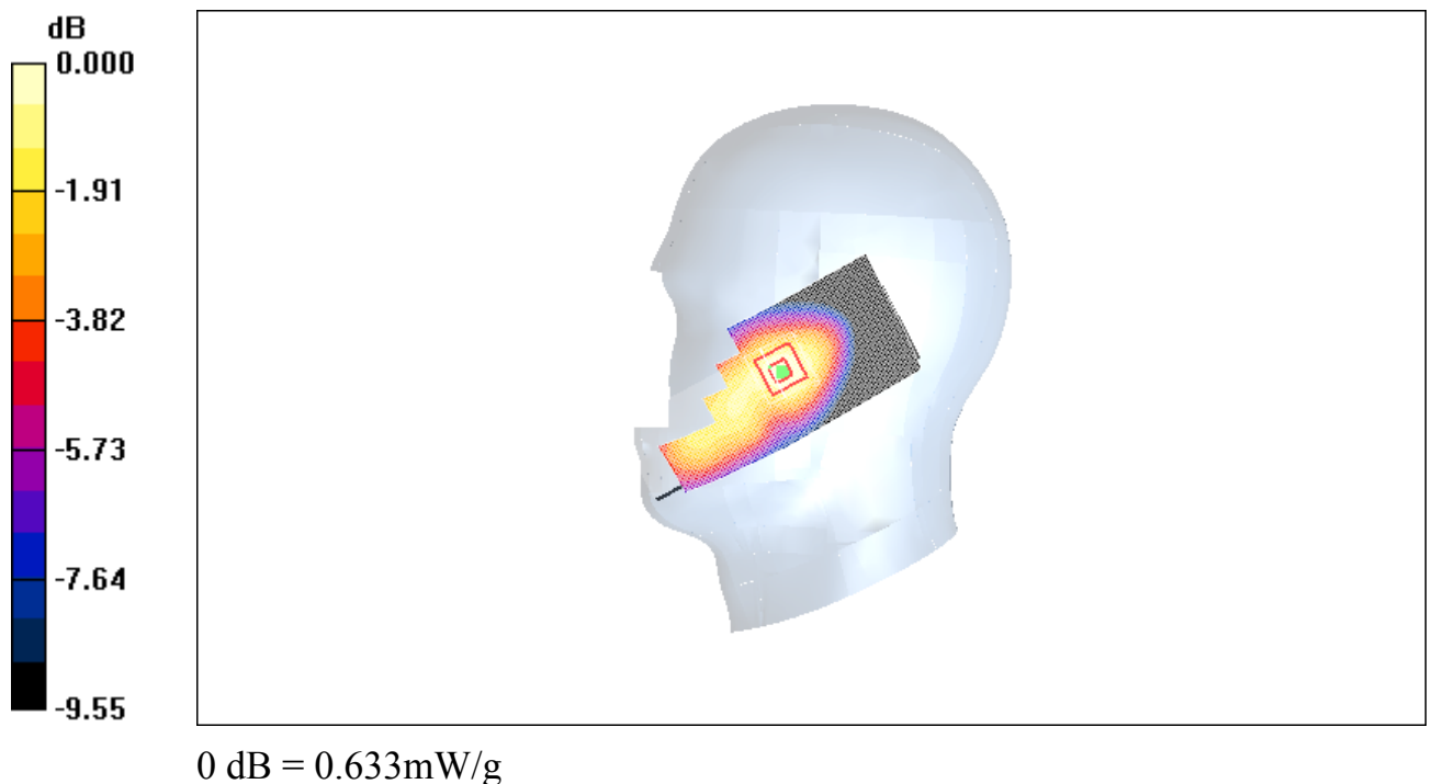
Fig. 8 850 MHz CH128
