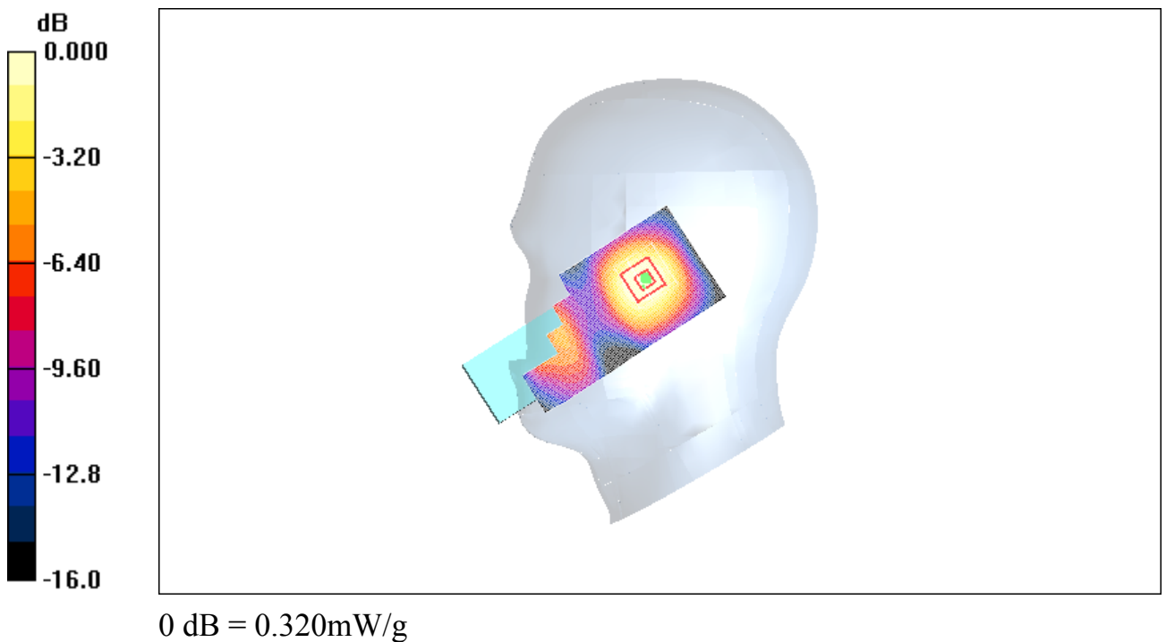
Fig.28 1900 MHz CH512
