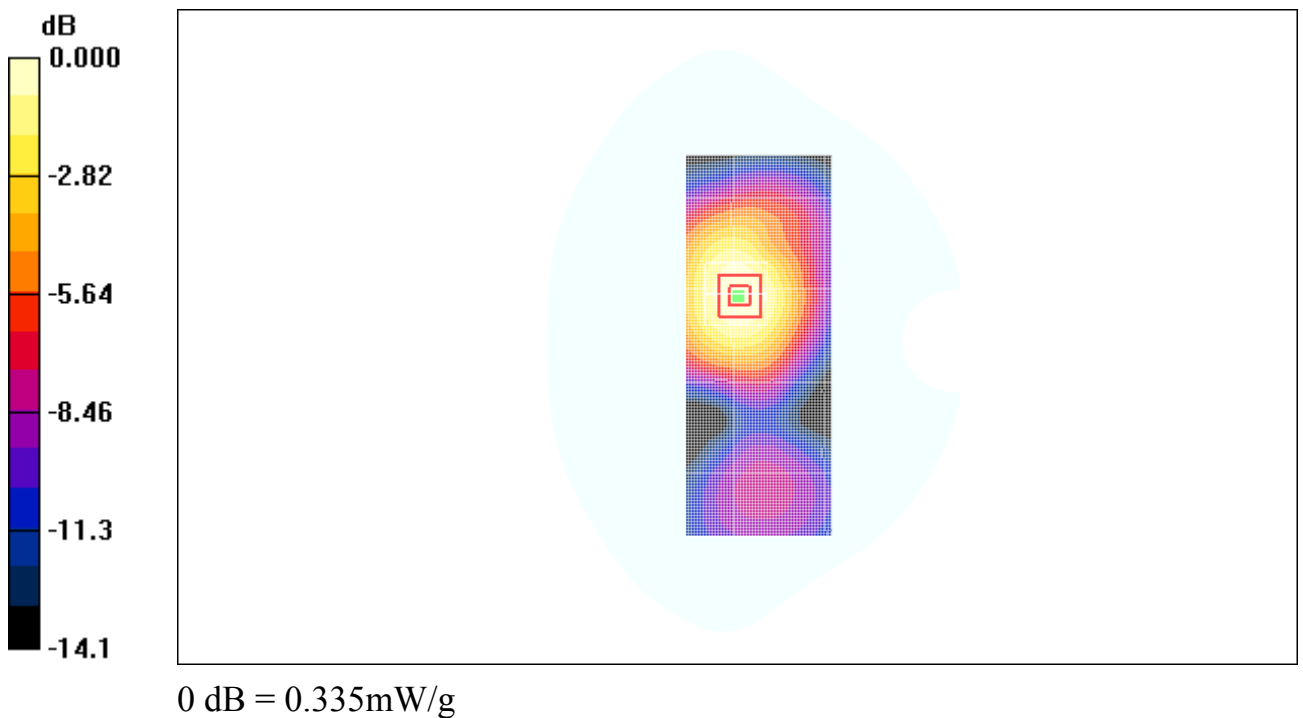
Fig. 30 1900 MHz CH661
