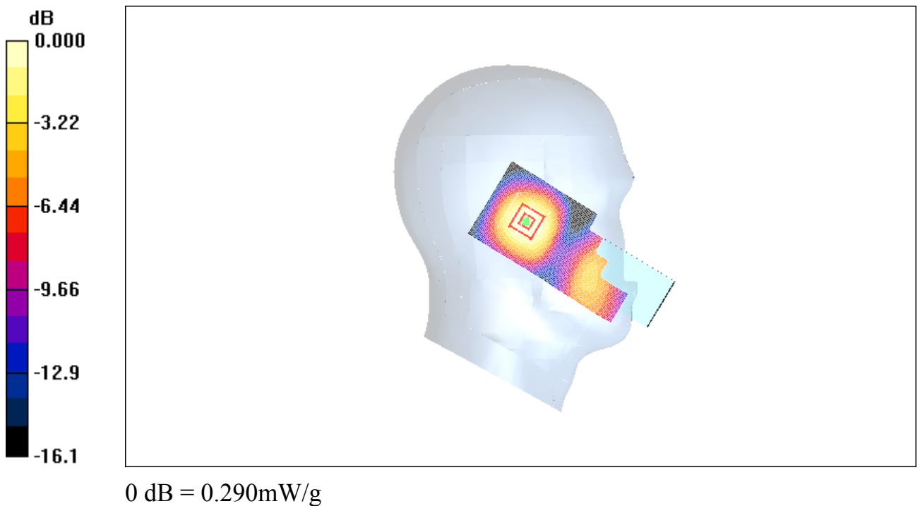
Fig. 21 1900 MHz CH661
