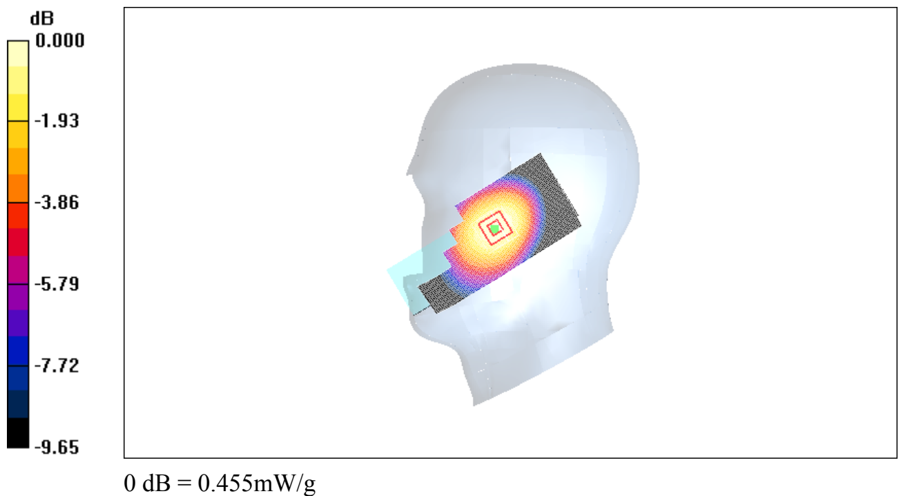
Fig.10 850 MHz CH251
