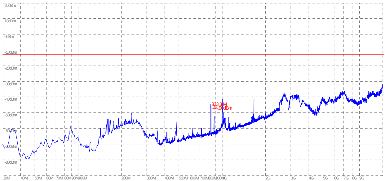
(Plot B.2: CDMA 850MHz Channel = 4175, Test Antenna Vertical)
