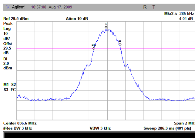
(Plot B1: GSM 850MHz Channel = 190)
