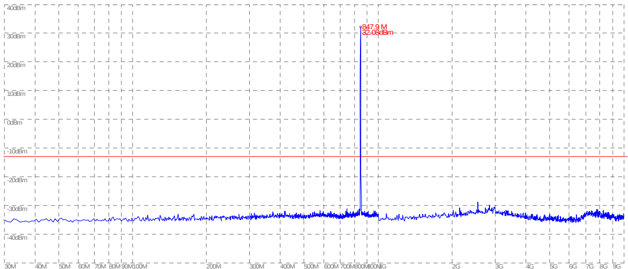
(Plot C: GSM 850MHz Channel = 251, 30MHz to 10GHz)
