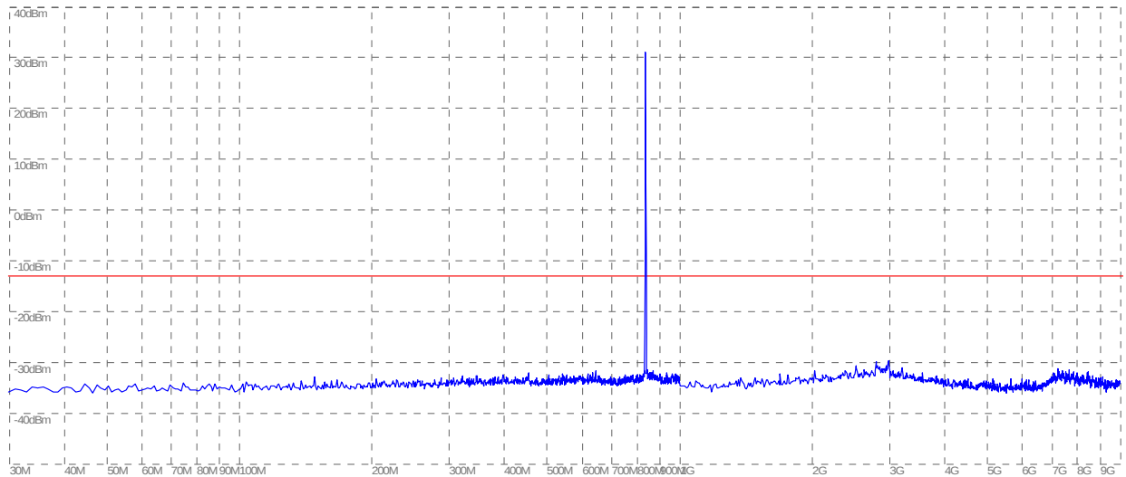
(Plot B: GSM 850MHz Channel = 190, 30MHz to 10GHz)
