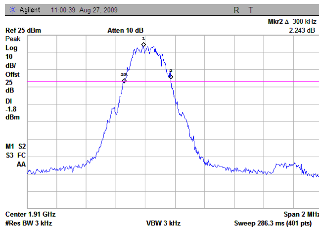
(Plot F2: EDGE 1900MHz Channel = 810)
