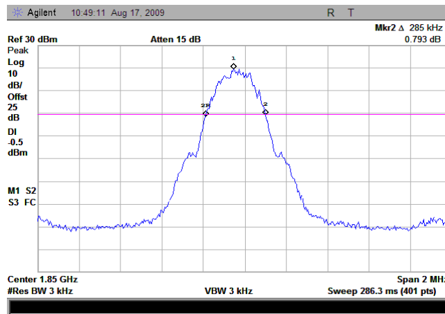
(Plot D1: GSM 1900MHz Channel = 512)
