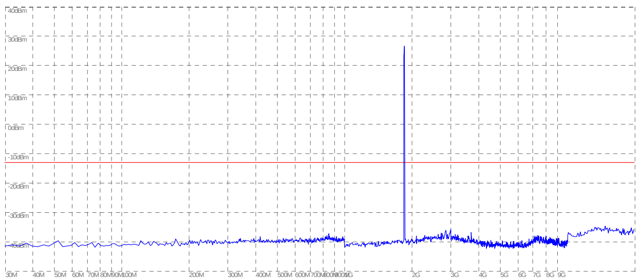
(Plot D: GSM 1900MHz Channel = 512, 30MHz to 20GHz)
