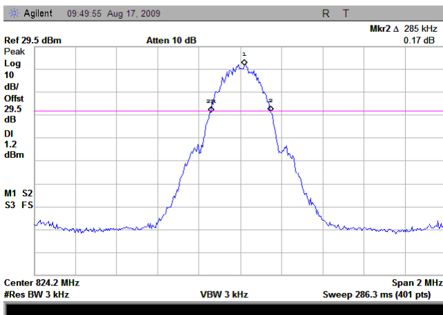
(Plot A1: GSM 850MHz Channel = 128)
