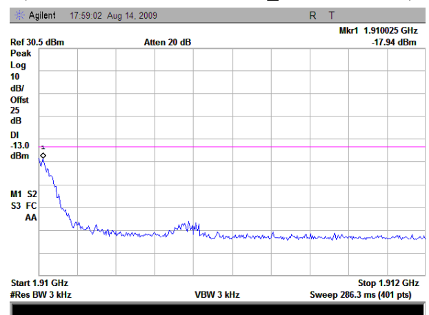
(Plot D1: GSM 1900MHz_Channel = 810)
