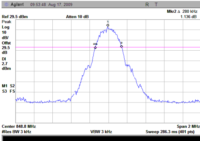
(Plot C1: GSM 850MHz Channel = 251)
