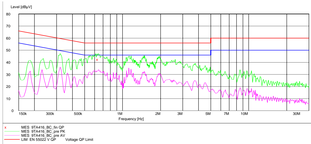
Fig. 34 AC Powerline Conducted Emission with charger 1
