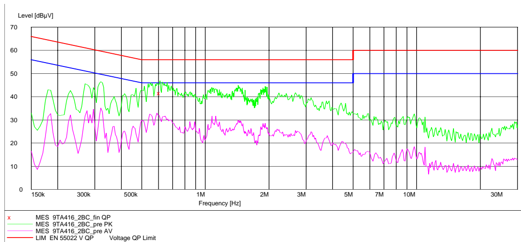
Fig. 35 AC Powerline Conducted Emission with charger 2
