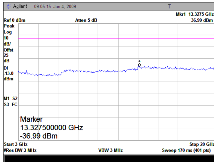
(Plot D.2: Channel = 9262, 3GHz to 20GHz)
