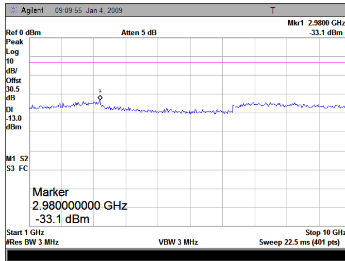
(Plot A.2: Channel = 4132, 1GHz to 10GHz)
