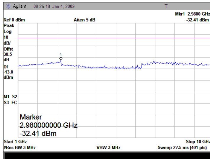
(Plot B.2: Channel = 4175, 1GHz to 10GHz)
