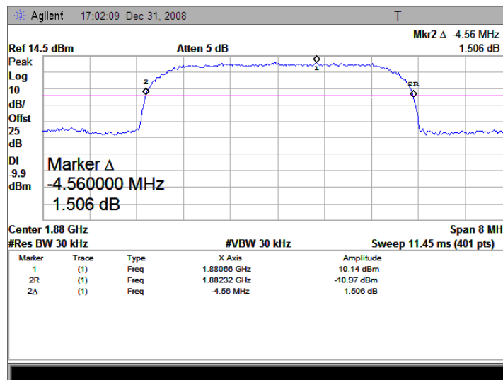
(Plot B: WCDMA 1900MHz Channel = 9400)
