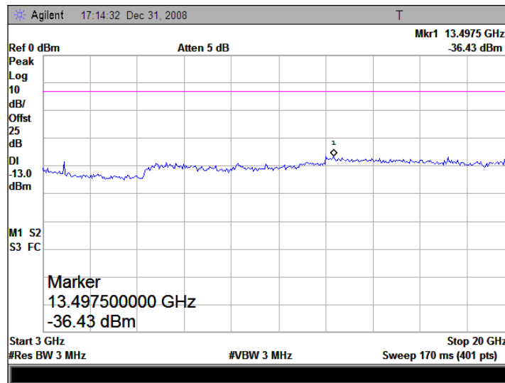
(Plot E.2: Channel = 9400, 3GHz to 20GHz)
