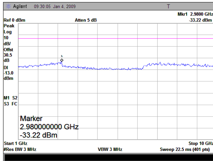
(Plot C.2: Channel = 4233, 1GHz to 10GHz)
