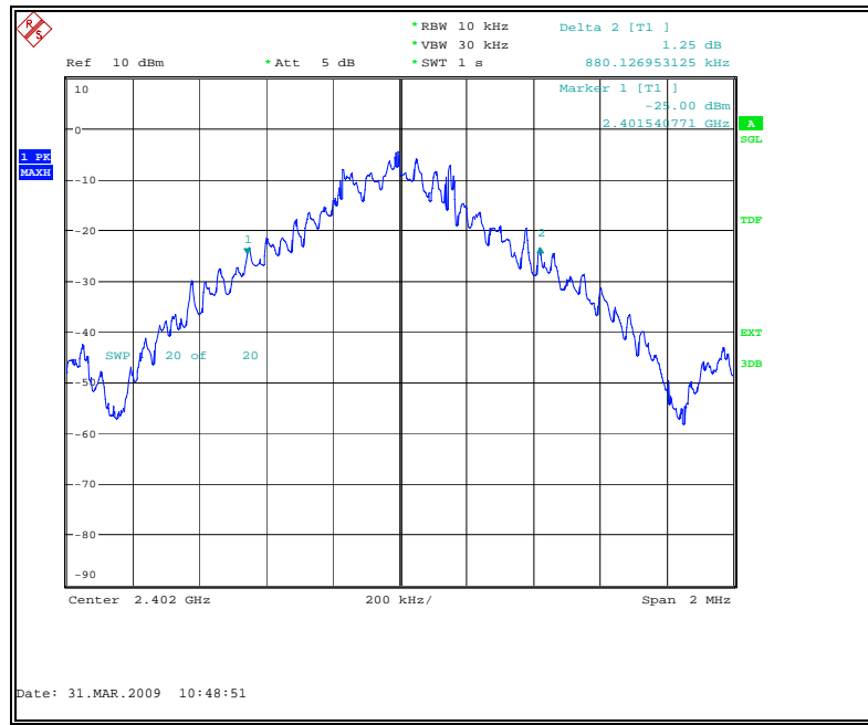
Fig. 28 20dB Bandwidth: Channel 0
