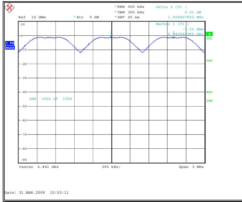
Fig. 31 Carrier frequency separation measurement: Channel 39
