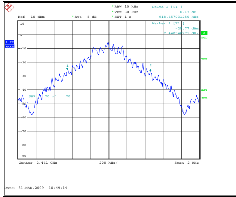
Fig. 29 20dB Bandwidth: Channel 39
