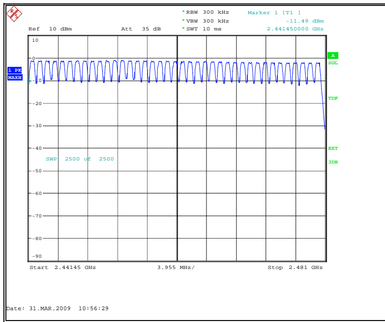
Fig. 33 Number of hopping frequencies: Channel 40 - 78
