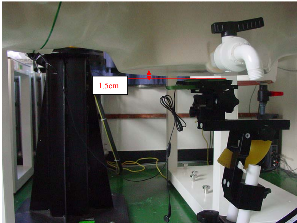
Picture G15: Body-worn Position with headset (EUT towards ground, the distance from handset to the bottom of the Phantom is 1.5cm) – Slide up
