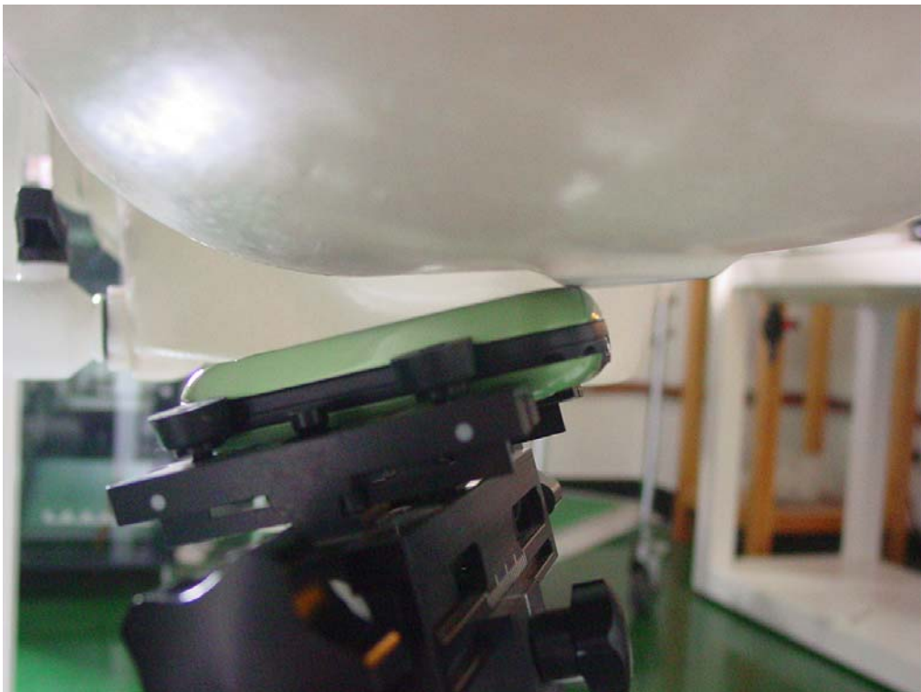
Picture G3: Left Hand Tilt 15° Position – Slide down
