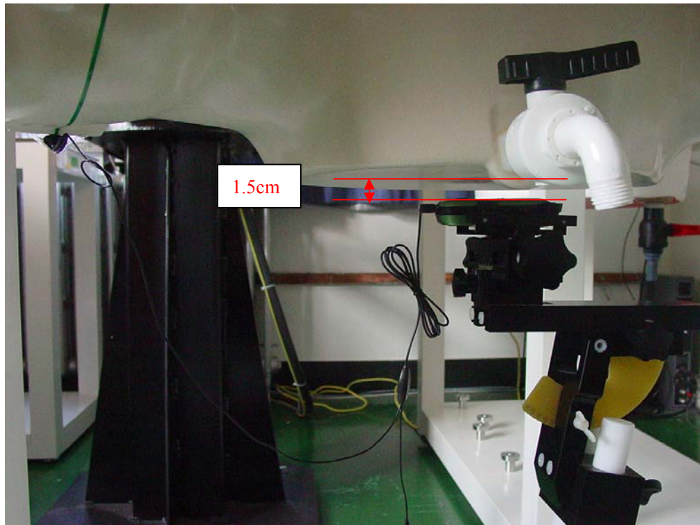
Picture G14: Body-worn Position with headset (EUT towards ground, the distance from handset to the bottom of the Phantom is 1.5cm) – Slide down
