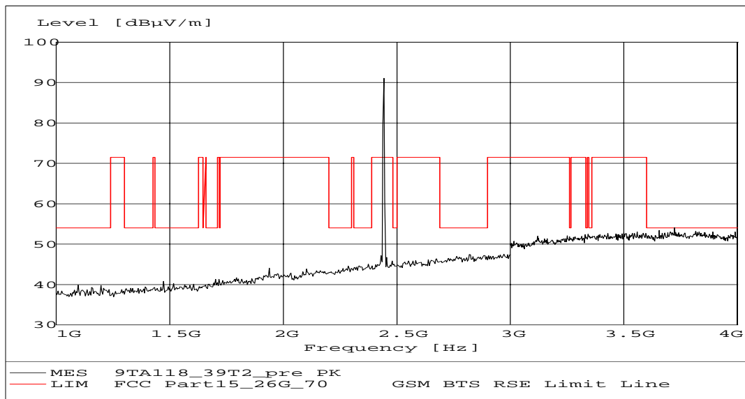
Fig. 18 Radiated emission: Channel 39, 1 GHz ~ 4 GHz
