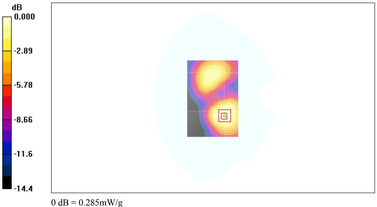
Fig. 42 1900 MHz CH512
