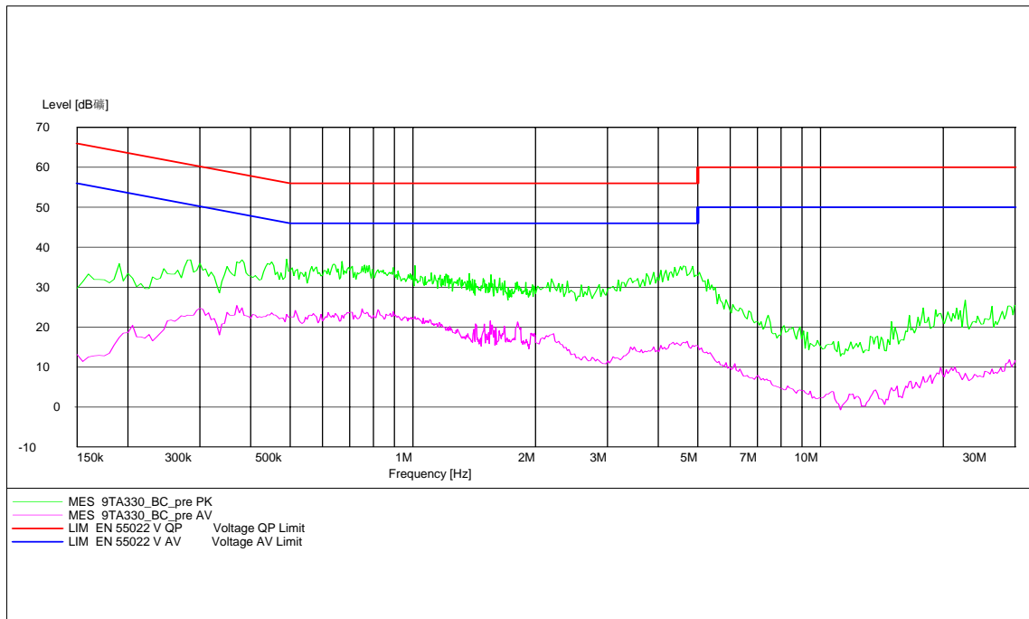
Fig. 35 AC Powerline Conducted Emission
