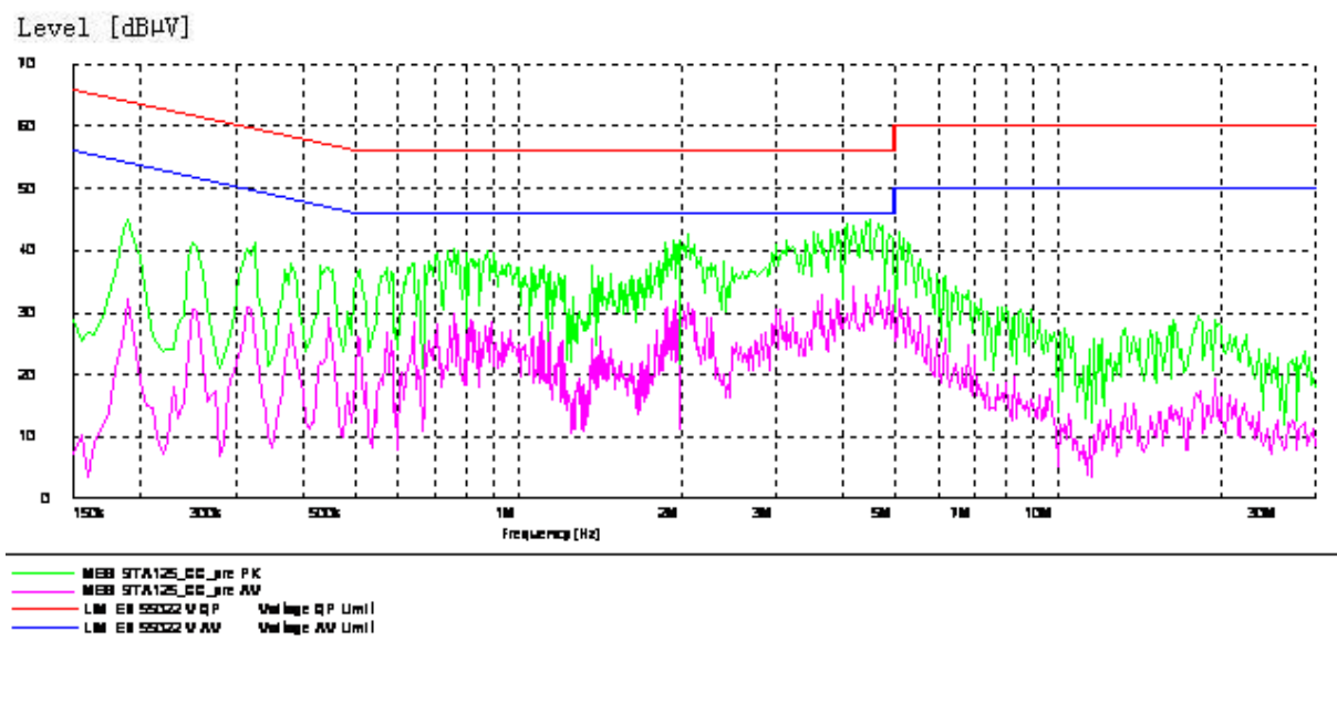
Conducted Continuous Emission (Set.1 : Camera)
