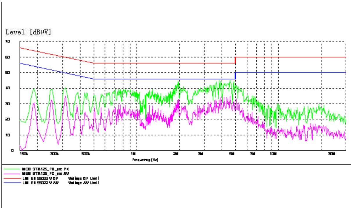
Conducted Continuous Emission (Set.1 : PCS 1900 MHz)
