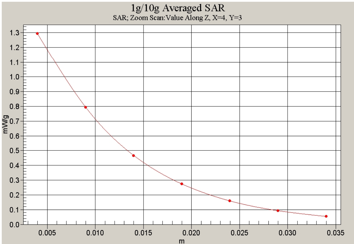
Fig. 22 Z-Scan at power reference point (1900 MHz CH512)
