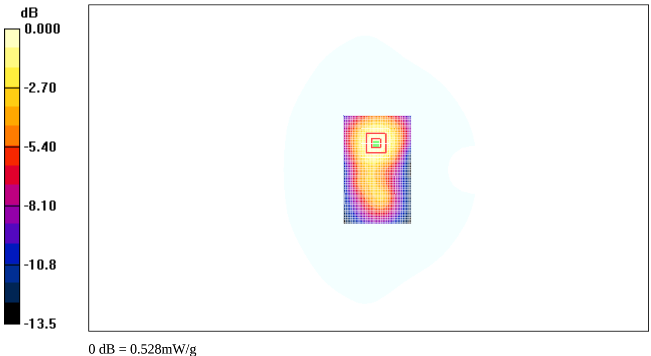
Fig. 77 1900 MHz CH512
