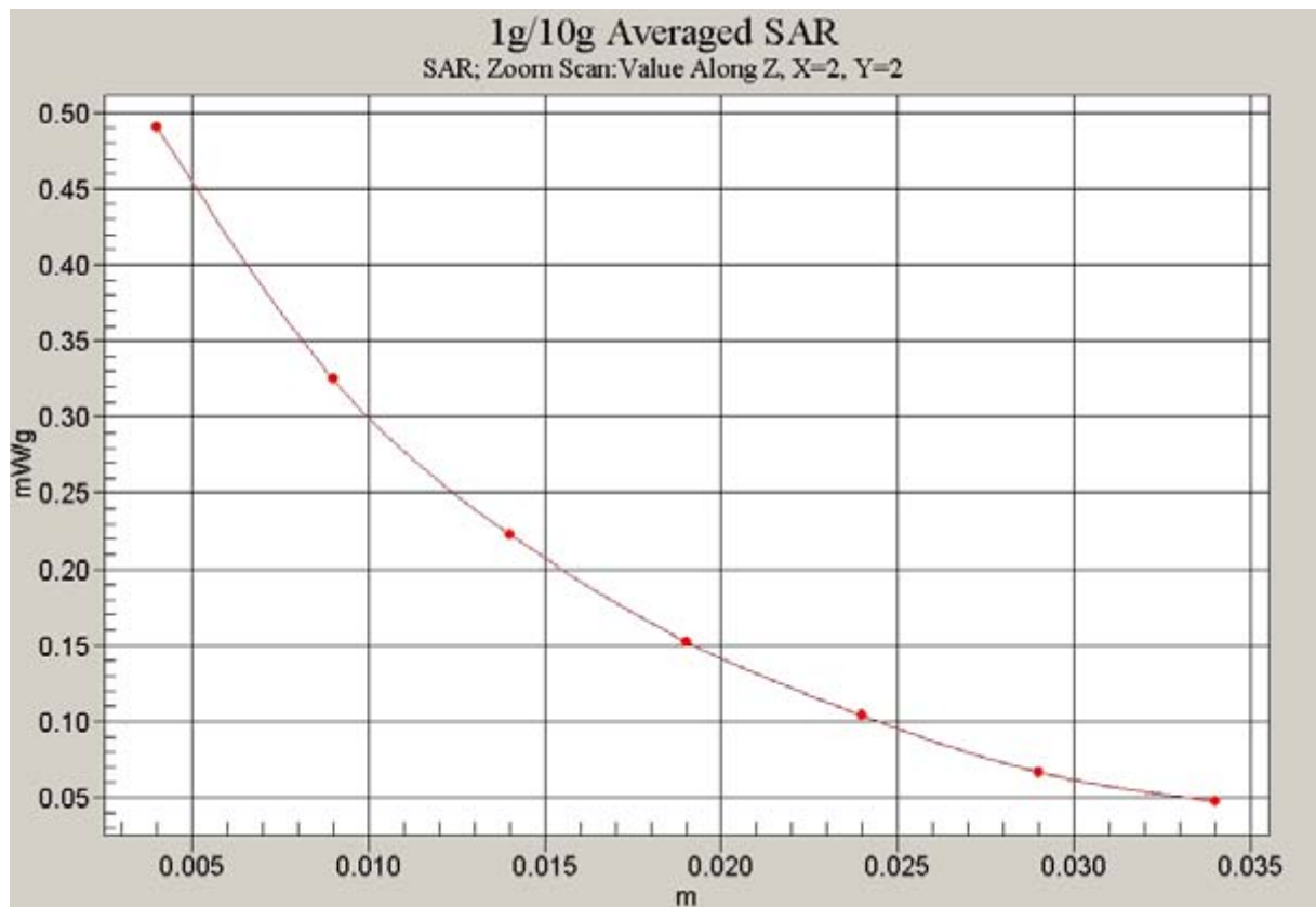
Fig. 66 Z-Scan at power reference point (1900 MHz CH810)
