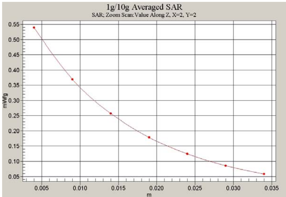
Fig. 80 Z-Scan at power reference point (1900 MHz CH512)
