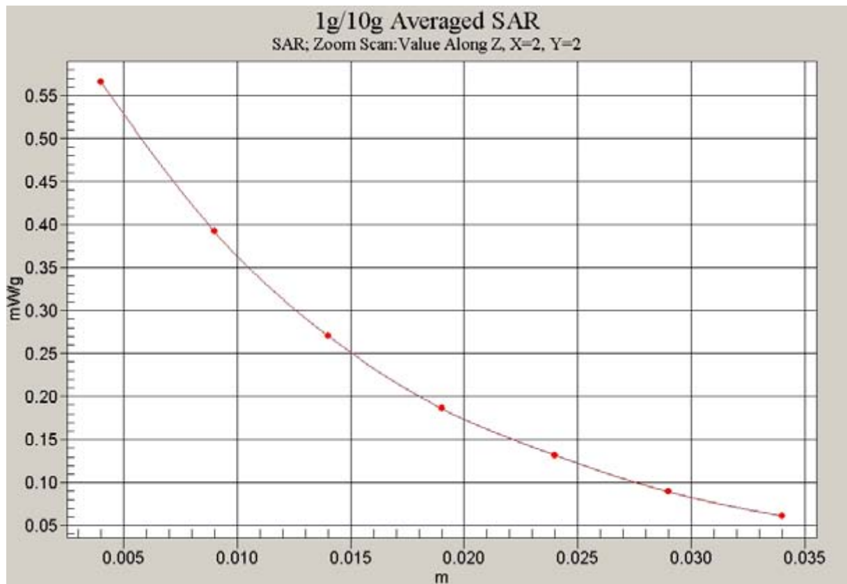
Fig. 70 Z-Scan at power reference point (1900 MHz CH512)
