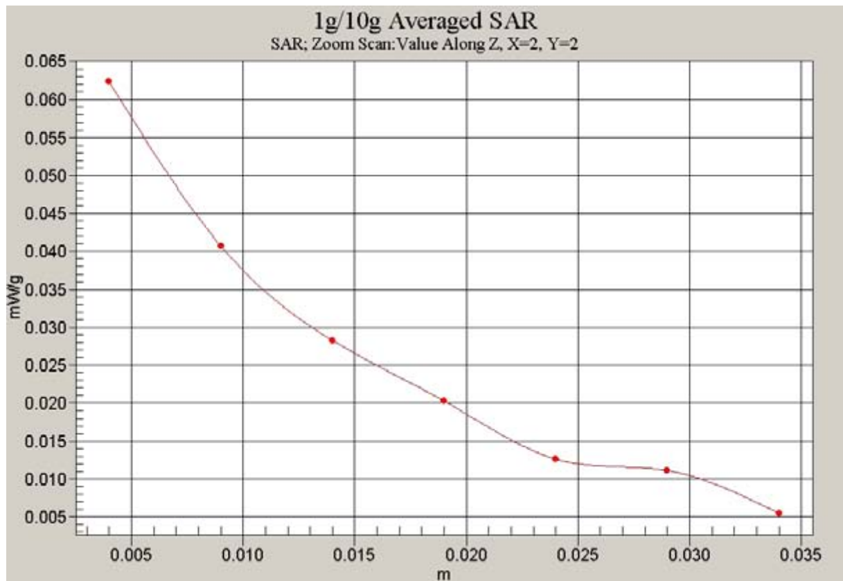
Fig.72 Z-Scan at power reference point (1900 MHz CH810)
