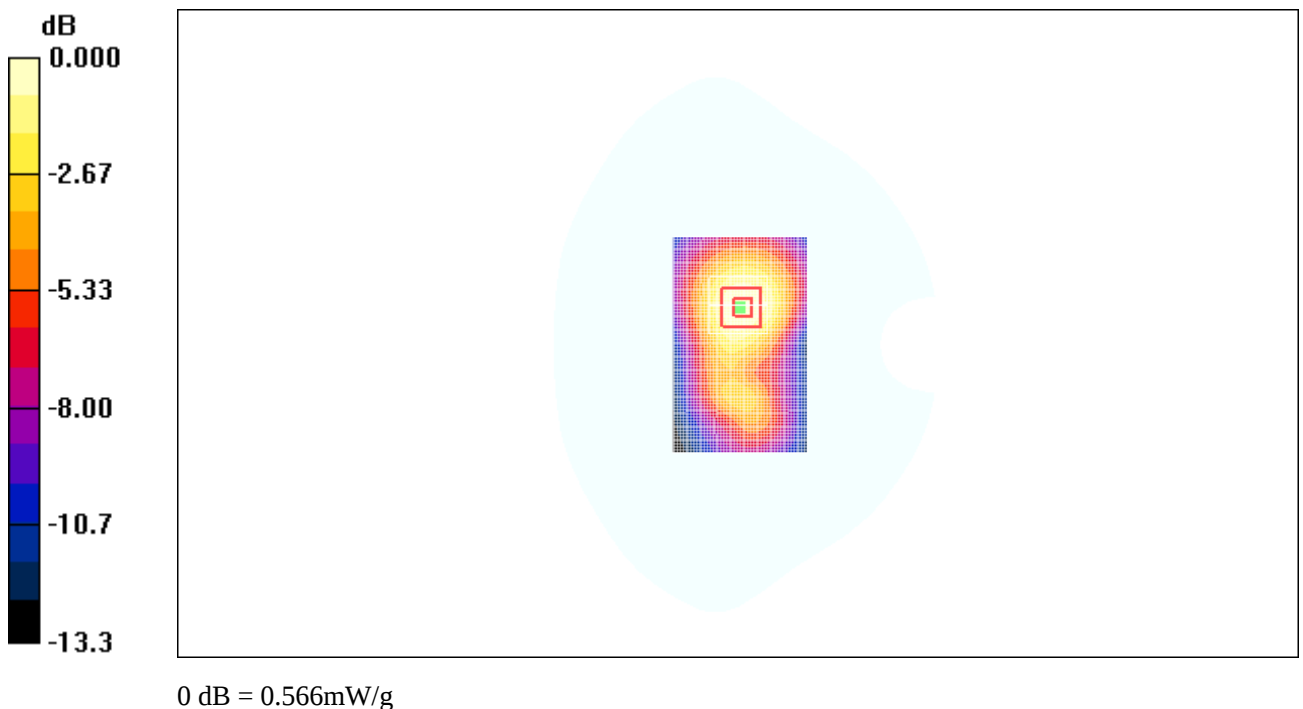
Fig. 69 1900 MHz CH512
