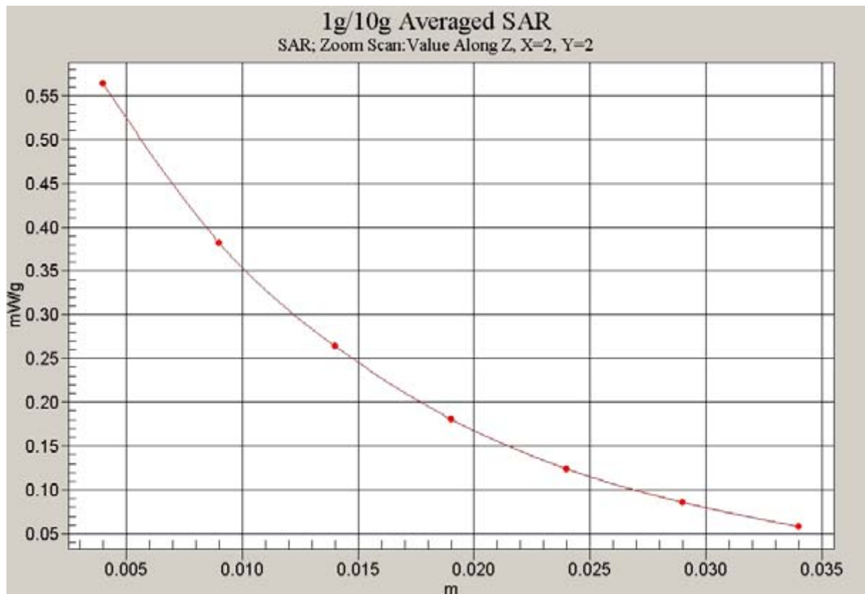
Fig. 68 Z-Scan at power reference point (1900 MHz CH661)
