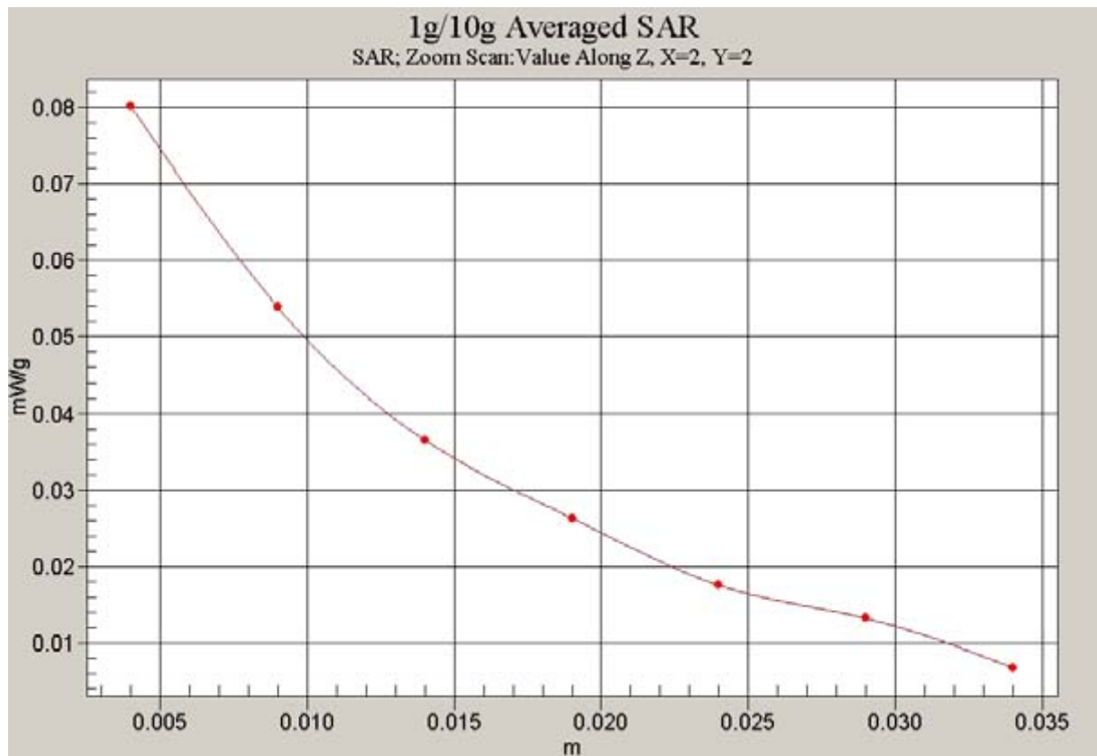
Fig. 74 Z-Scan at power reference point (1900 MHz CH661)
