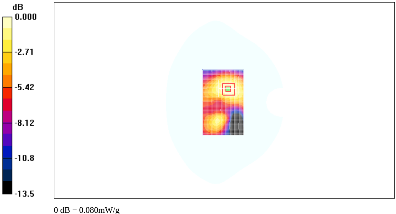
Fig. 73 1900 MHz CH661
