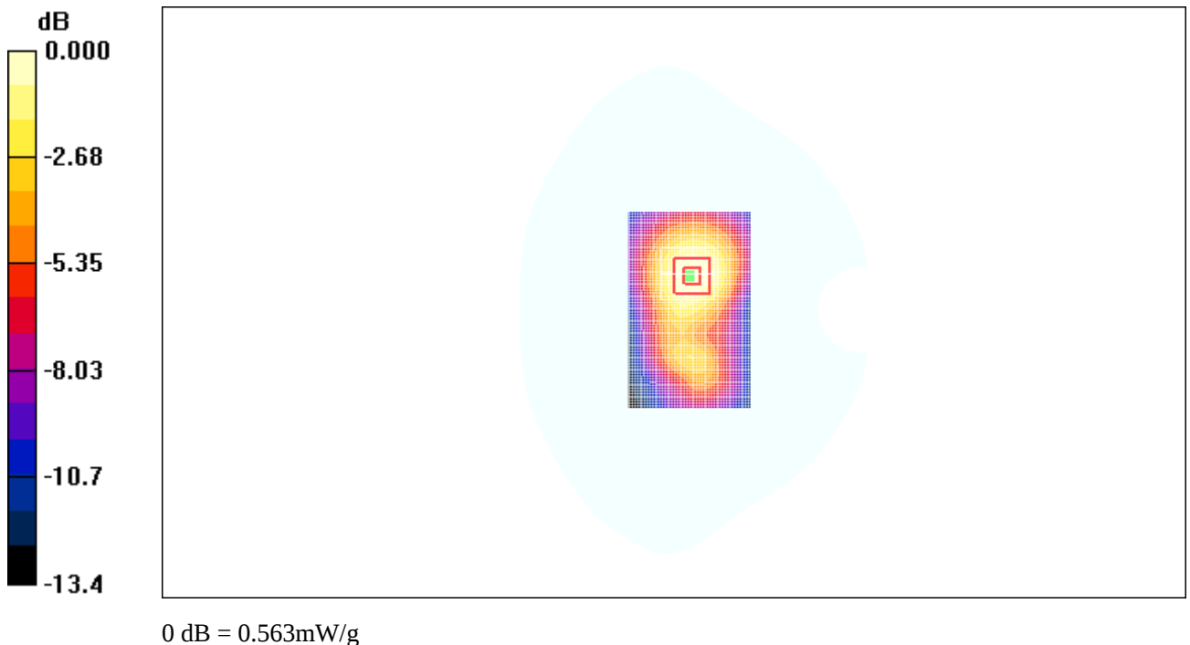
Fig. 67 1900 MHz CH661
