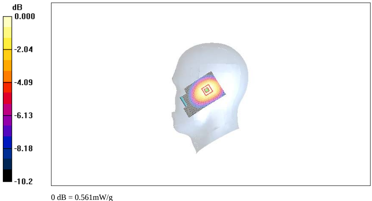
Fig.19 850 MHz CH251
