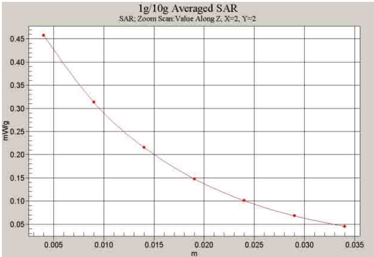
Fig. 78 Z-Scan at power reference point (1900 MHz CH661)
