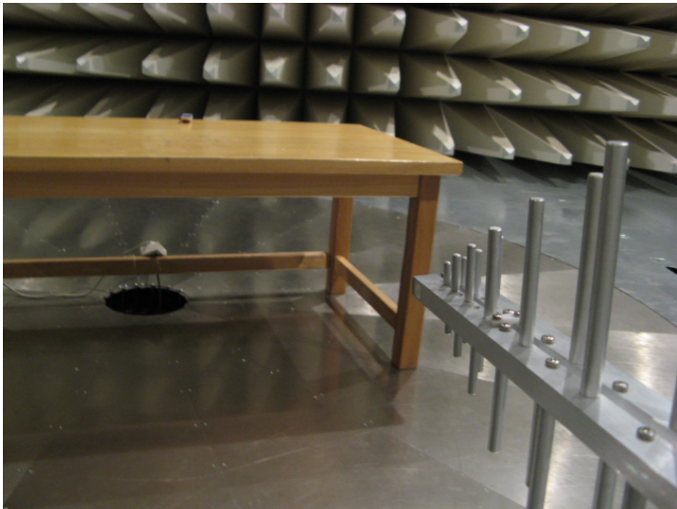
Pic 6 Radiated Spurious Emission (Part 15C)
