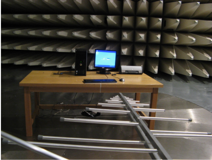
Pic 5 Radiated Spurious Emission (USB Mode)
