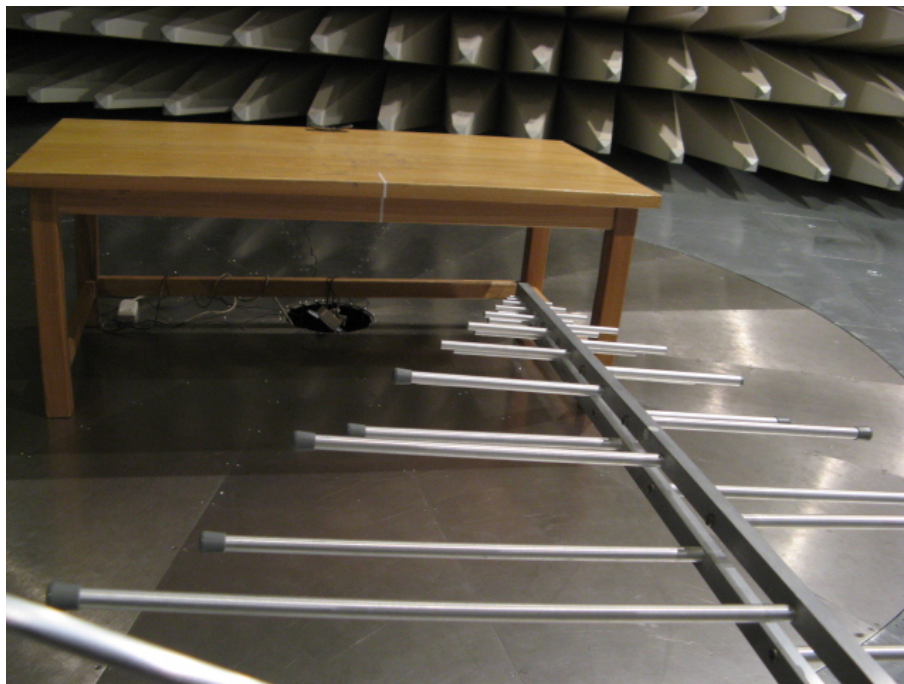
Pic 4 Radiated Spurious Emission (Charging Mode)
