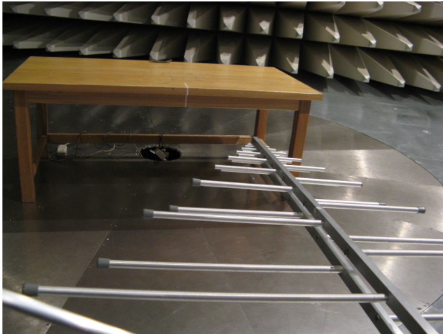
Pic C-3 Radiated Spurious Emission (Charging Mode)
