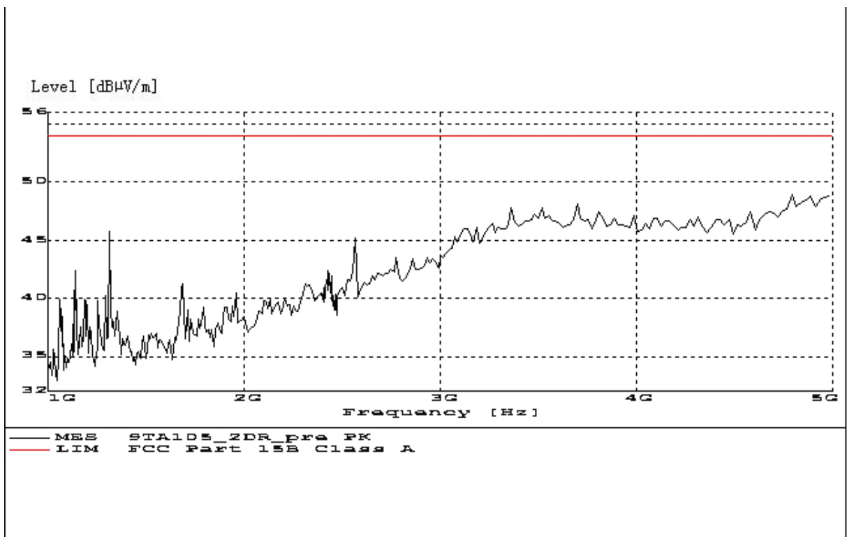
Figure B.4 Radiated Emission from 1GHz to 5GHz
