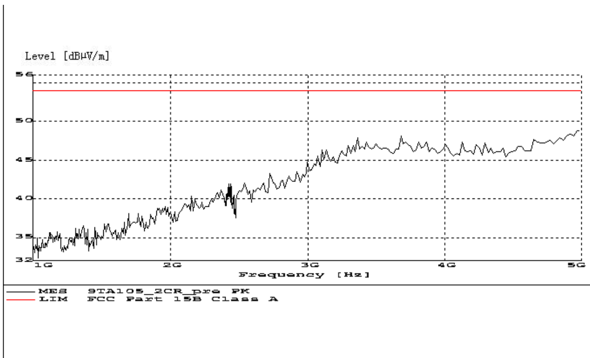
Figure B.2 Radiated Emission from 1GHz to 5GHz
