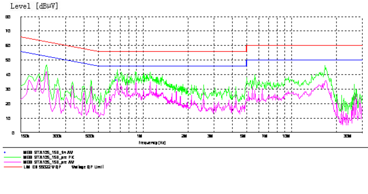
Figure B.6 Conducted Emission
