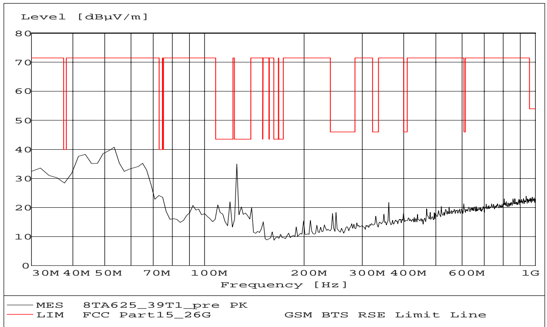
Fig. 18 Radiated emission: Channel 39, 30 MHz ~ 1 GHz
