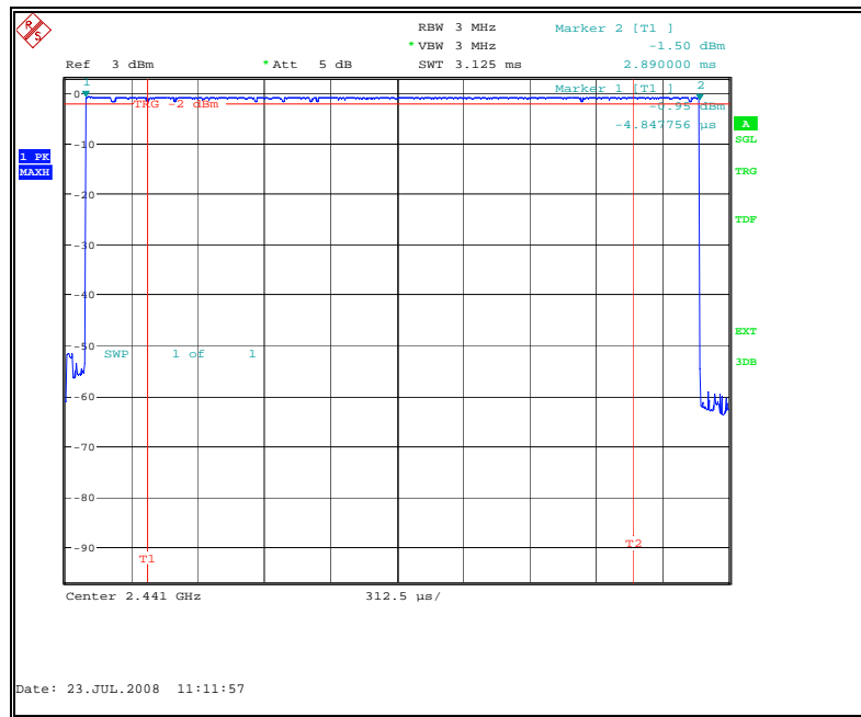
Fig. 26 Time of occupancy (Dwell Time): Channel 39
