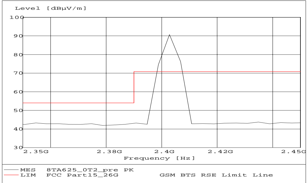
Fig. 17 Radiated emission: Channel 0, 2.35 GHz ~ 2.45 GHz
