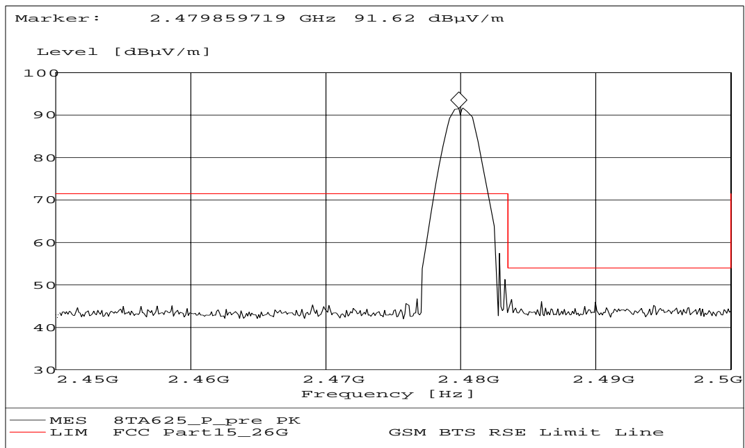
Fig. 24 Radiated emission: Channel 78, 2.45GHz ~ 2.5GHz
