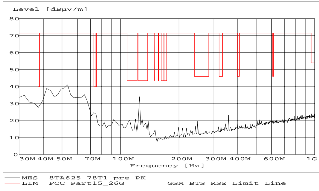
Fig. 21 Radiated emission: Channel 78, 30 MHz ~ 1 GHz
