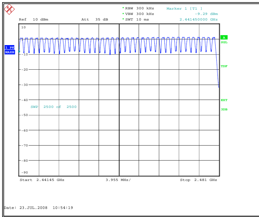
Fig. 32 Number of hopping frequencies: Channel 40 - 78
