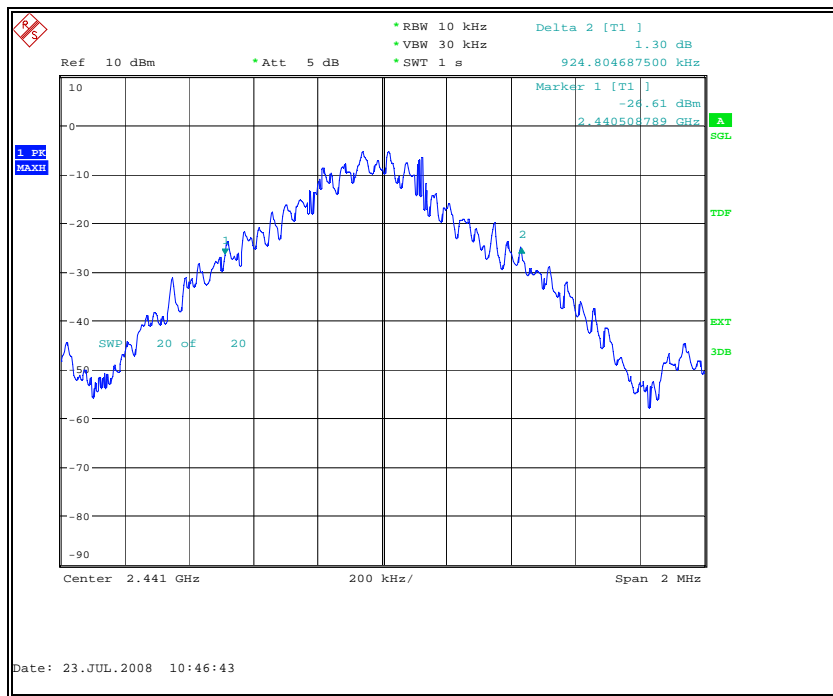
Fig. 28 20dB Bandwidth: Channel 39
