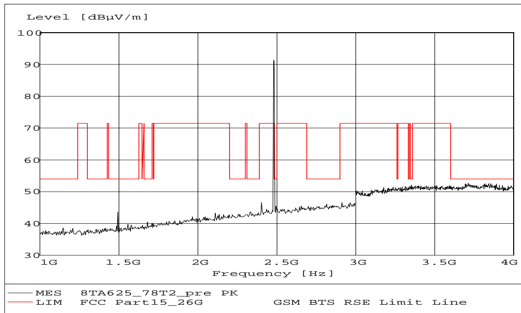
Fig. 22 Radiated emission: Channel 78, 1 GHz ~ 4 GHz
