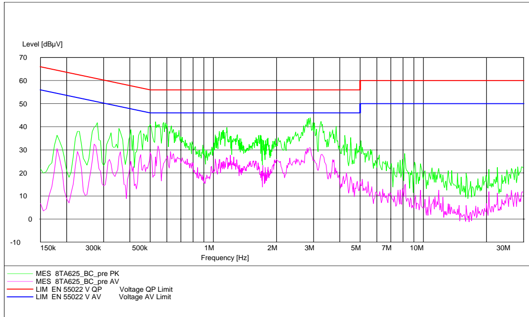
Fig. 33 AC Powerline Conducted Emission
