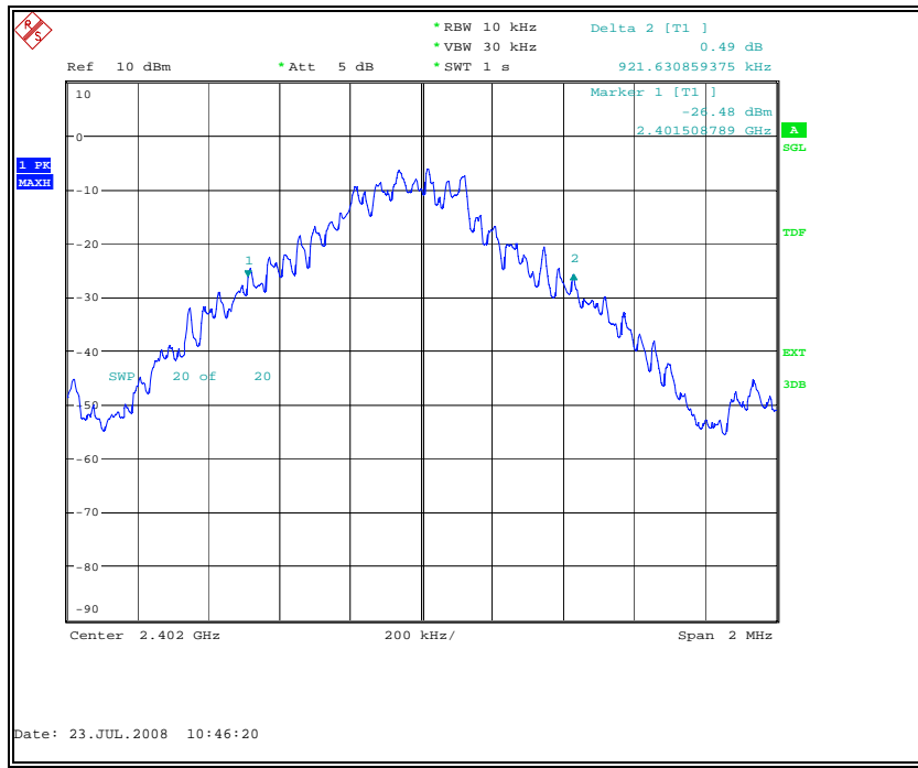
Fig. 27 20dB Bandwidth: Channel 0
