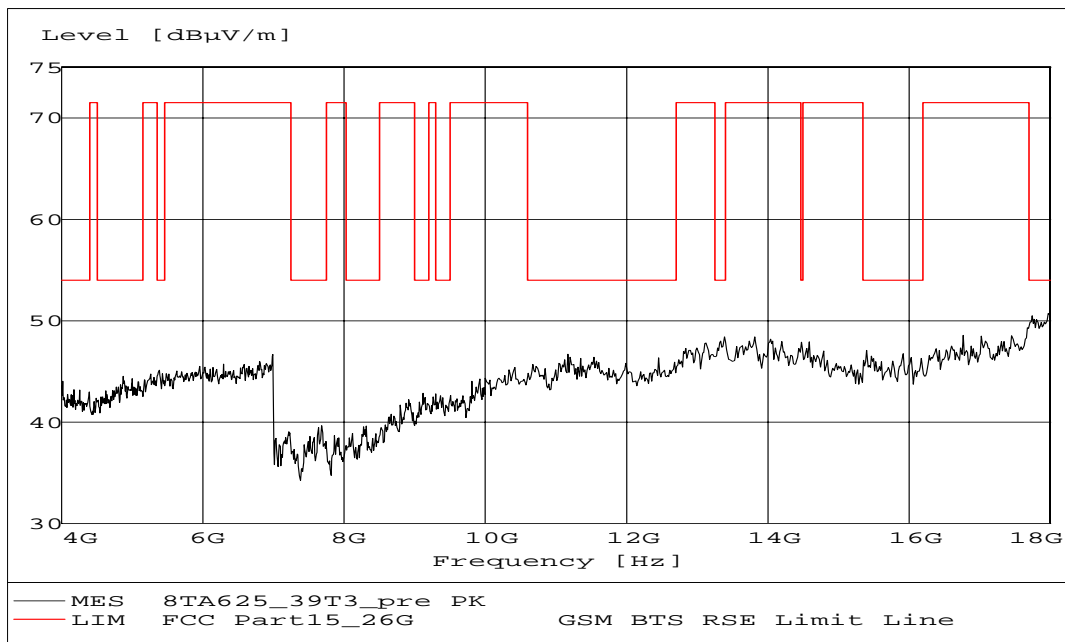
Fig. 20 Radiated emission: Channel 39, 4 GHz ~ 18 GHz
