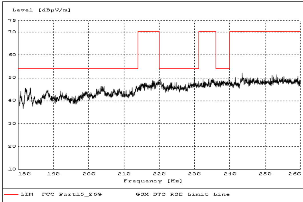
Fig. 25 Radiated emission: 18 GHz ~ 26 GHz
