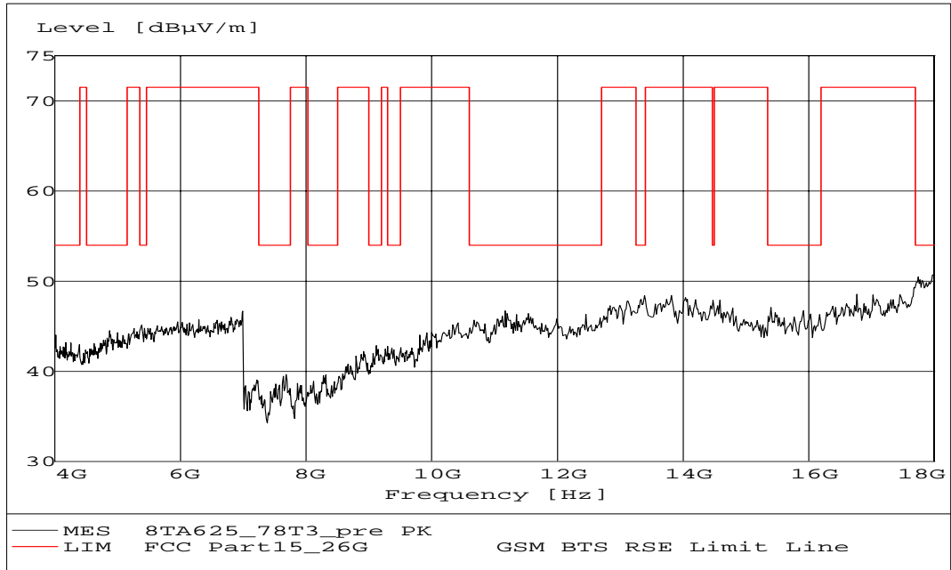
Fig. 23 Radiated emission: Channel 78, 4 GHz ~ 18 GHz
