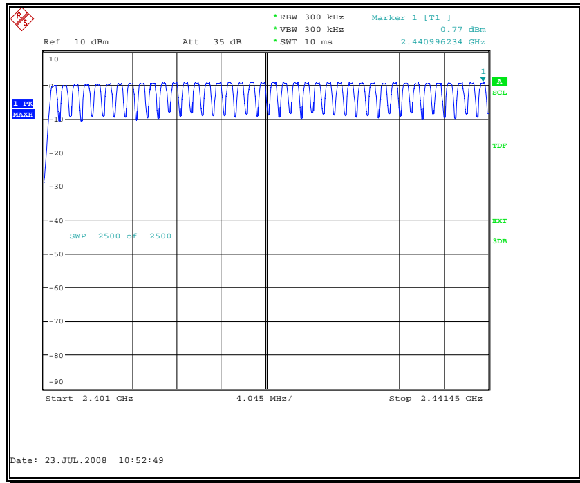
Fig. 31 Number of hopping frequencies: Channel 0 – 39
