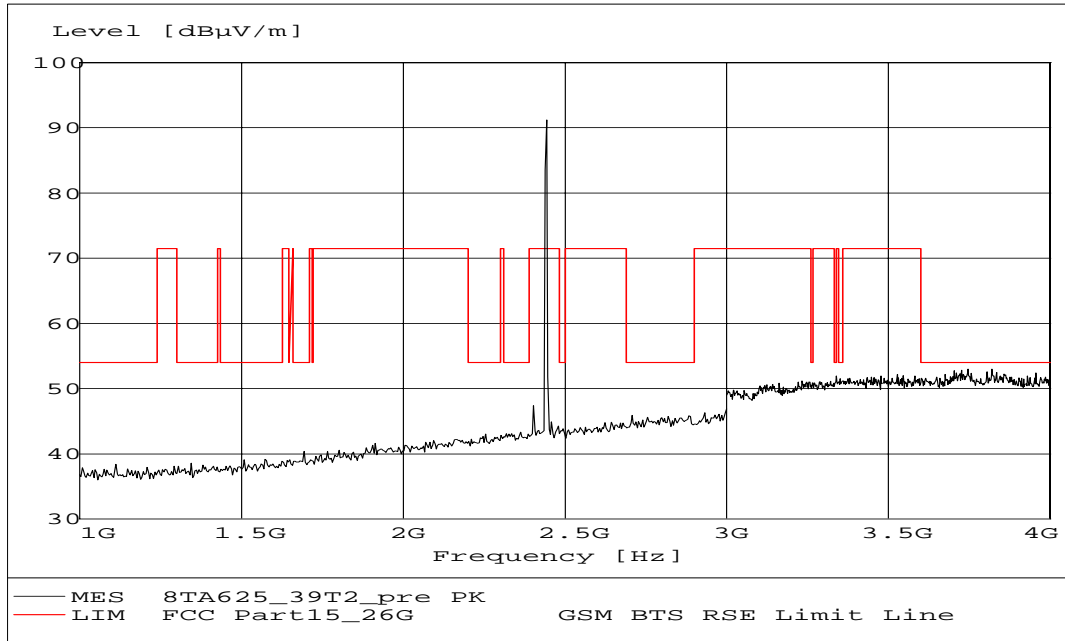
Fig. 19 Radiated emission: Channel 39, 1 GHz ~ 4 GHz
