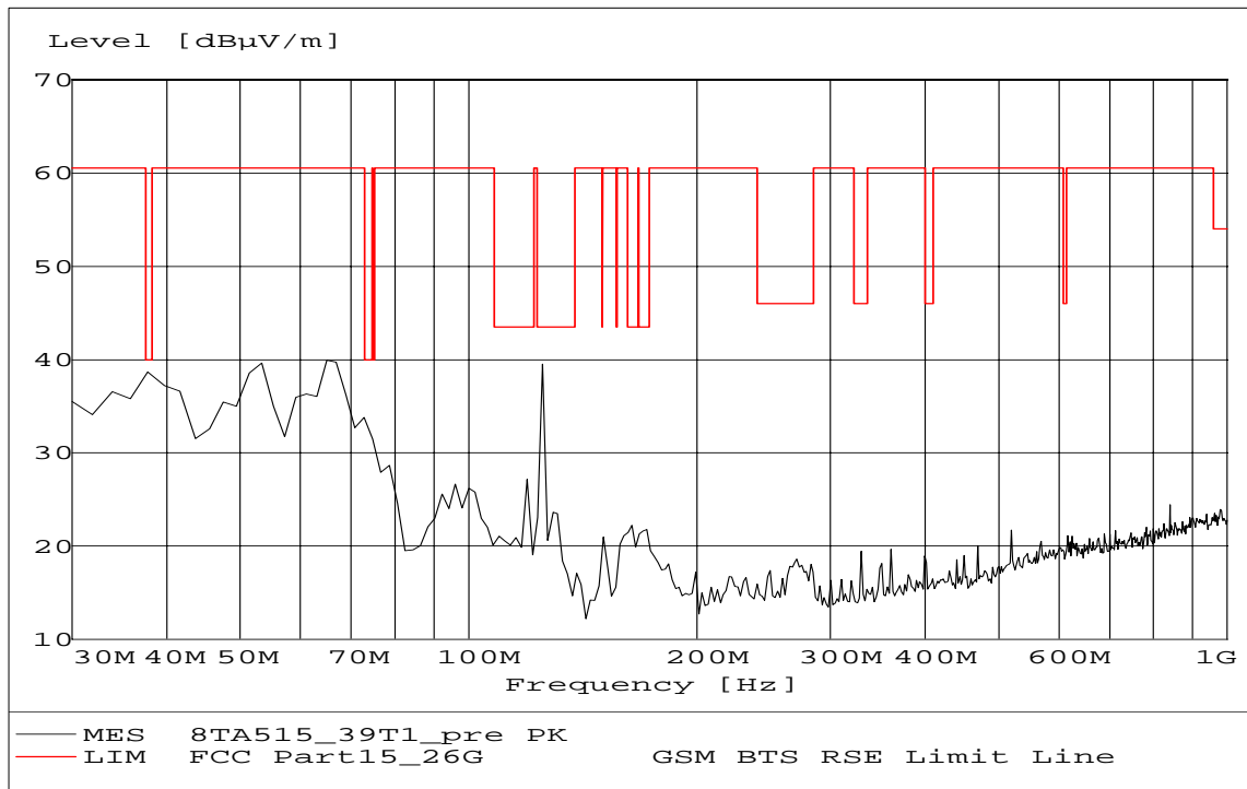
Fig. 17 Radiated emission: Channel 39, 30 MHz ~ 1 GHz
