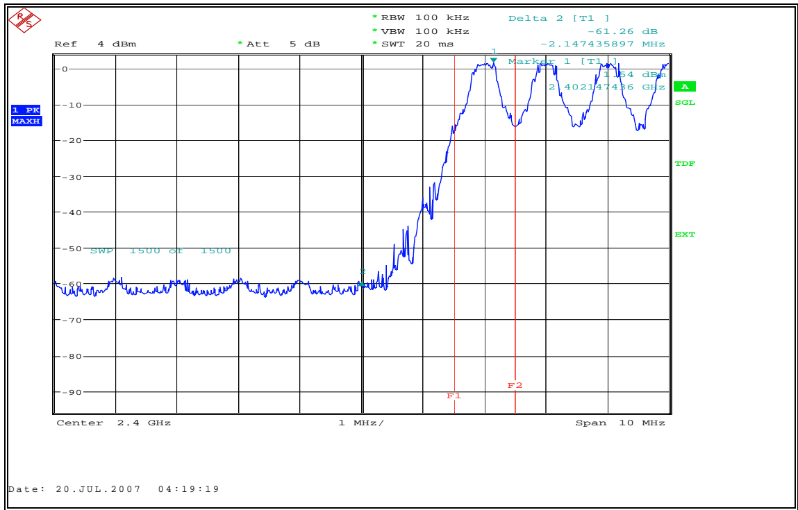
Fig. 2 Frequency Band Edges: Channel 0, Hopping On
