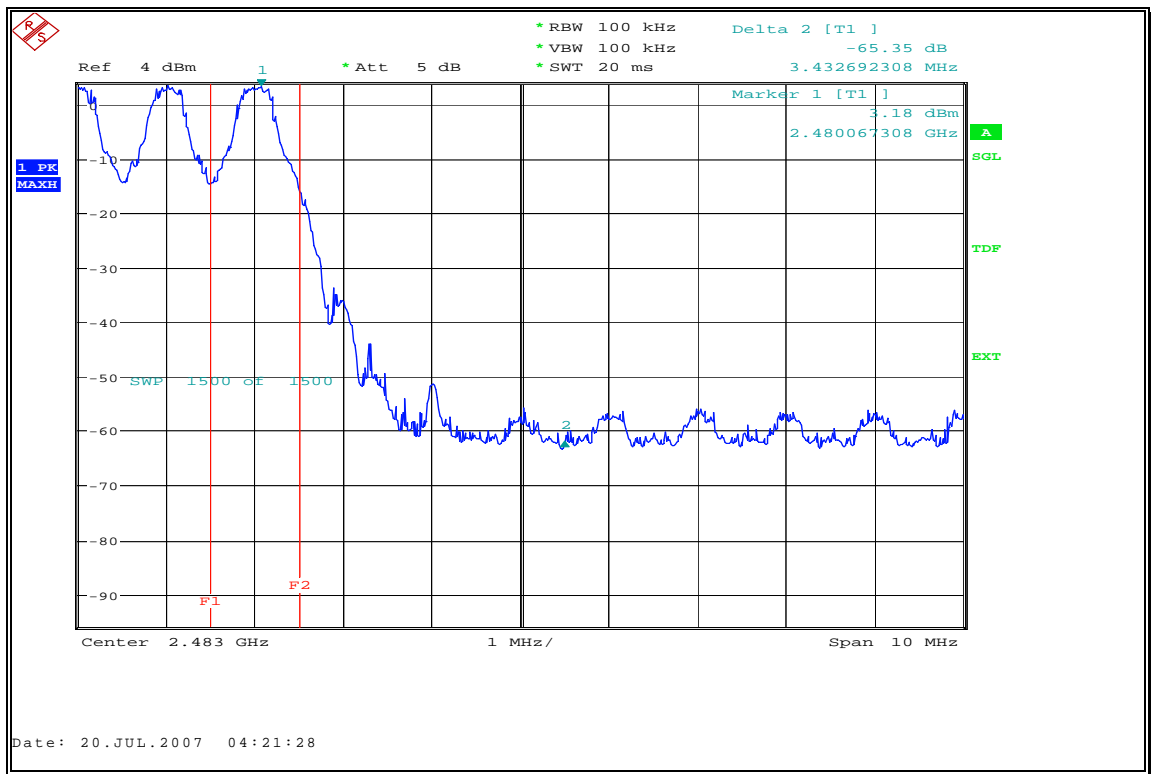
Fig. 4 Frequency Band Edges: Channel 78, Hopping On
