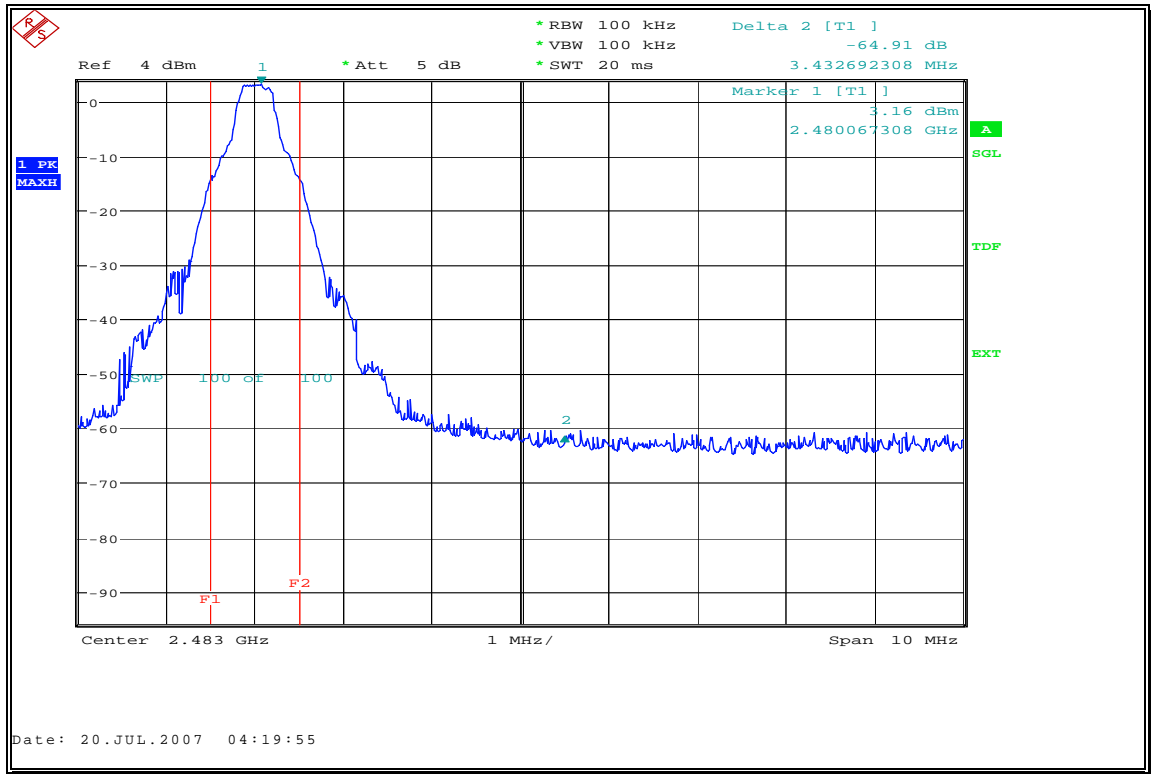
Fig. 3 Frequency Band Edges: Channel 78, Hopping Off
