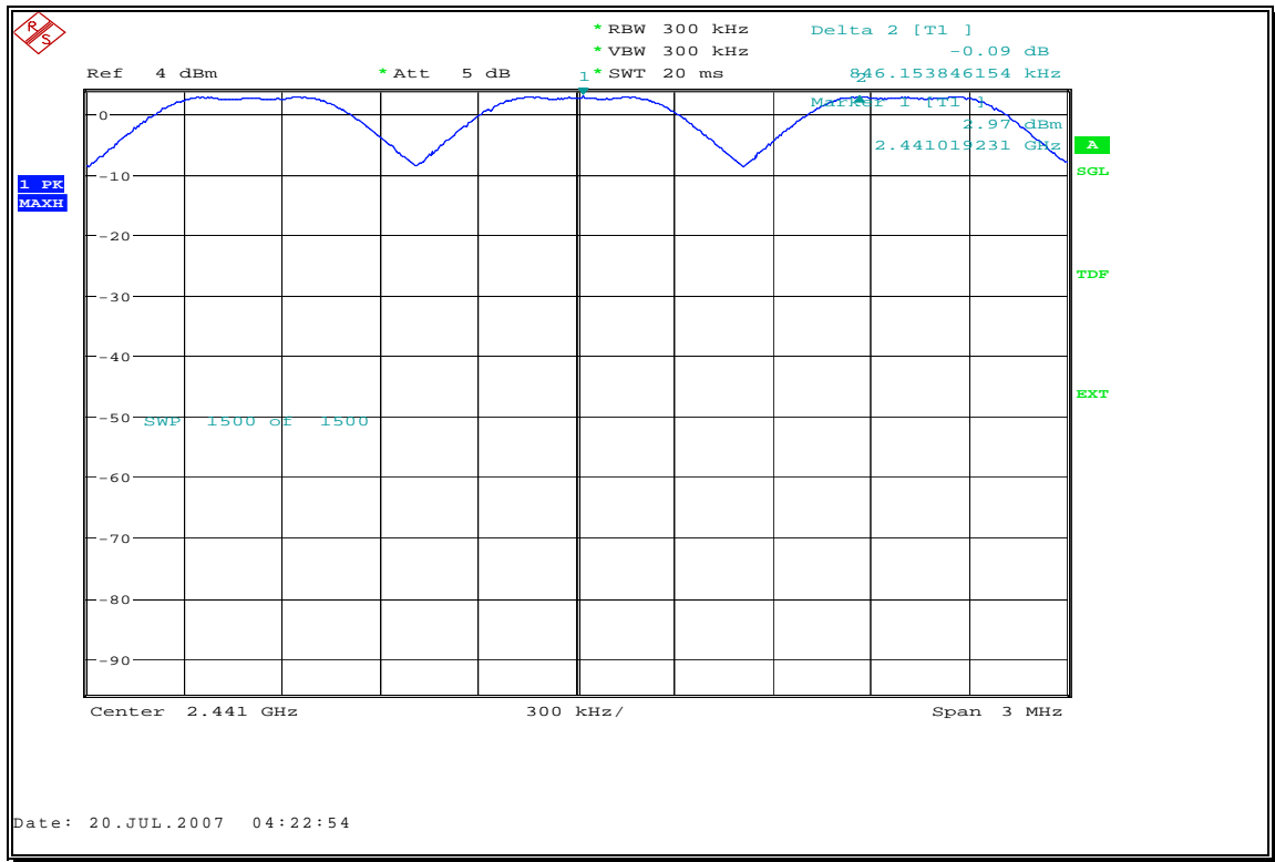
Fig. 29 Carrier frequency separation measurement: Channel 39
