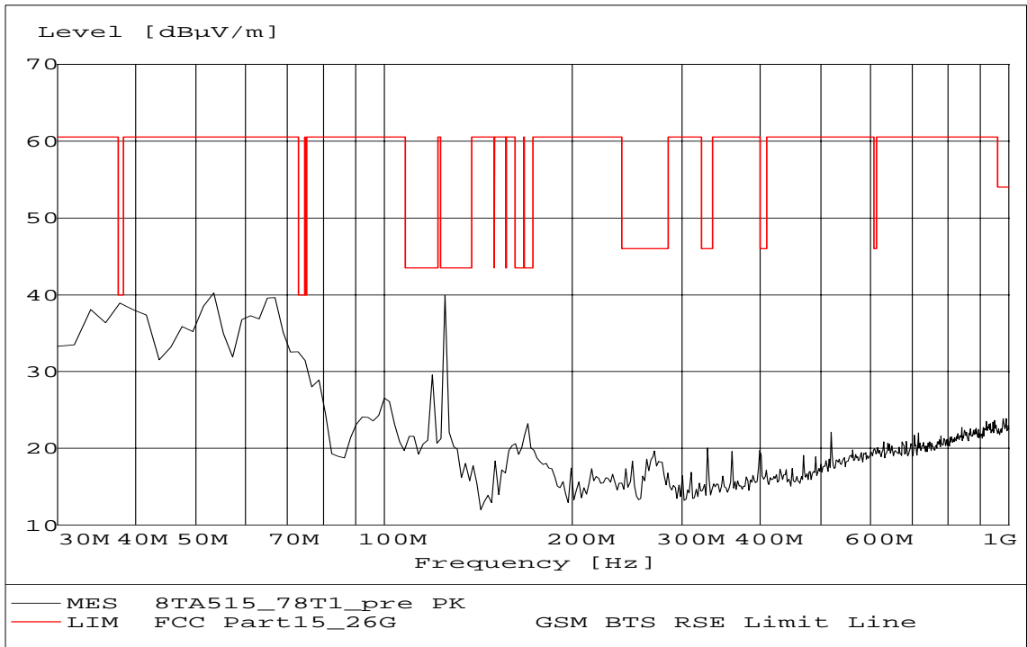
Fig. 20 Radiated emission: Channel 78, 30 MHz ~ 1 GHz
