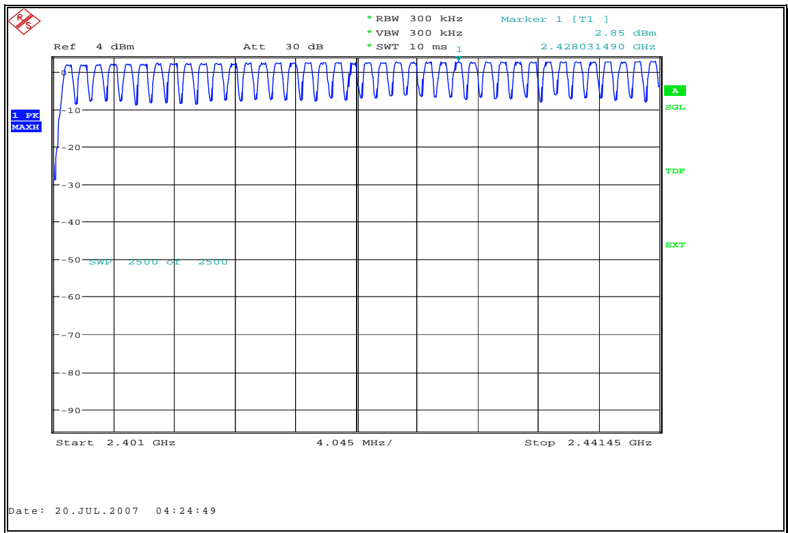
Fig. 30 Number of hopping frequencies: Channel 0 – 39
