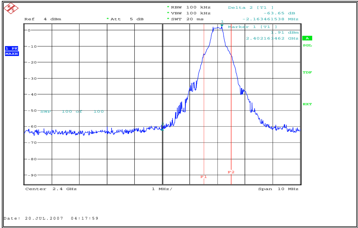
Fig. 1 Frequency Band Edges: Channel 0, Hopping Off
