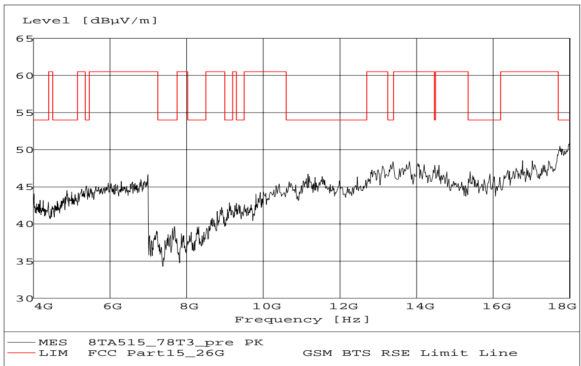
Fig. 22 Radiated emission: Channel 78, 4 GHz ~ 18 GHz
