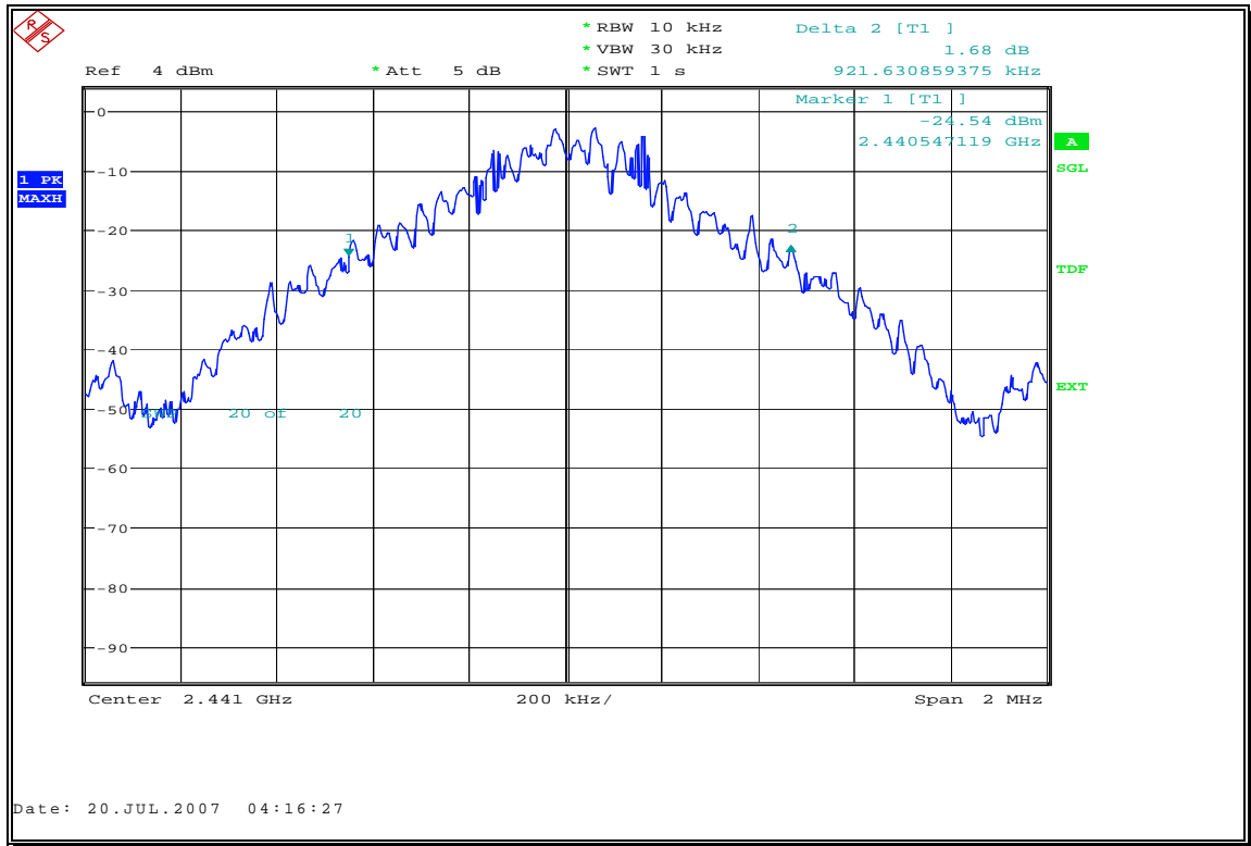
Fig. 27 20dB Bandwidth: Channel 39
