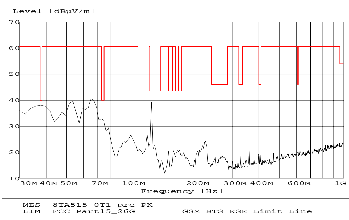
Fig. 14 Radiated emission: Channel 0, 30 MHz ~ 1 GHz
