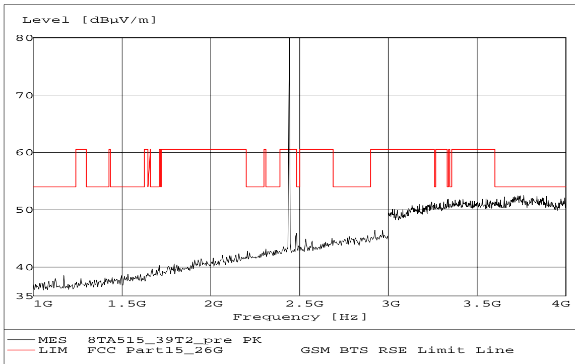
Fig. 18 Radiated emission: Channel 39, 1 GHz ~ 4 GHz
