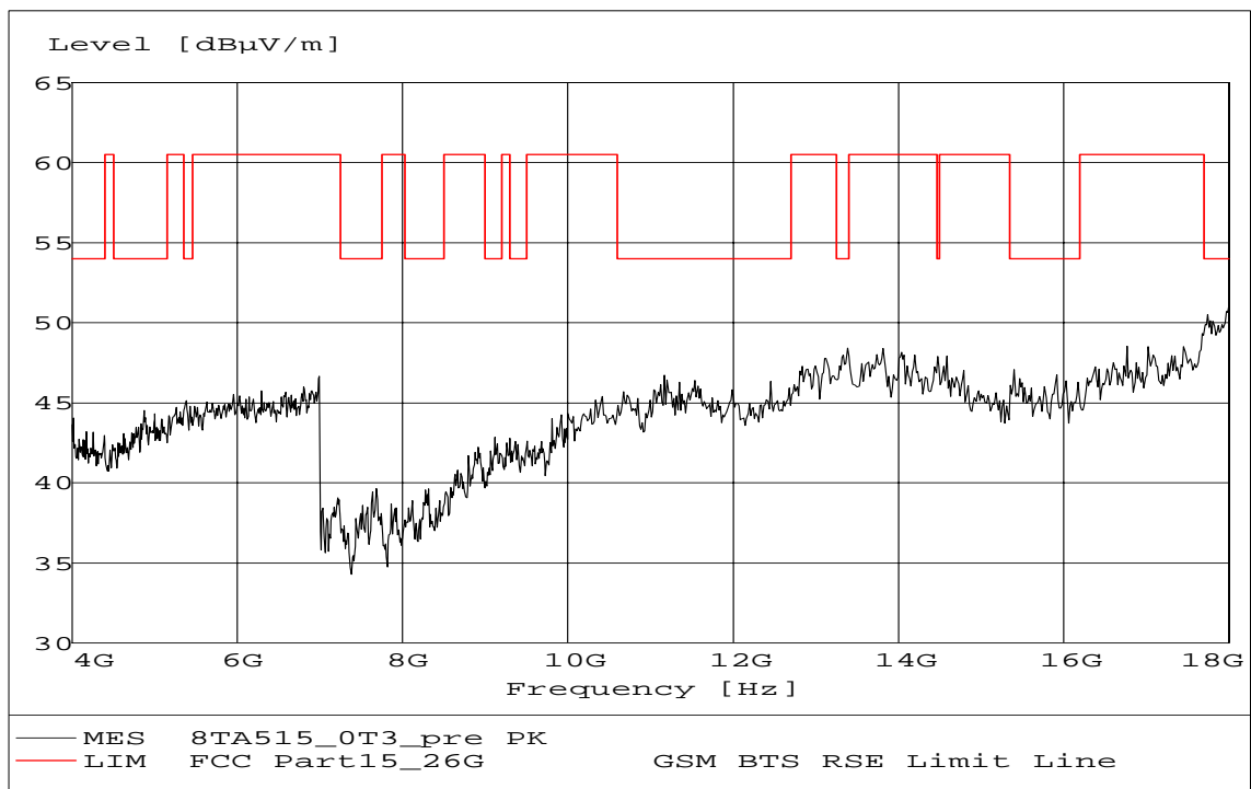
Fig. 16 Radiated emission: Channel 0, 4 GHz ~ 18 GHz
