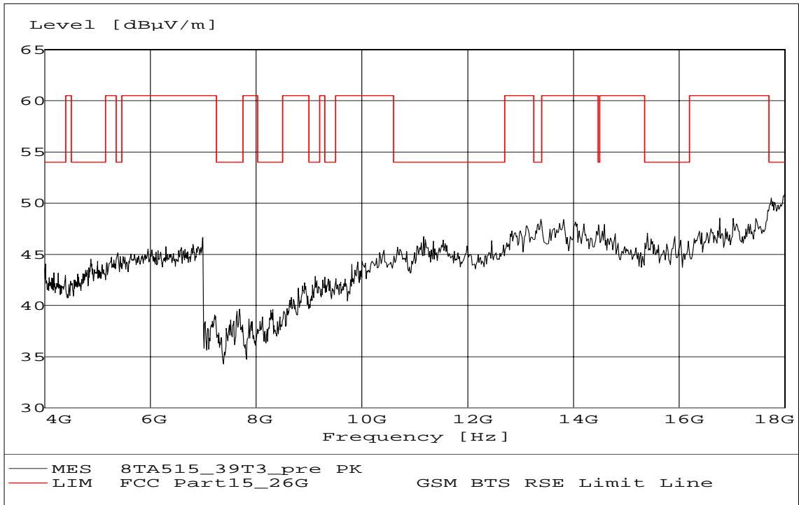
Fig. 19 Radiated emission: Channel 39, 4 GHz ~ 18 GHz
