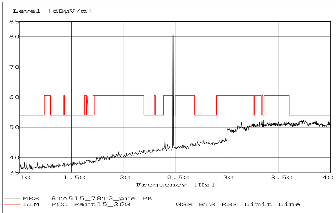
Fig. 21 Radiated emission: Channel 78, 1 GHz ~ 4 GHz
