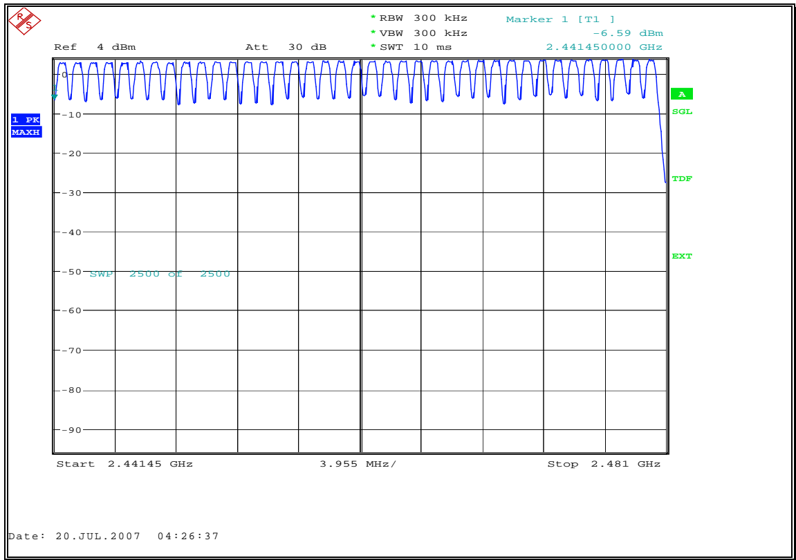
Fig. 31 Number of hopping frequencies: Channel 40 - 78
