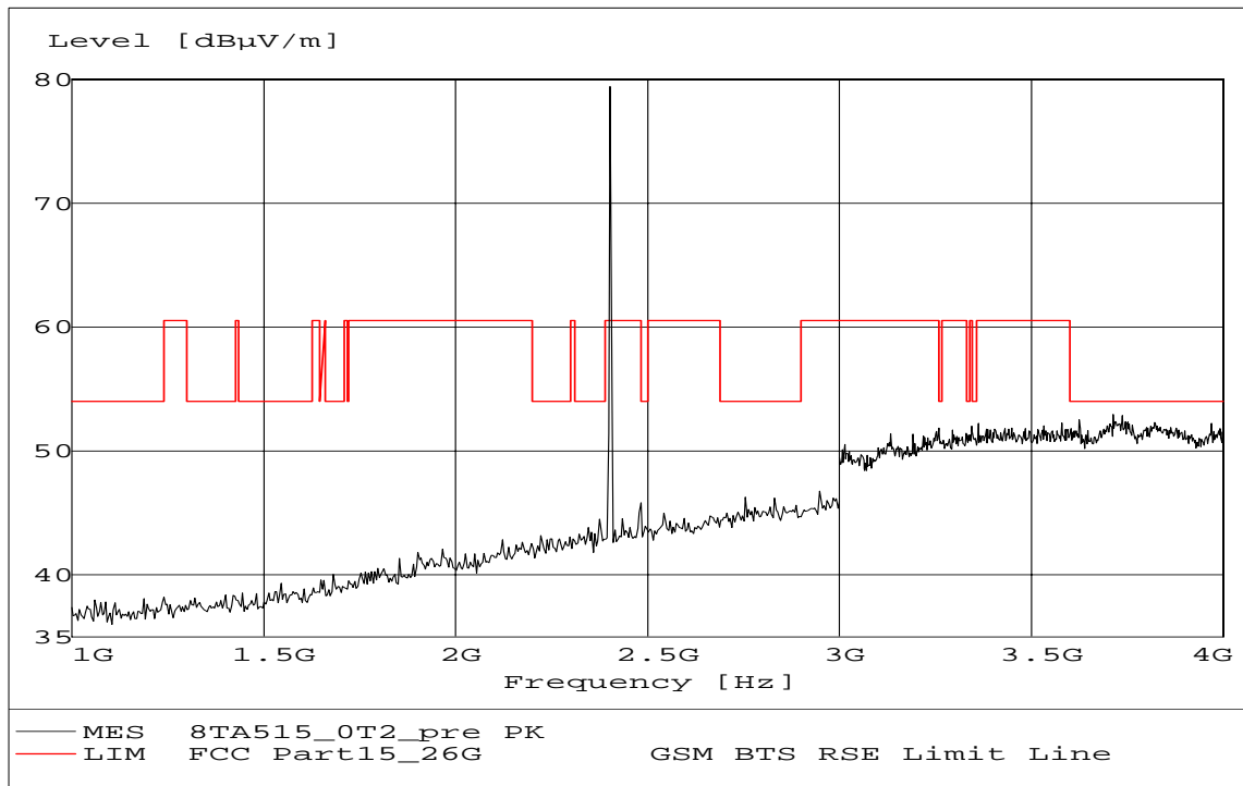
Fig. 15 Radiated emission: Channel 0, 1 GHz ~ 4 GHz
