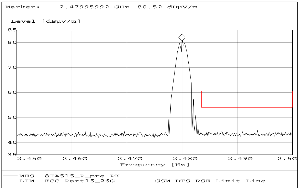
Fig. 23 Radiated emission (Power): 2.45GHz ~ 2.5GHz
