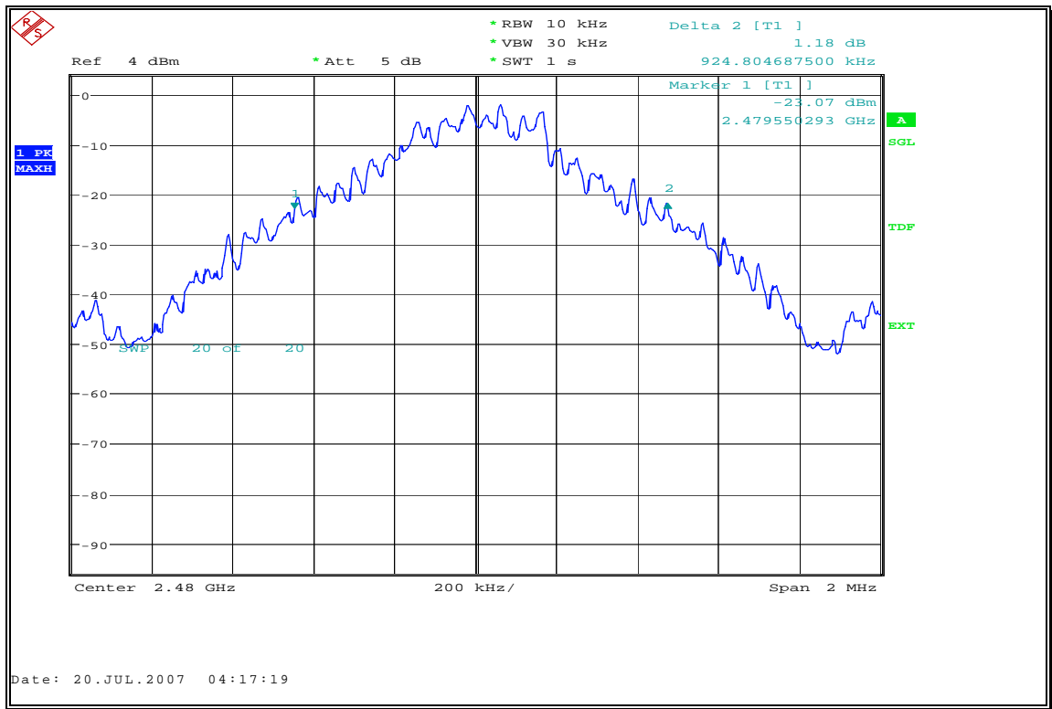
Fig. 28 20dB Bandwidth: Channel 78
