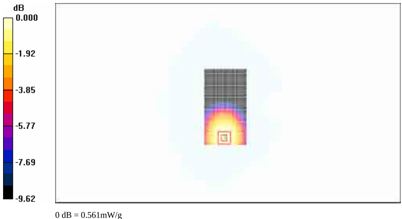
Fig. 73 850 MHz CH251 with Bluetooth function
