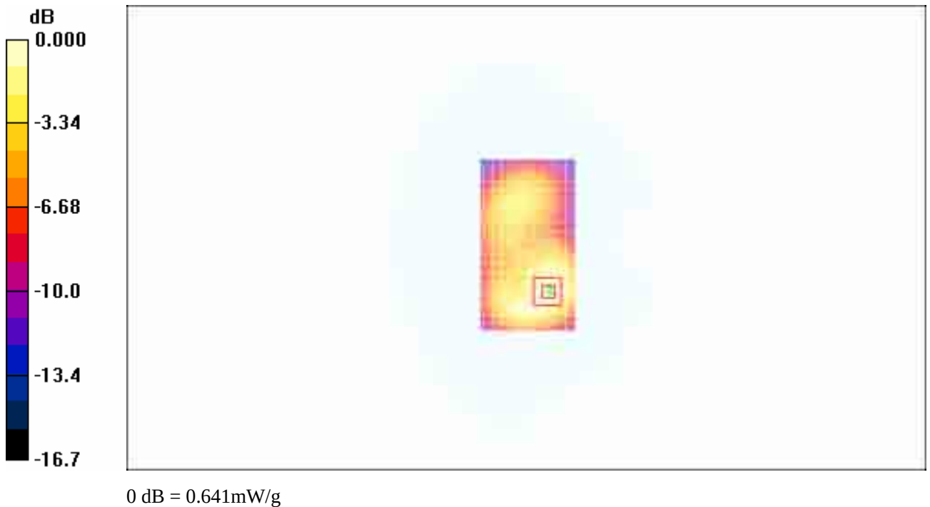
Fig. 69 1900 MHz CH661
