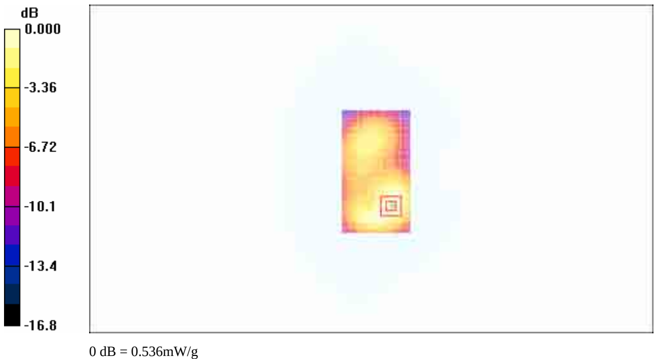
Fig. 71 1900 MHz CH512
