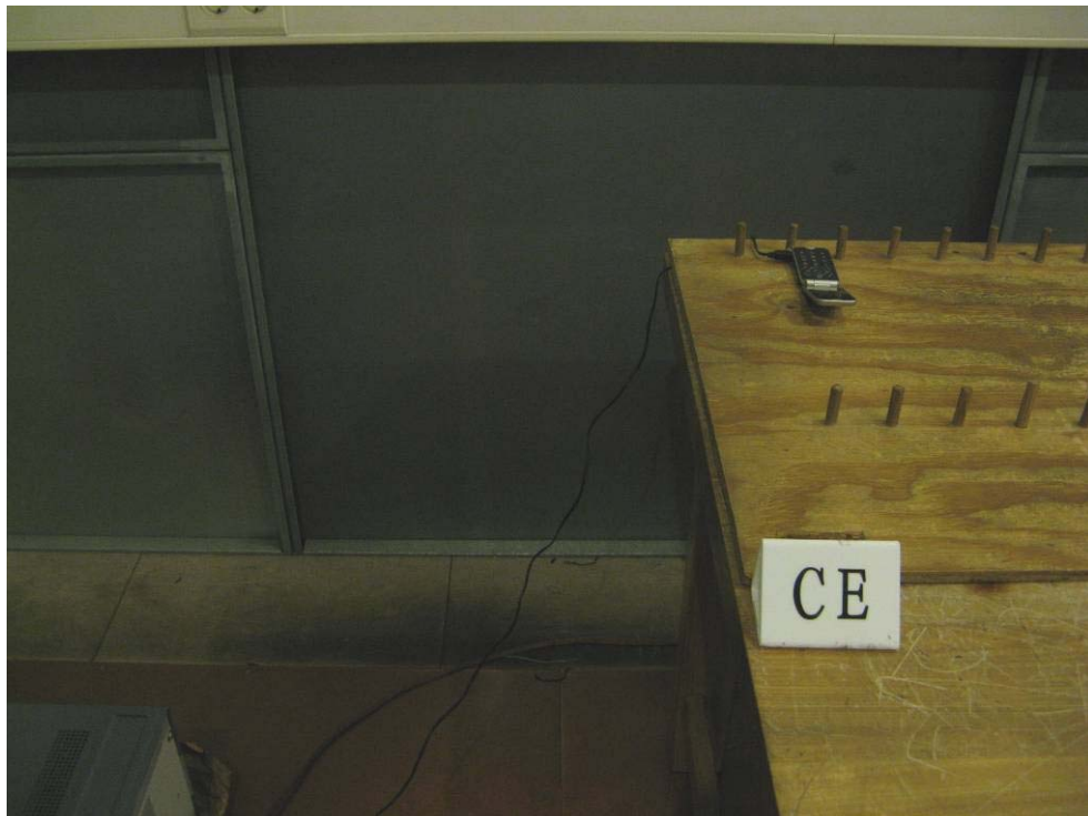
Pic 4 Part 15B Conducted Emission with charger
