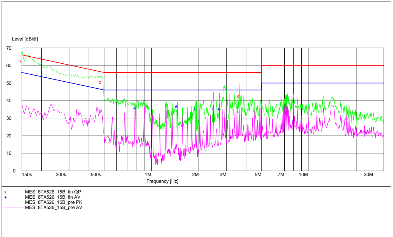
Figure B.3 Conducted Emission
