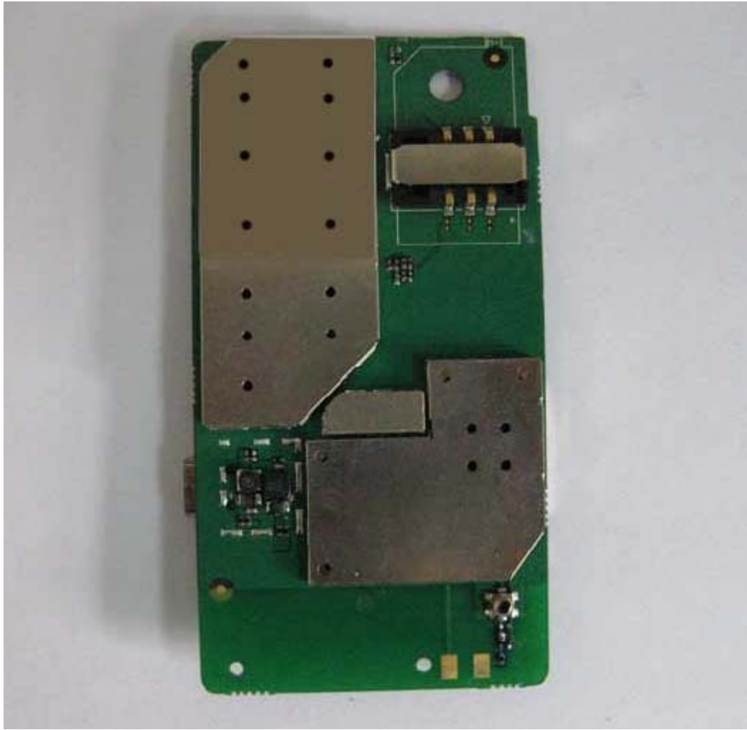
Picture 4: the back view of the sample with the RF shield-2
