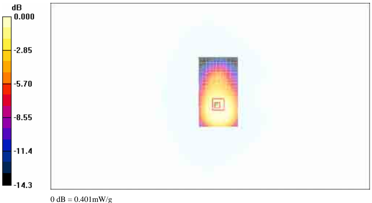
Fig. 71 1900 MHz CH512
