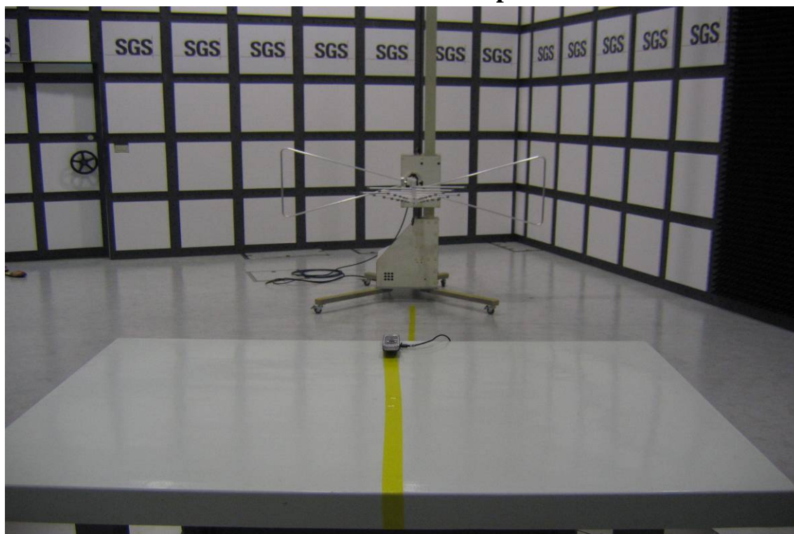
Radiated Emission Set up Photo
