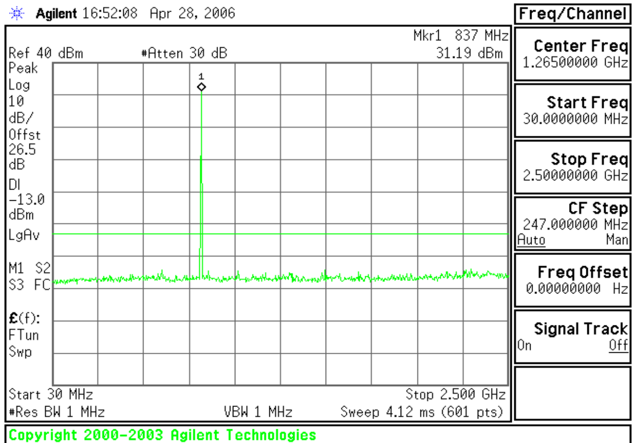
Figure 7-3: Out of Band emission at antenna terminals – GSM CH Mid
